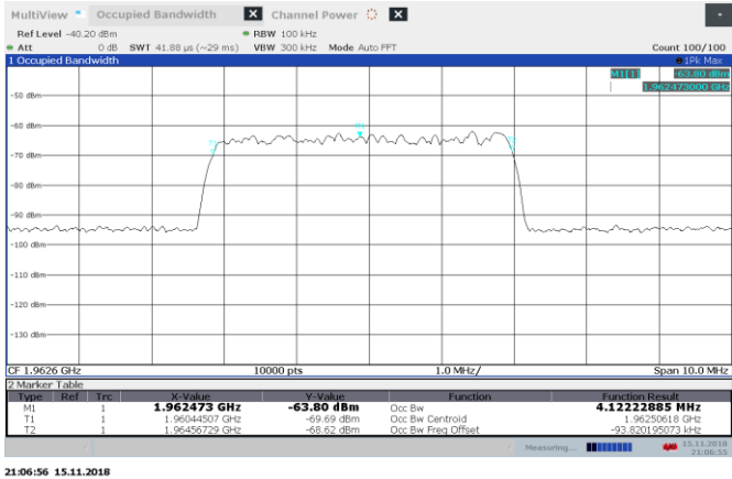
Figure 8.3-3: AWGN AGC+3 dB 1962.5 MHz input 99% BW DL
