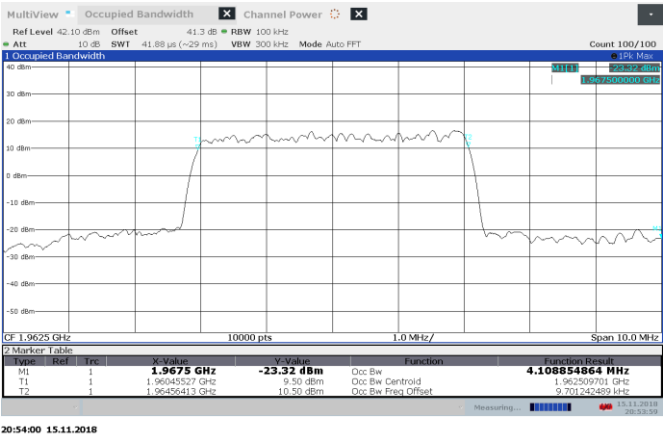
Figure 8.3-2: AWGN AGC-0.5 dB 1962.5 MHz output 99% BW DL
