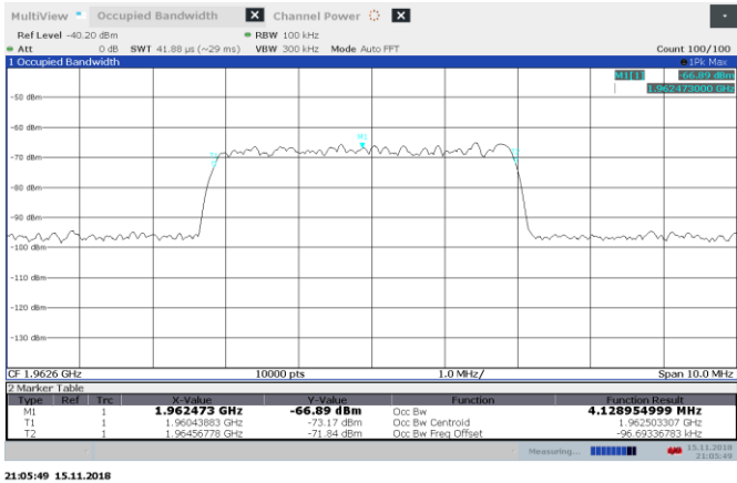
Figure 8.3-1: AWGN AGC-0.5 dB 1962.5 MHz input 99% BW DL
