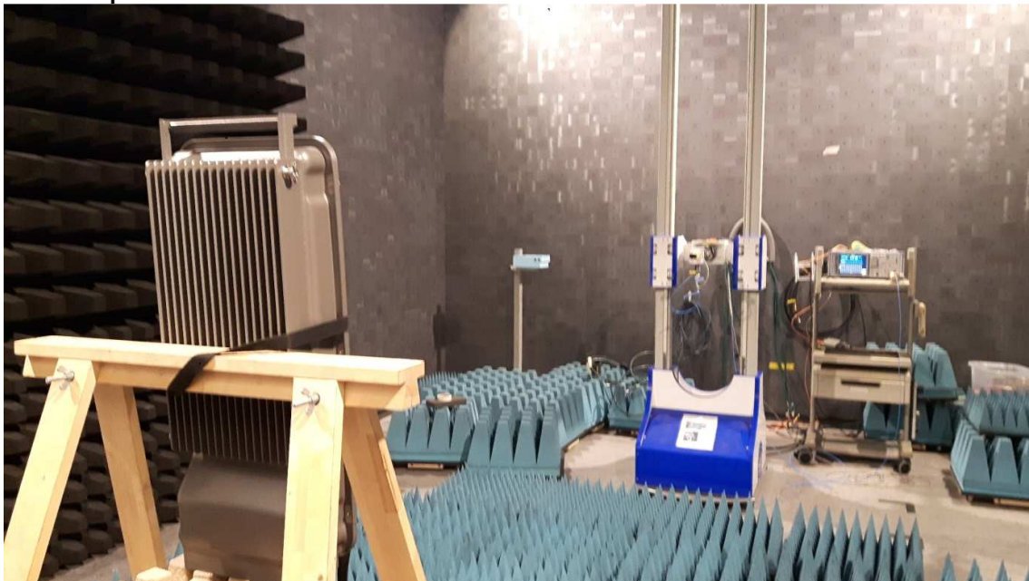
Test set up radiated emission 18 GHz – 26 GHz
