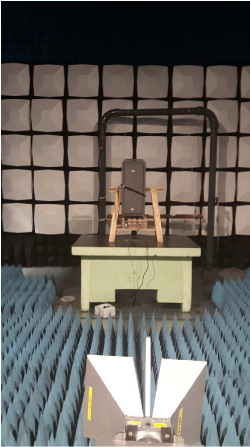
Test set up radiated emission 1GHz – 18 GHz
