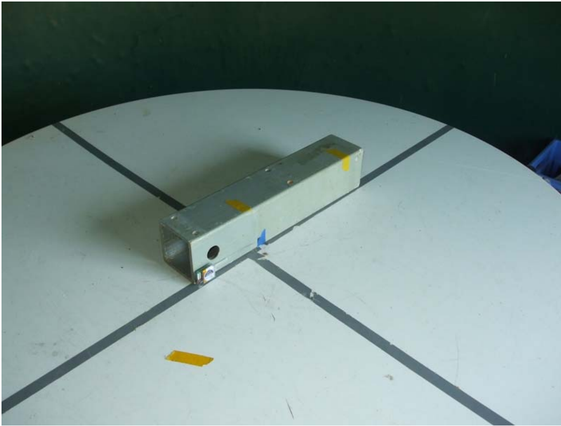
Z Plane
