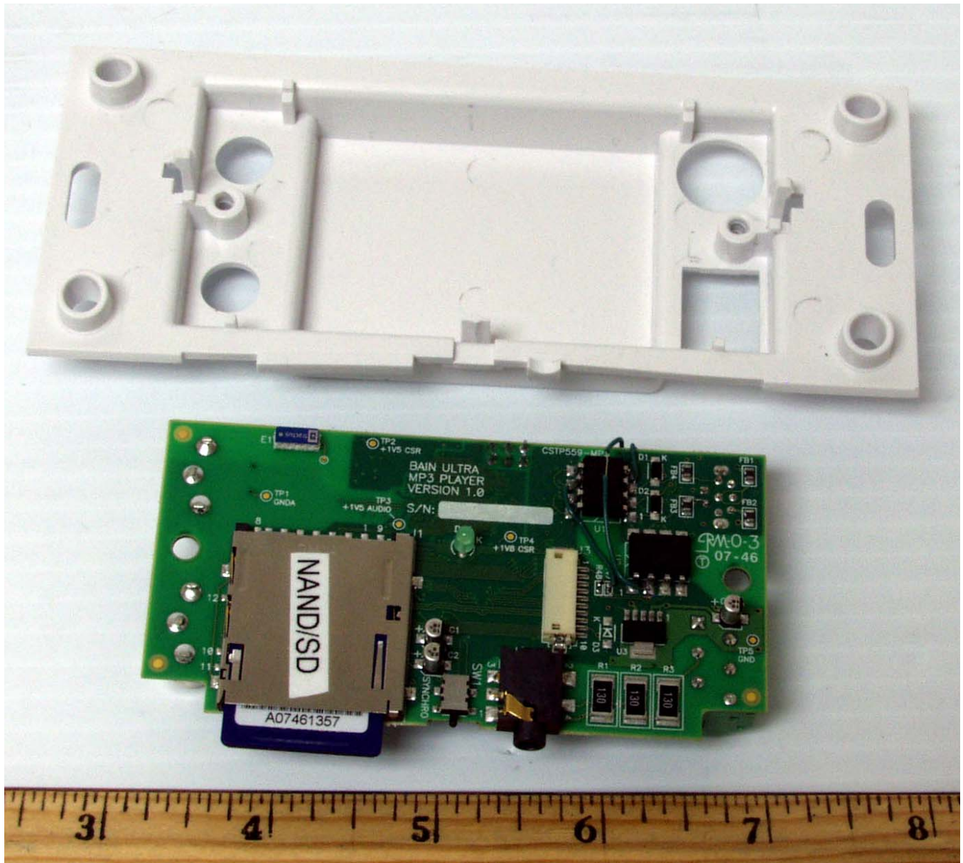
PCB removed from back cover
