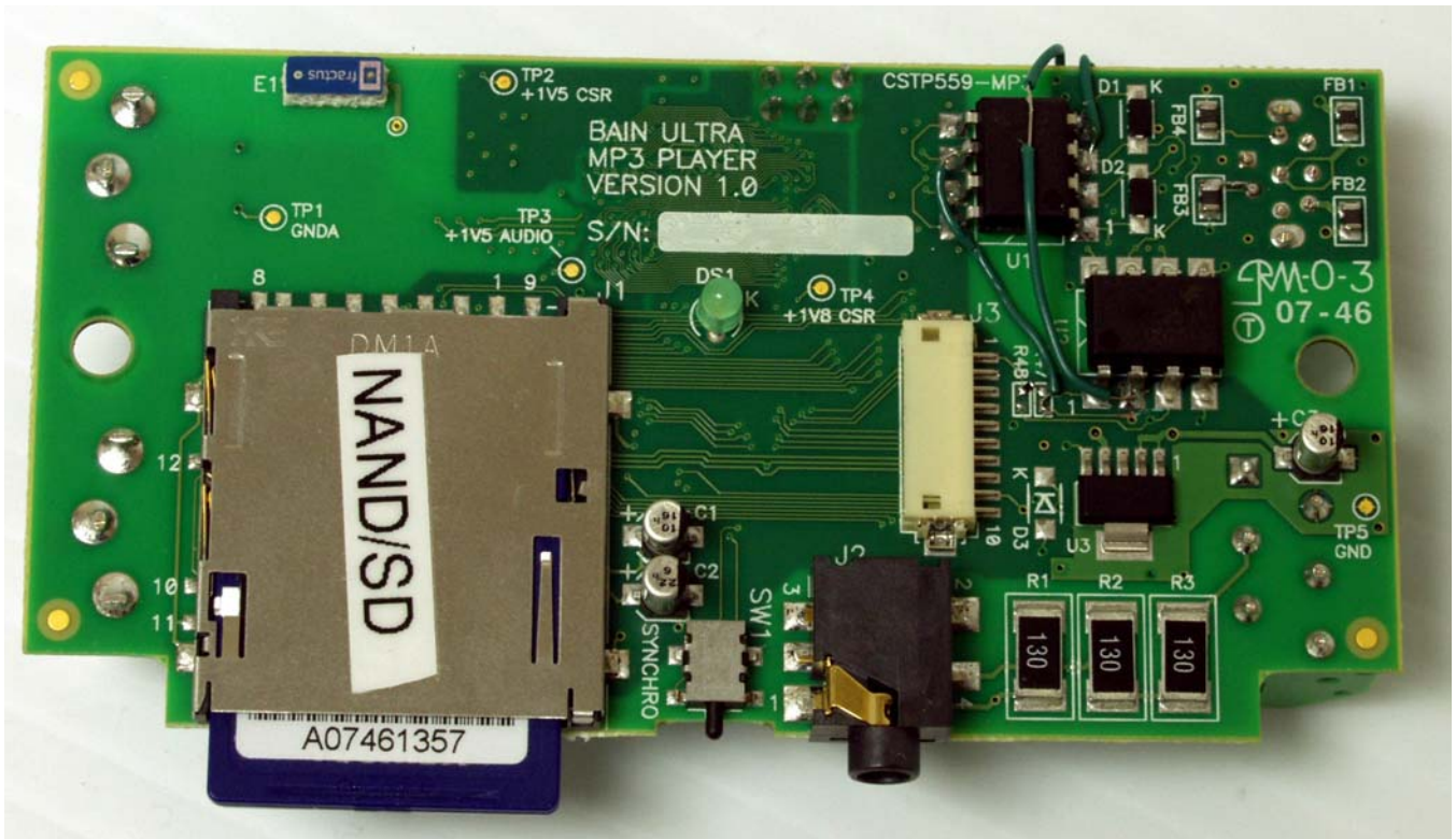
PCB top side view
