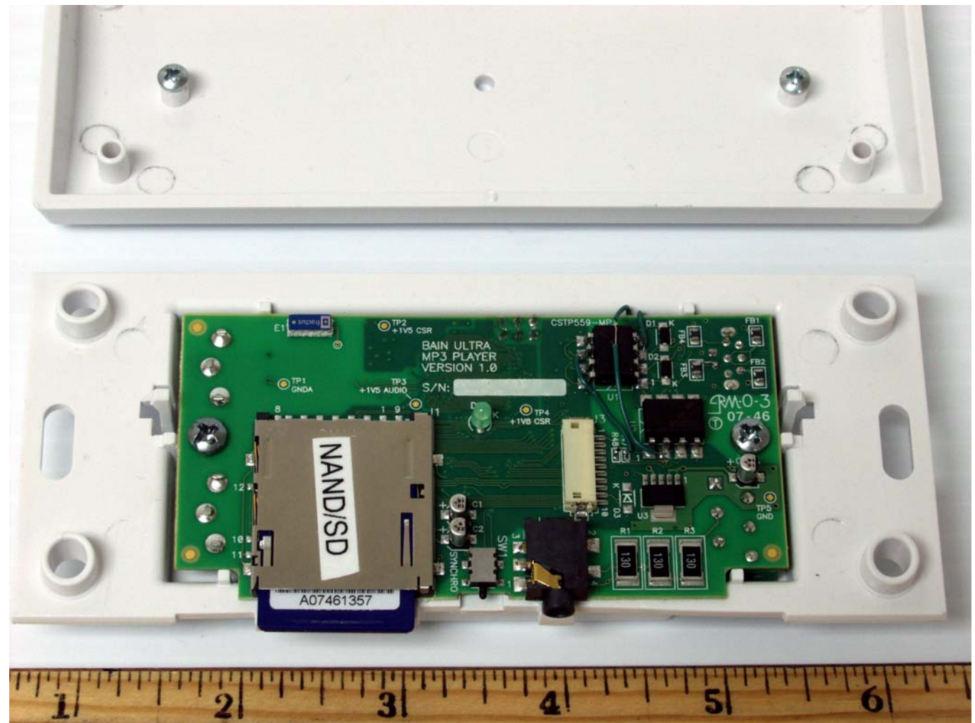
Internal view with removed front cover
