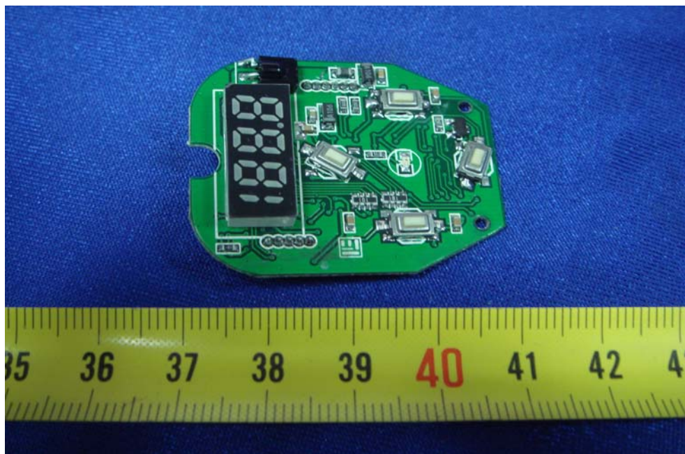
PCB1-Back View
