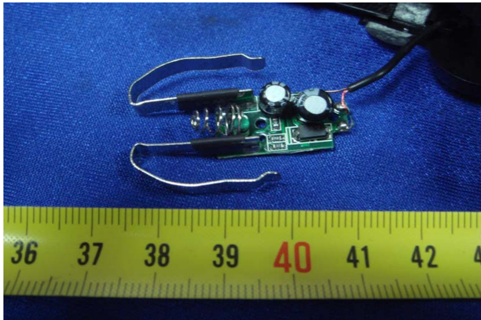
PCB3-Front View
