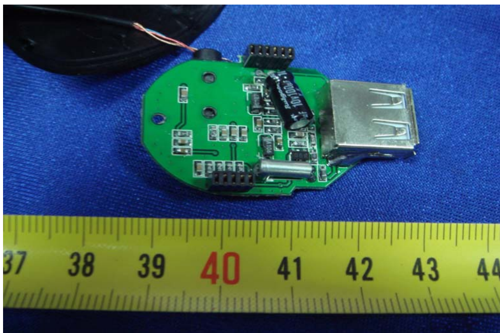
PCB2-Back View
