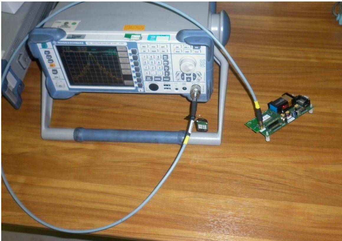
Transmitter conducted measurements
