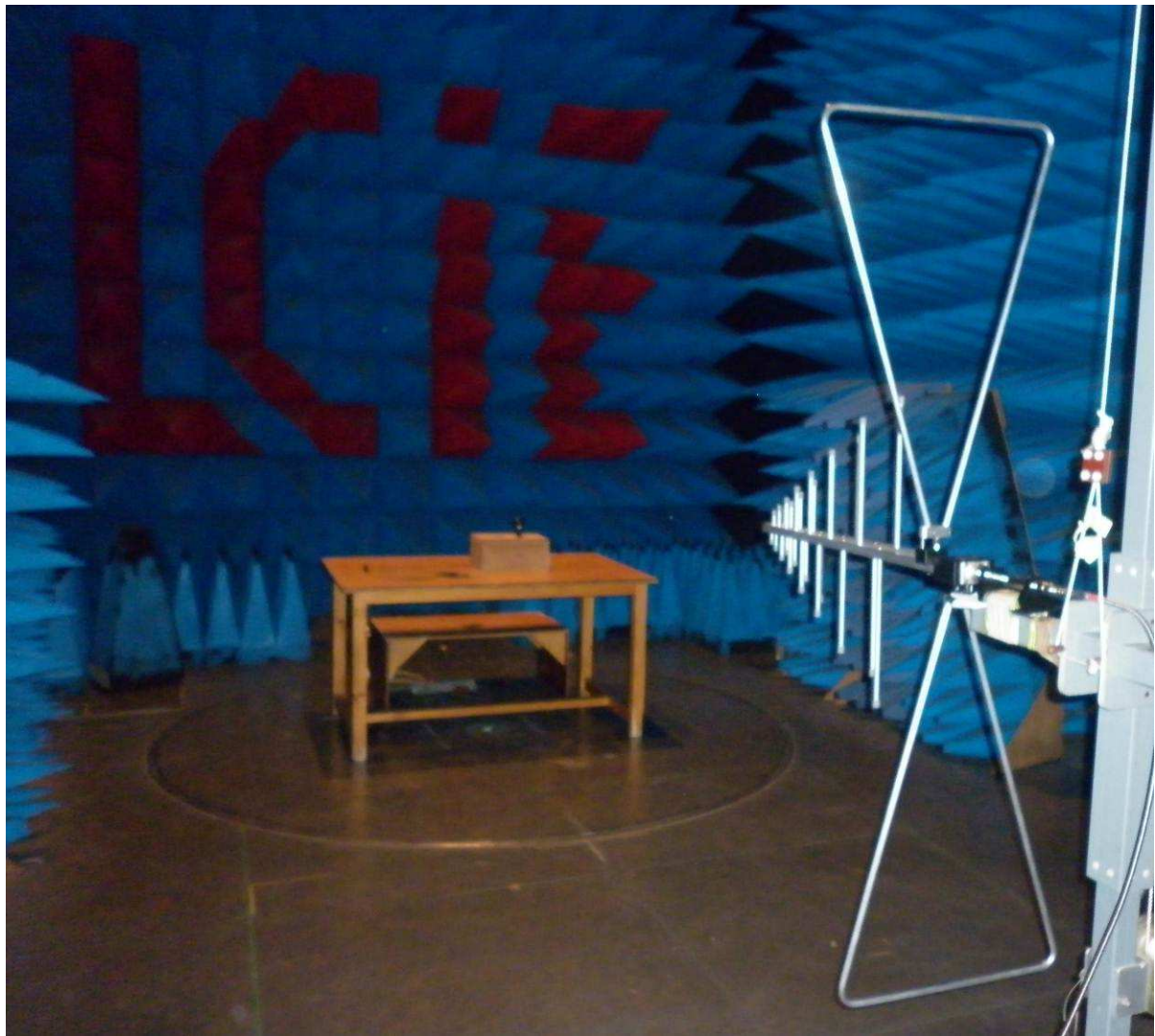
Radiated emissions measurements
