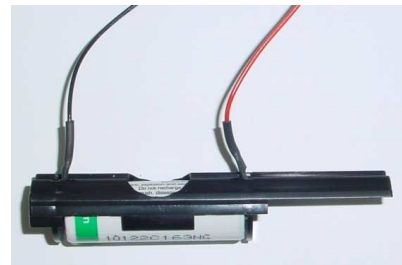
Diver-DXT with radio board, cap (with o-ring) and lithium battery
