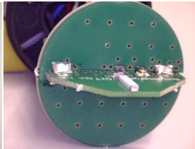
Diver-DXT antenna area (two sides)
