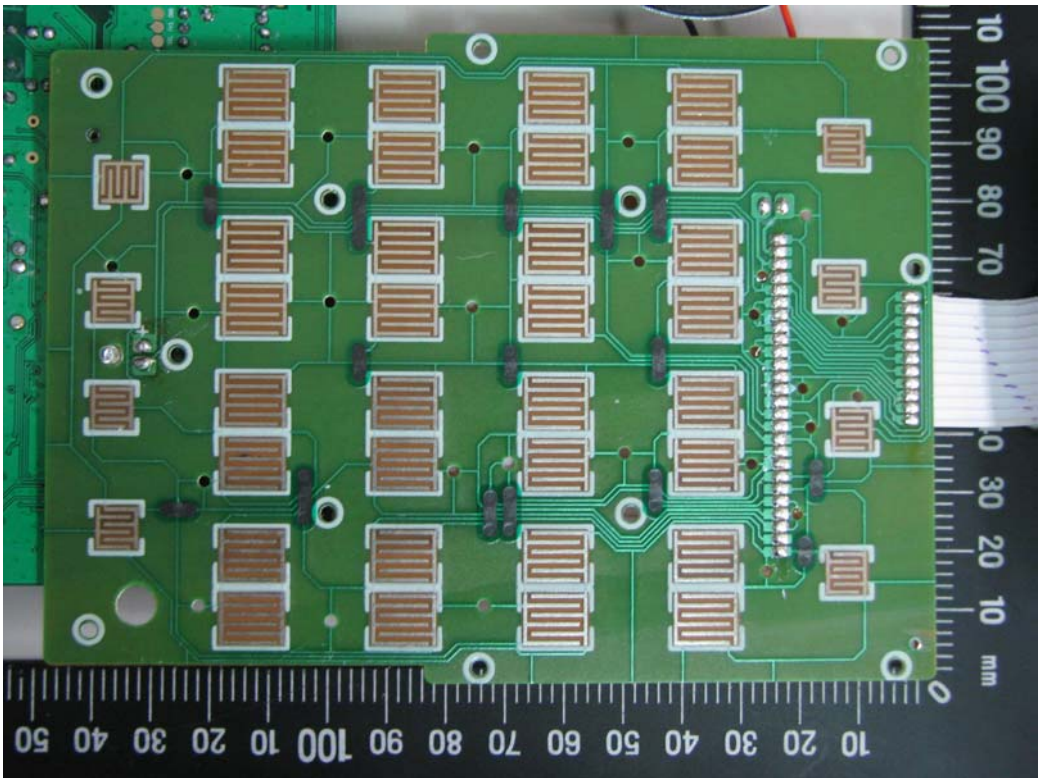
10. Front view of PCB3
