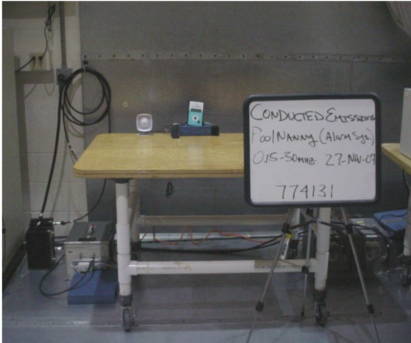
Test Set Up Conducted Emissions
