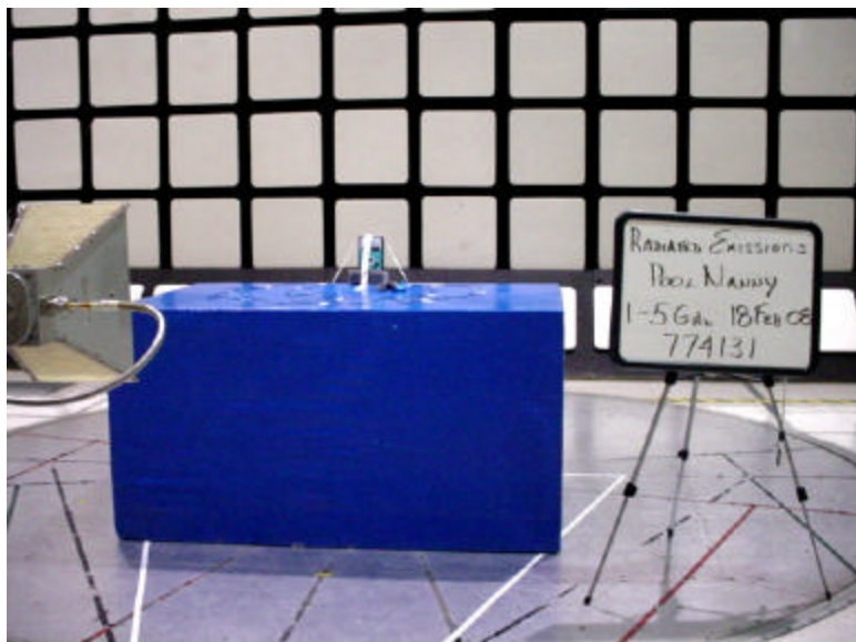
Test Set Up Radiated Emissions 1GHz to 5GHz
