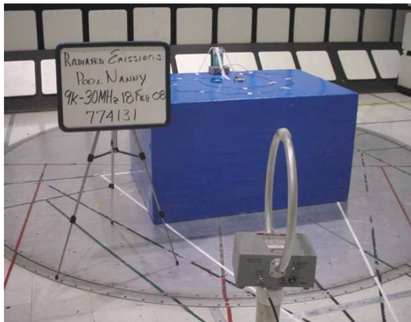
Test Set Up Radiated Emissions 9KHz to 30MHz
