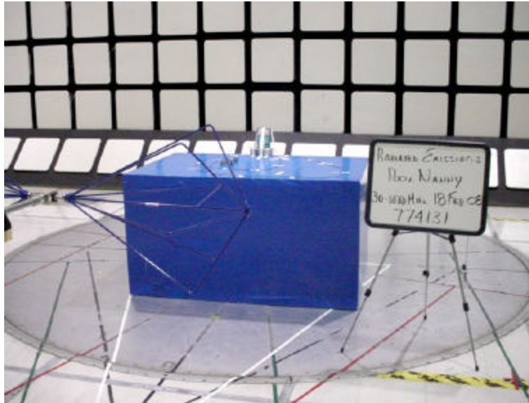
Test Set Up Radiated Emissions 30MHz to 1000MHz
