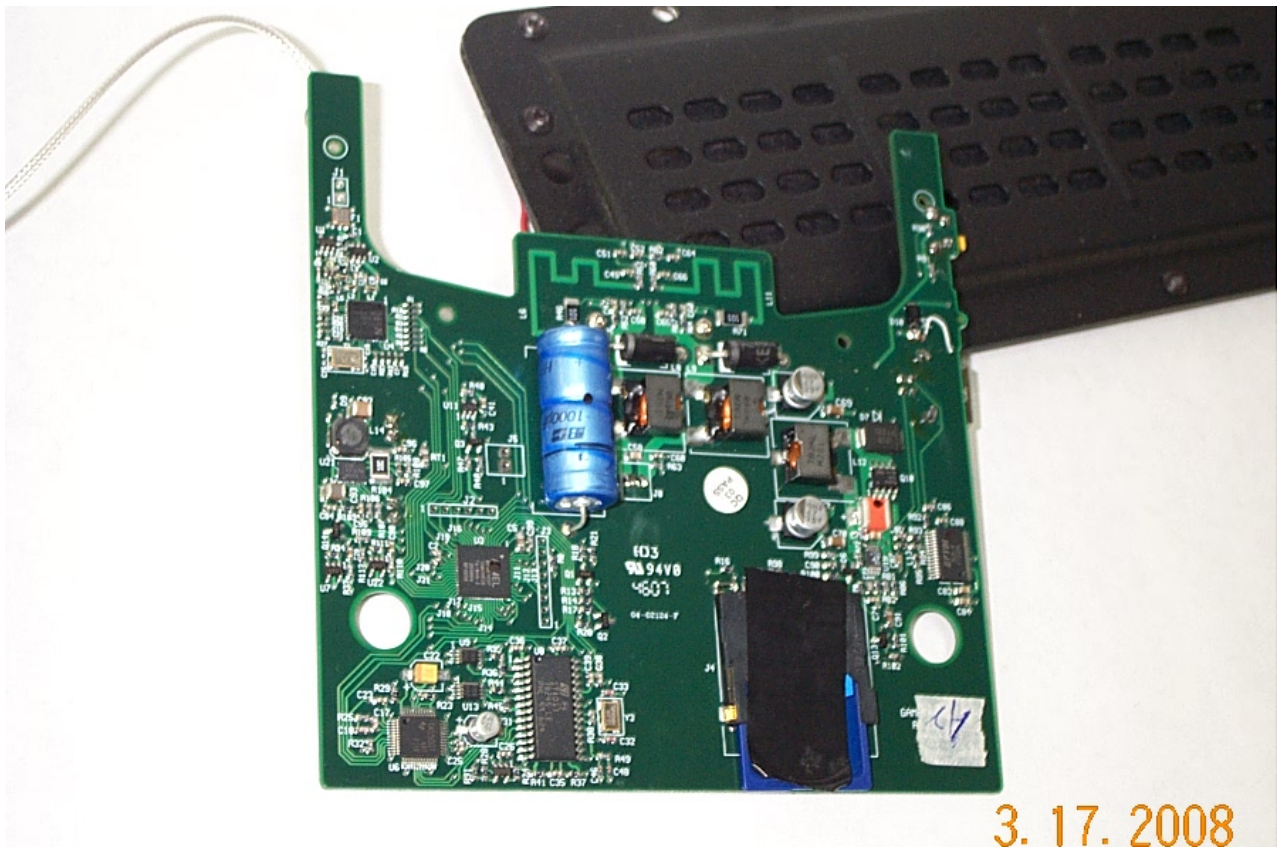
Photograph of Speaker Board: Flash card exposed
