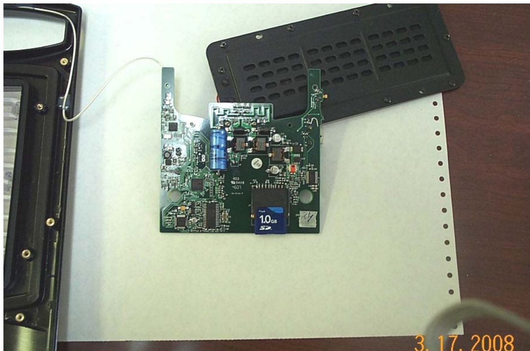
Photograph of Speaker Board: Flash card exposed
