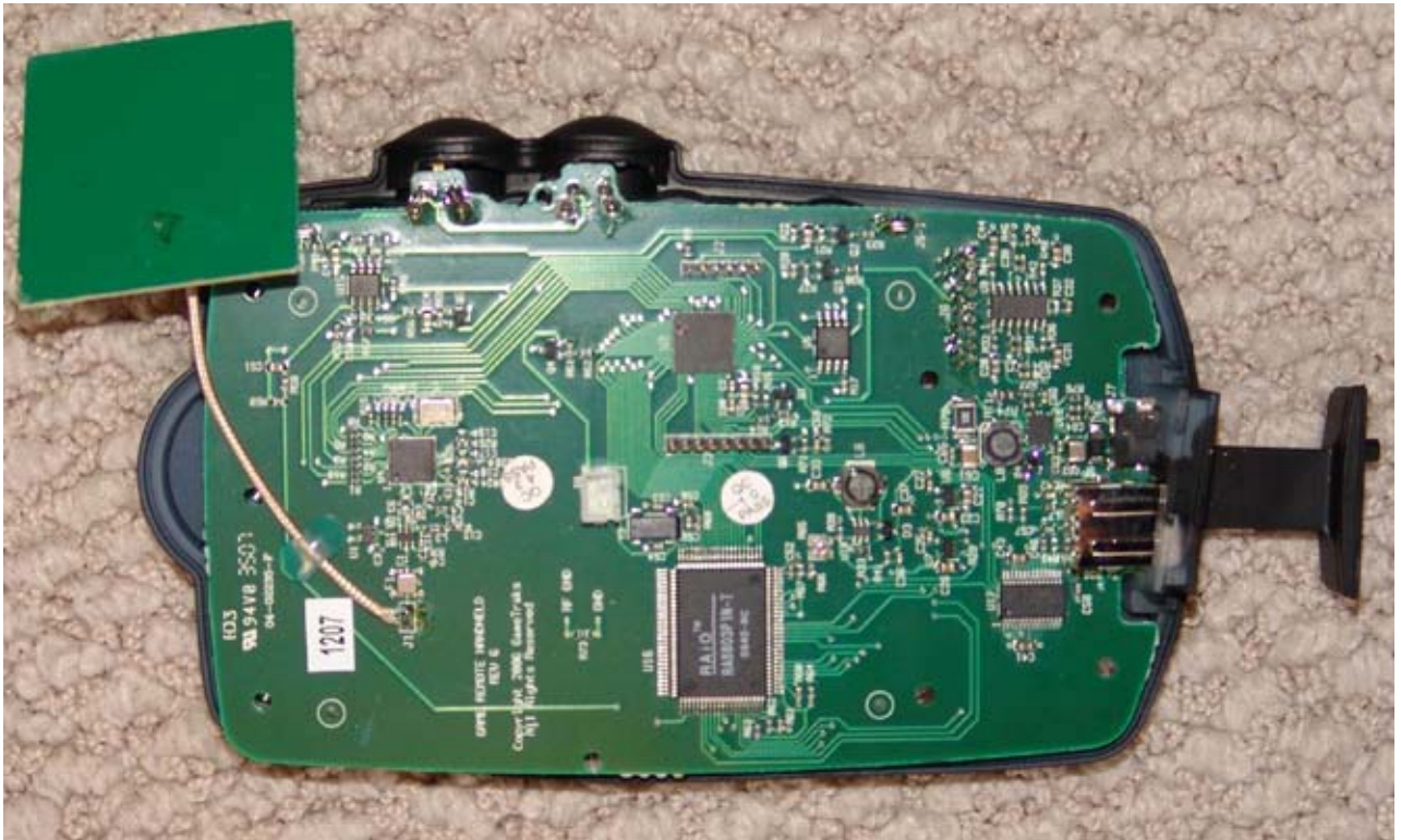
Photograph of Hand Held:
