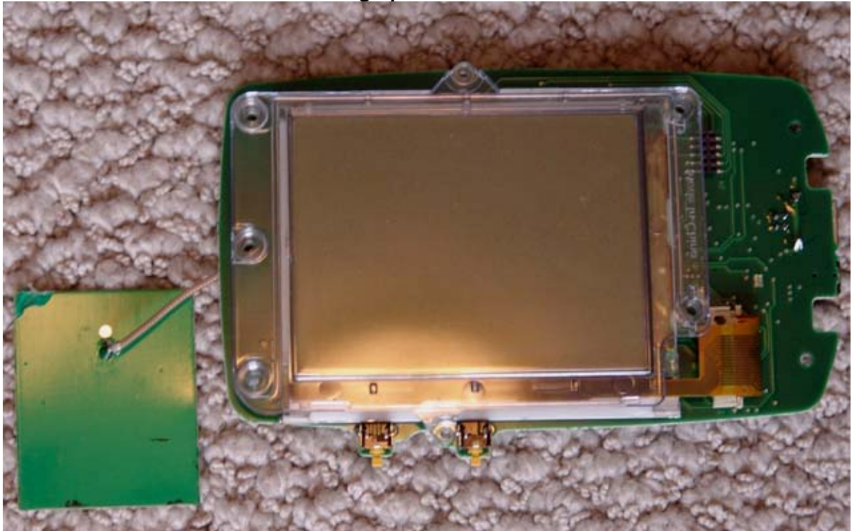
Photograph of Hand Held:
