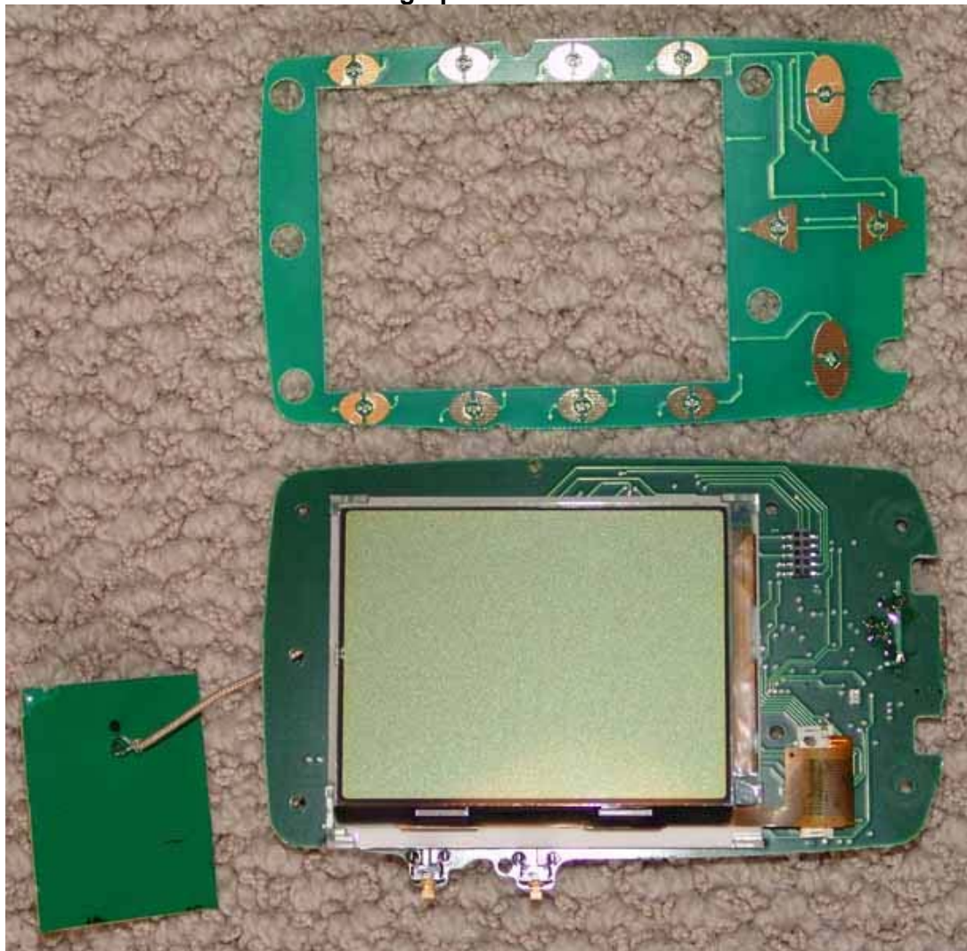
Photograph of Hand Held:
