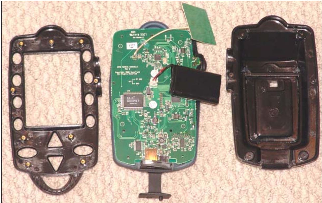
Photograph of Hand Held: Inside of battery compartment
