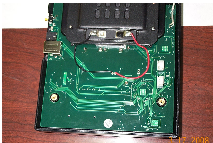
Photograph of Speaker Board: Foil Side
