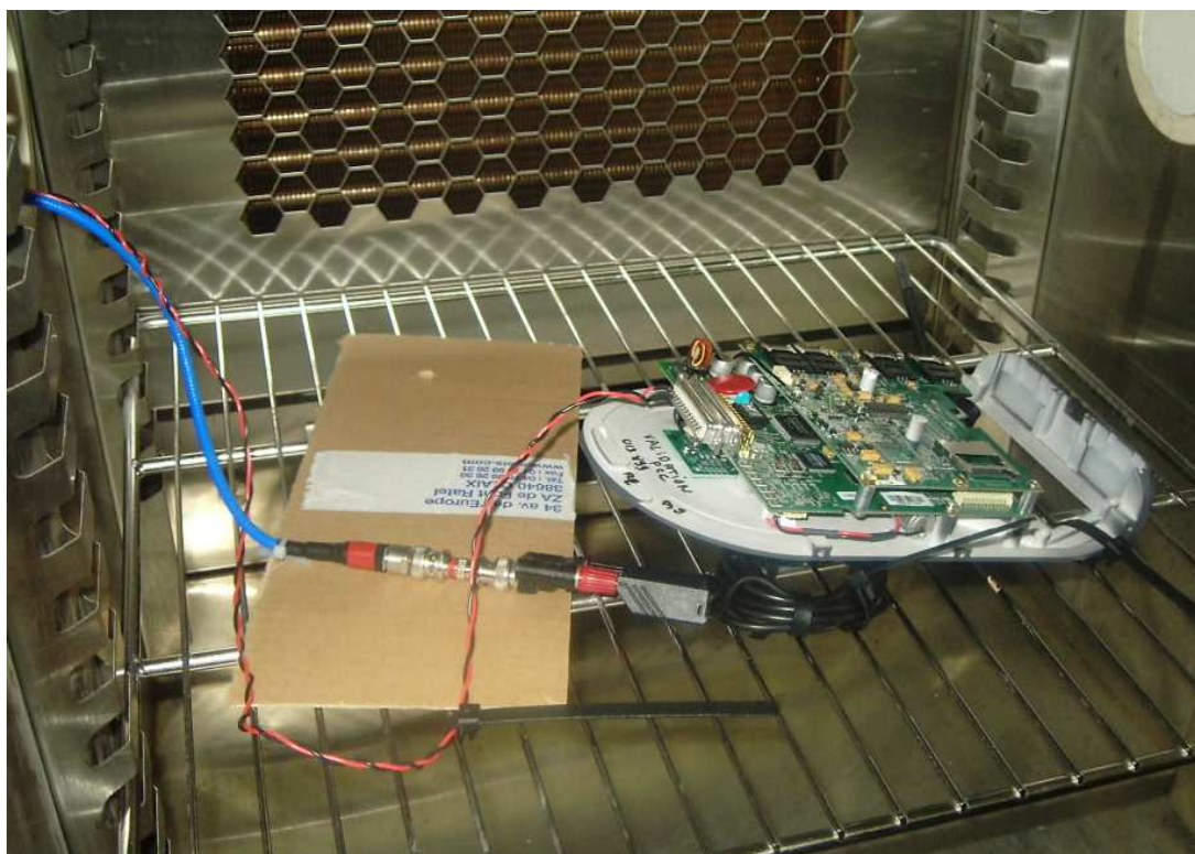
Frequency stability set up
