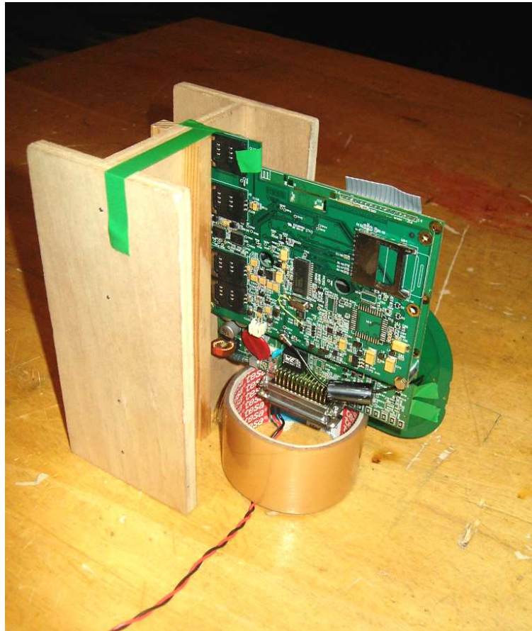
Frequency stability set up
