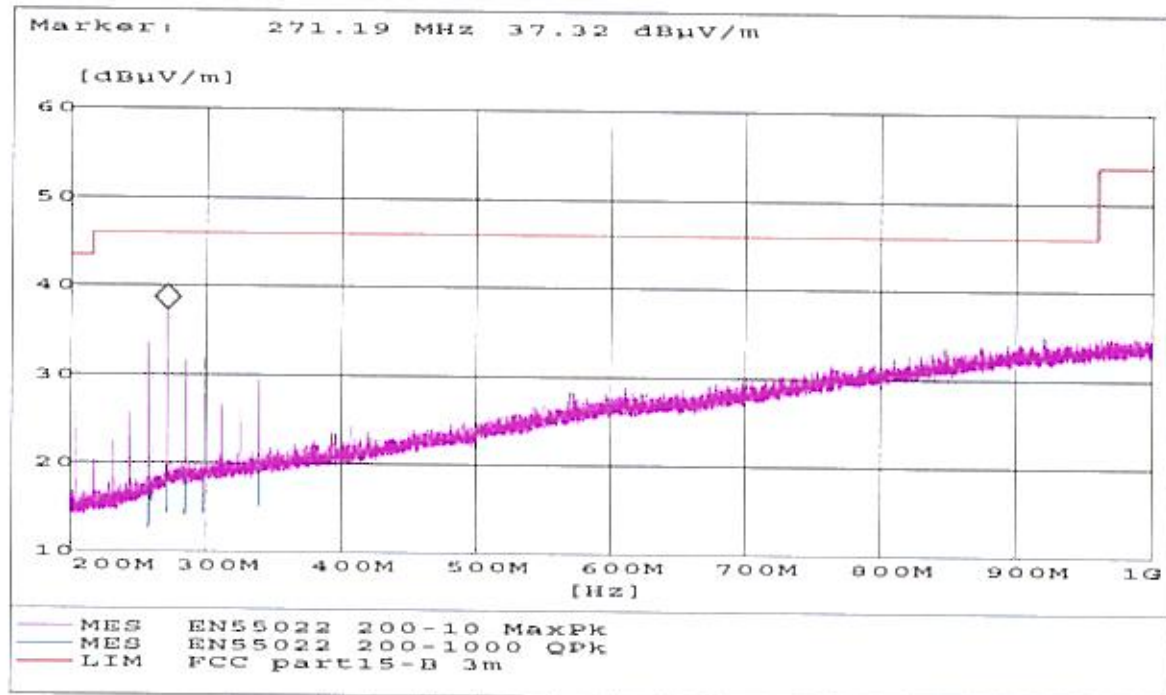
Horizontal antenna from 200MHz to 1000MHz
