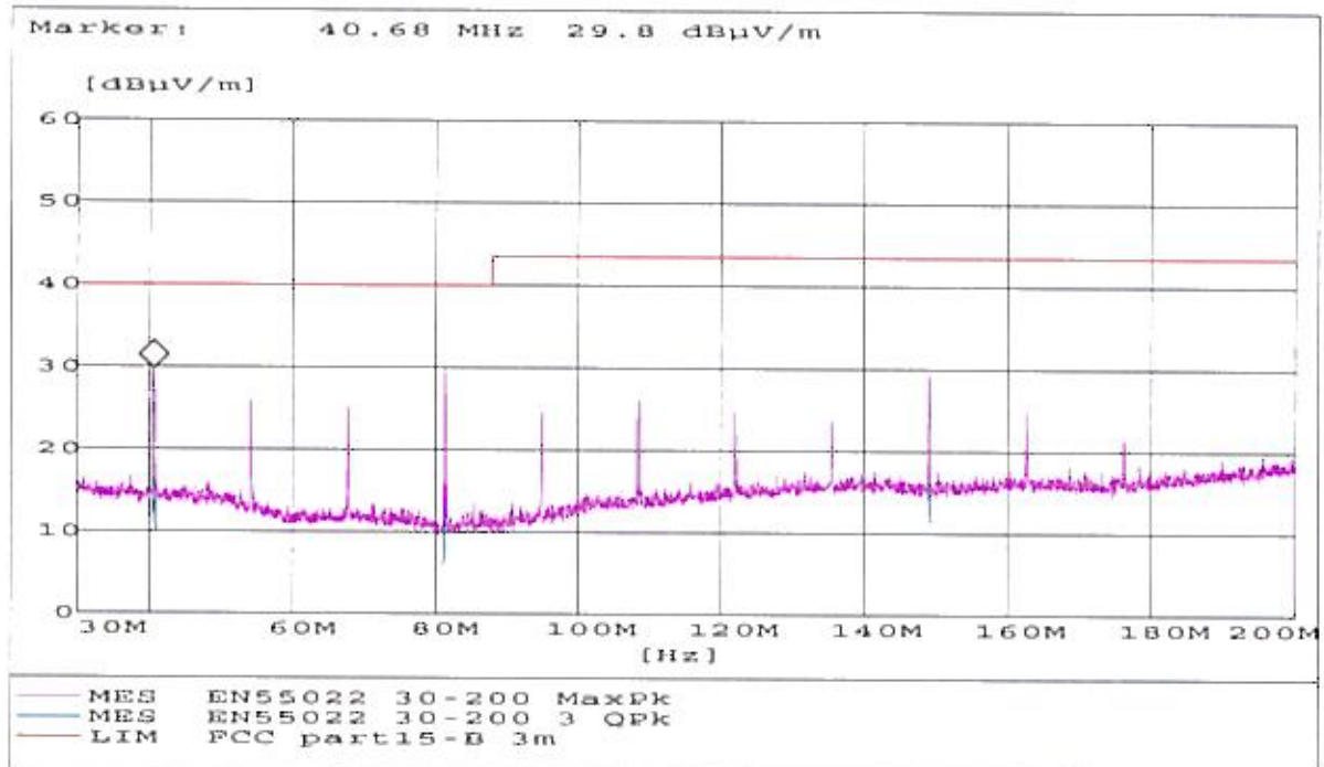
Vertical antenna from 30MHz to 200MHz
