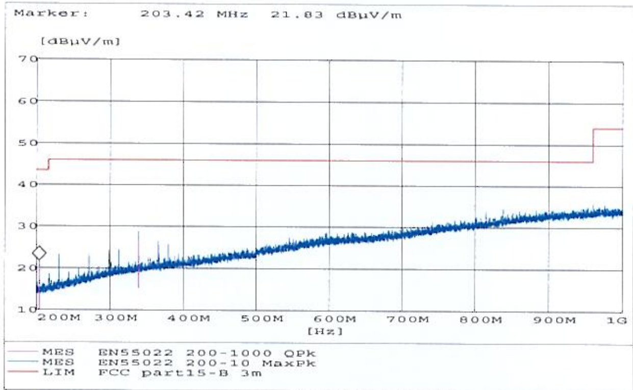
Horizontal antenna from 200MHz to 1000MHz
