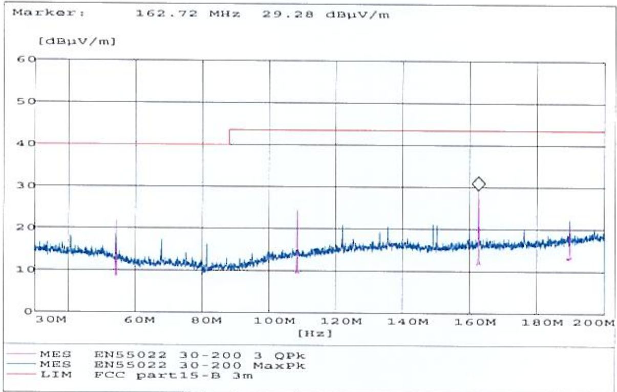
Horizontal antenna from 30MHz to 200MHz
