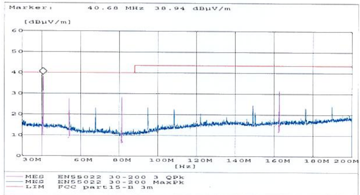
Vertical antenna from 30MHz to 200MHz
