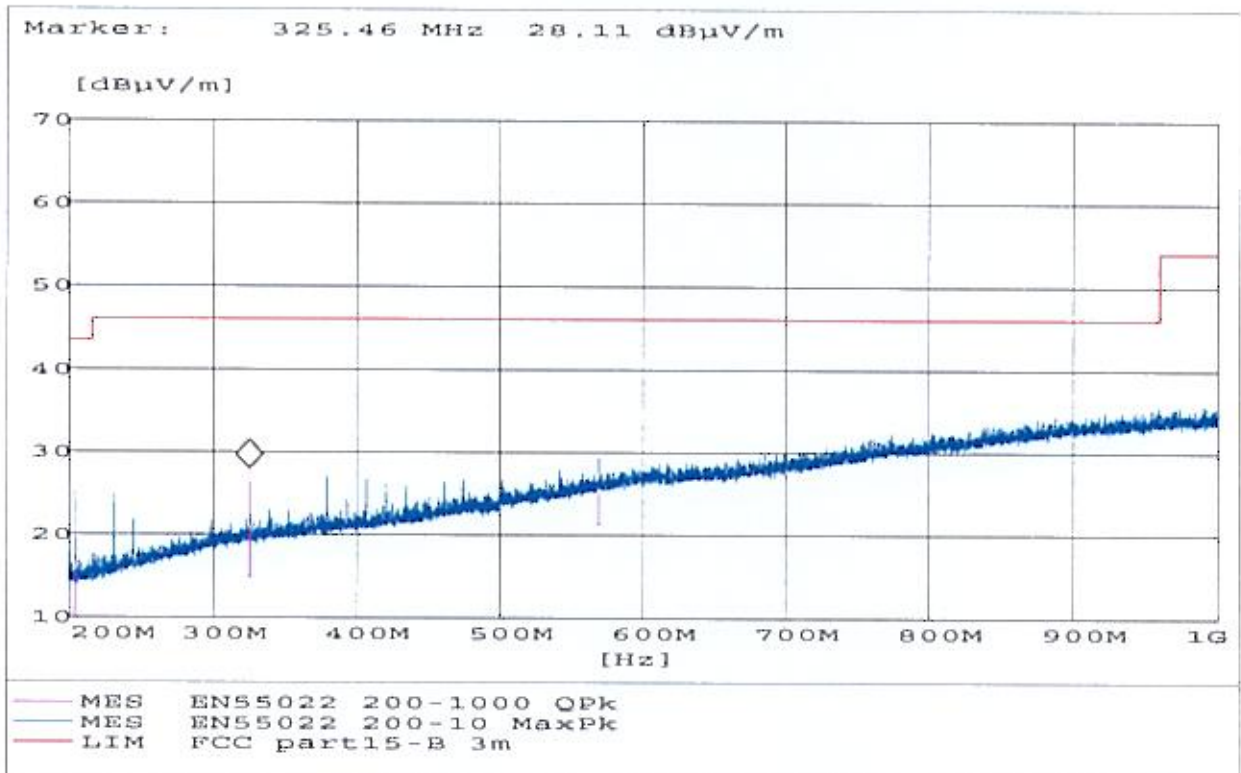
Verical antenna from 200MHz to 1000MHz
