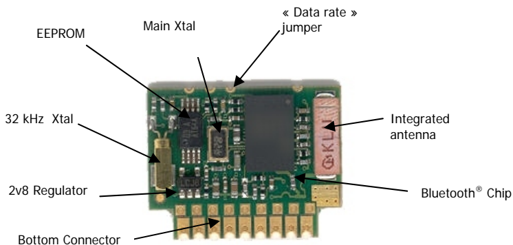
INTERNAL VIEW
