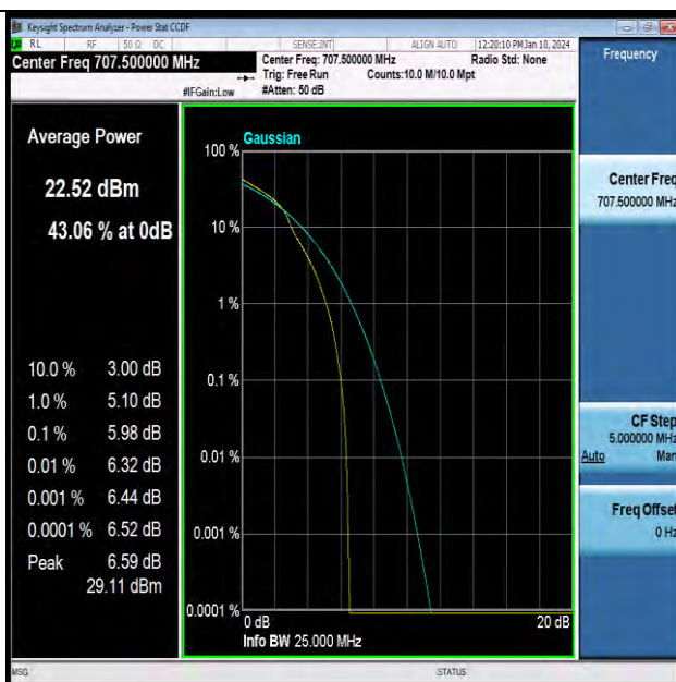
Band12-10MHz-16QAM-23095-1RB#0-PASS
