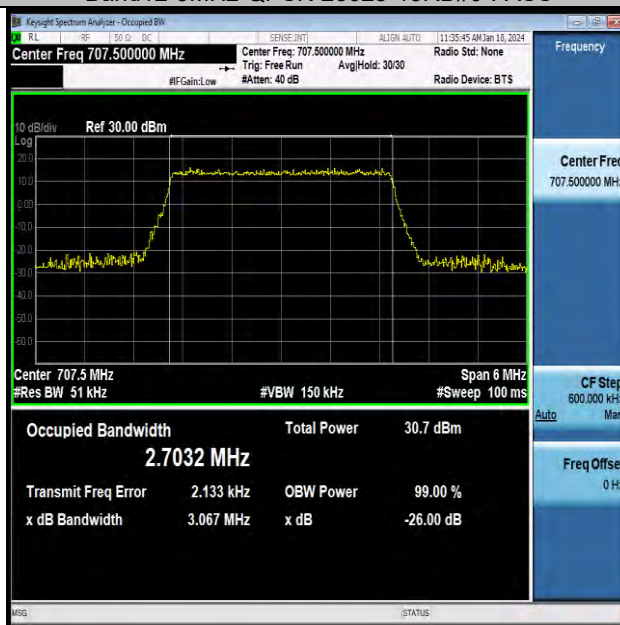
Band12-3MHz-QPSK-23095-15RB#0-PASS
