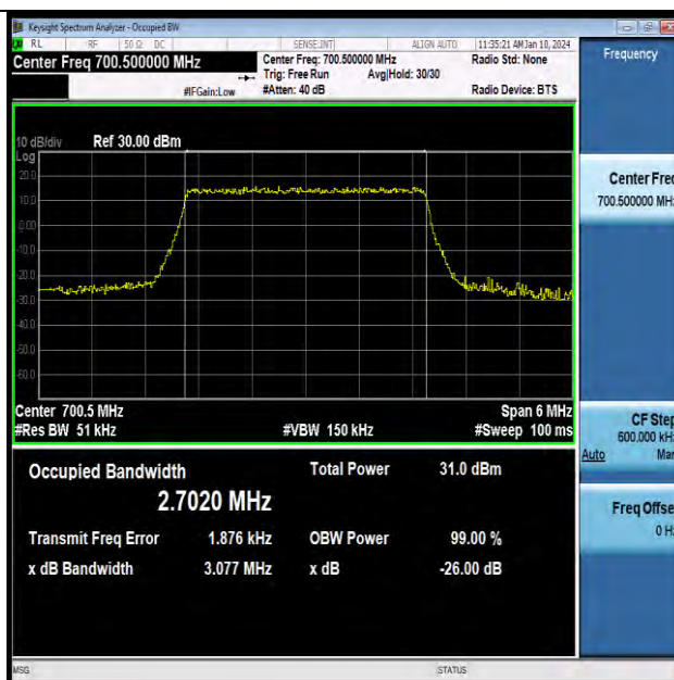
Band12-3MHz-QPSK-23025-15RB#0-PASS
