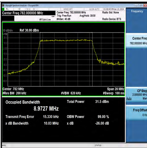
Band13-10MHz-QPSK-23230-50RB#0-PASS
