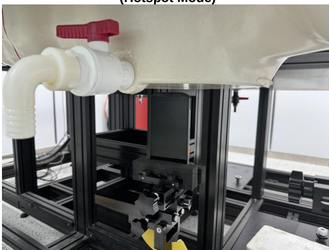
Bottom Side of EUT with 1 cm Gap (Hotspot Mode)
