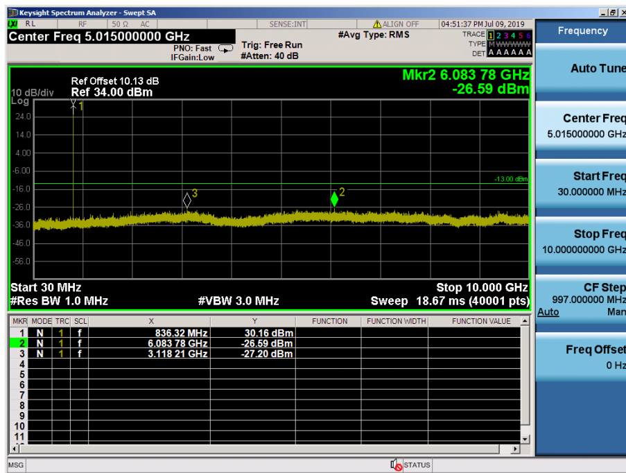
LTE Band 5, 26 / 1.4MHz / 16QAM - RB Size/Offset (1/0) – Mid Channel
