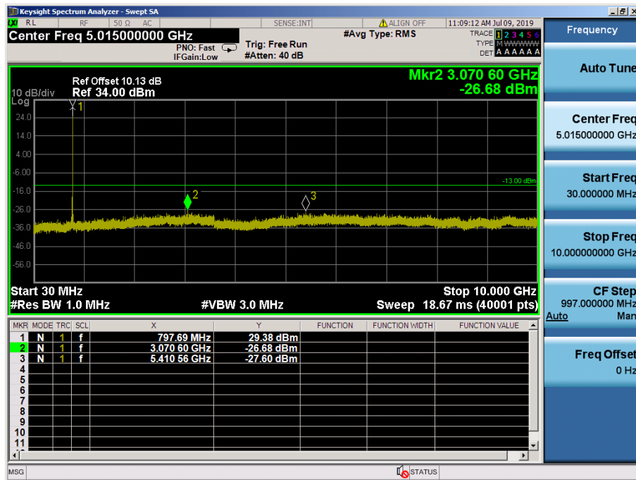
LTE Band 14 / 10MHz / 16QAM - RB Size/Offset (1/49) – Low Channel
