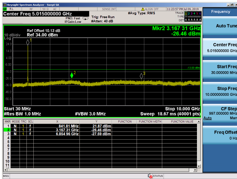
LTE Band 5, 26 / 10MHz / 64QAM - RB Size/Offset (50/0) – High Channel
