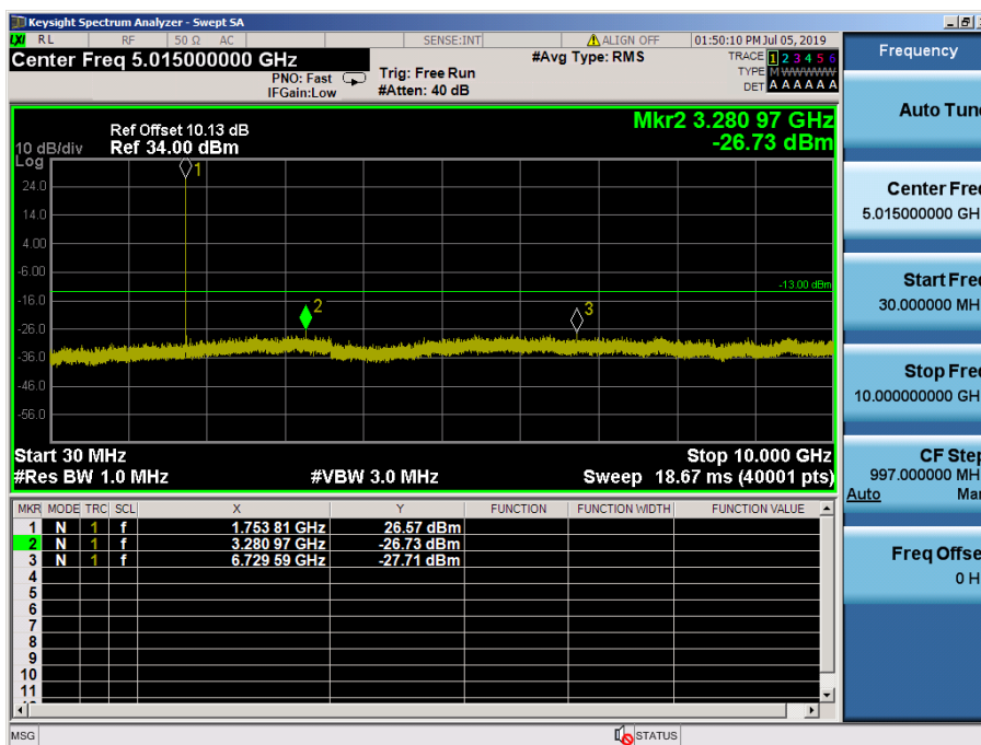
LTE Band 4 / 3MHz / 64QAM - RB Size/Offset (8/4) – High Channel
