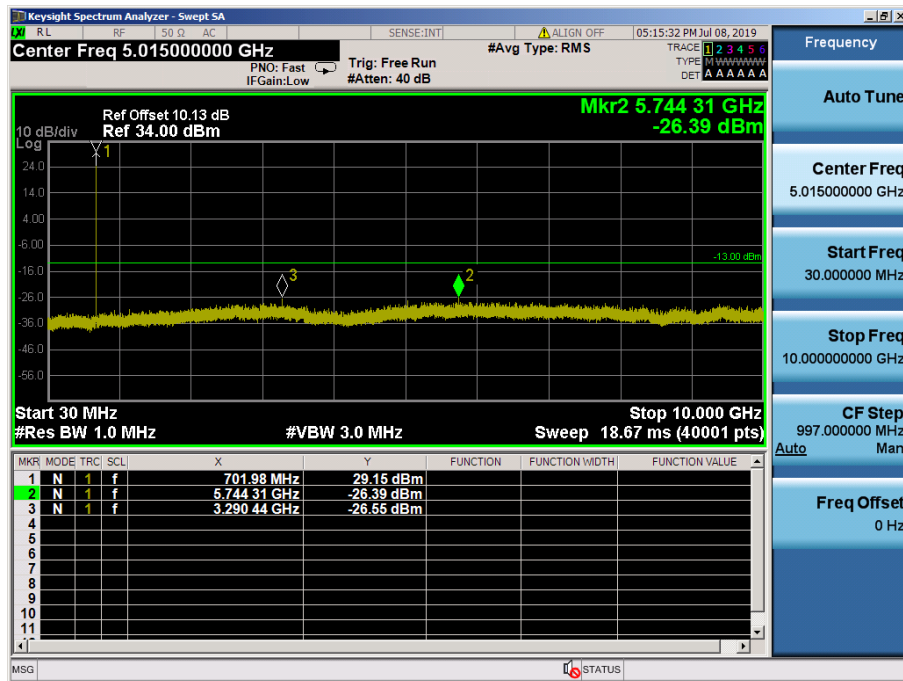
LTE Band 12 / 3MHz / 16QAM - RB Size/Offset (1/14) – Low Channel
