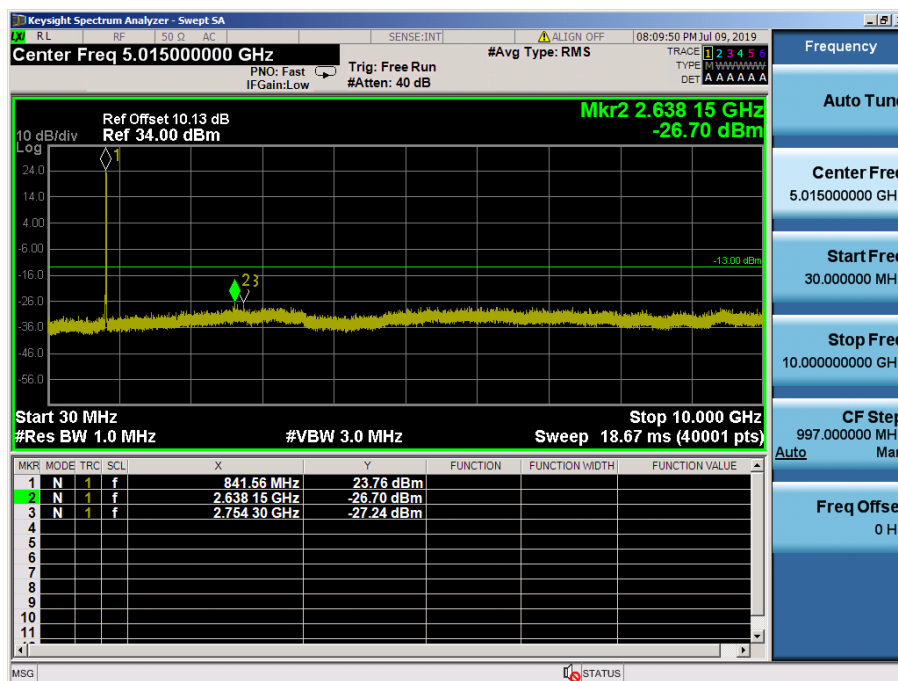
LTE Band 26 / 15MHz / 16QAM - RB Size/Offset (36/18) – High Channel
