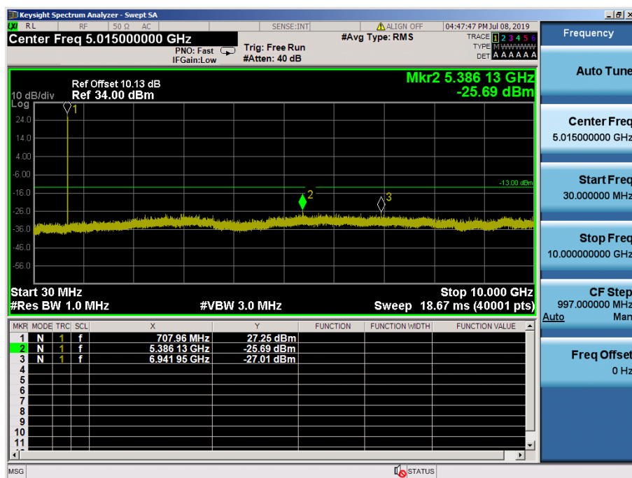
LTE Band 12 / 1.4MHz / 16QAM- RB Size/Offset (6/0) – Mid Channel
