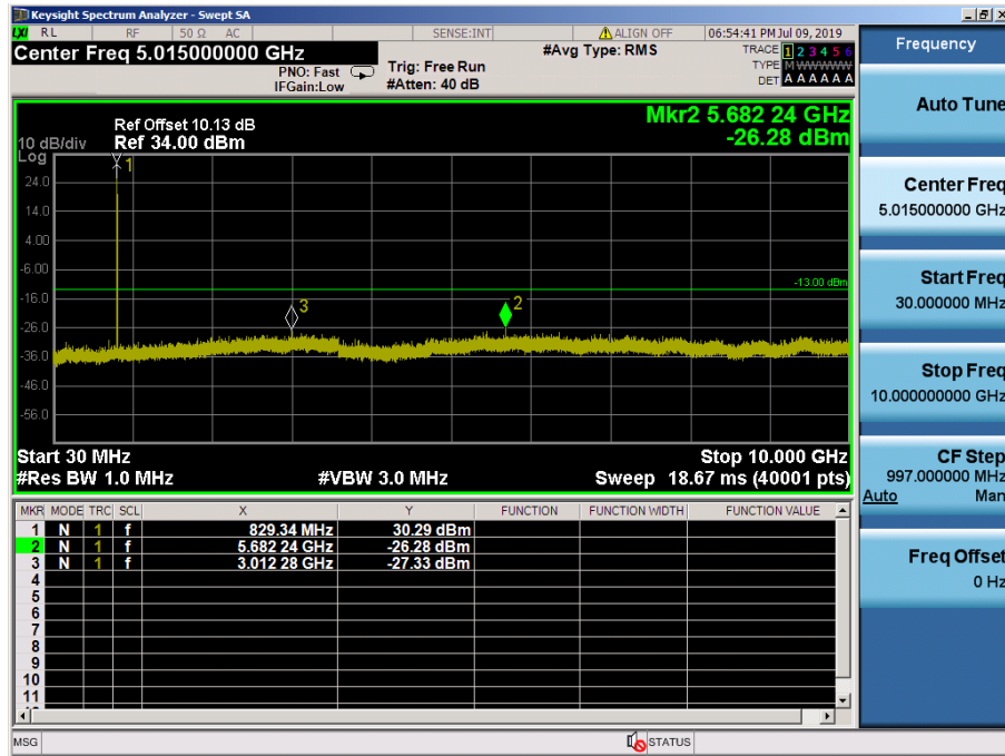
LTE Band 5, 26 / 10MHz / 16QAM - RB Size/Offset (1/25) – Low Channel
