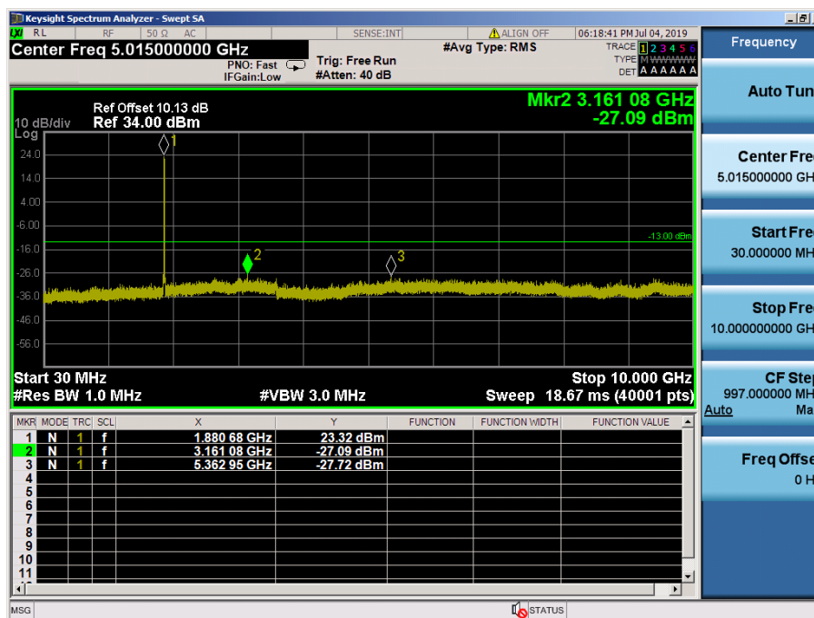
LTE Band 2, 25 / 10MHz / 16QAM - RB Size/Offset (25/0) – Mid Channel
