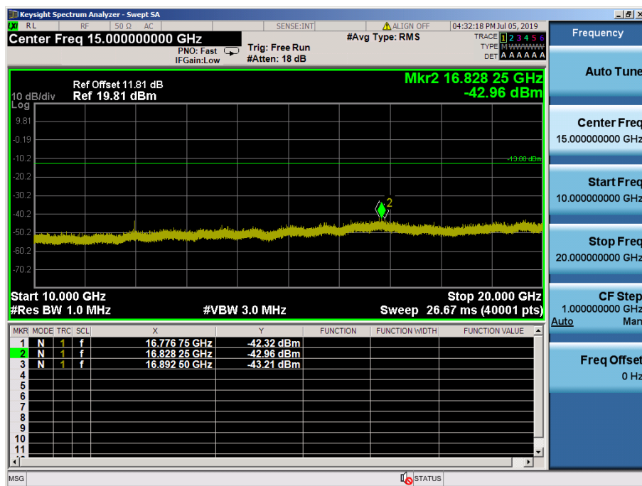
LTE Band 4 / 20MHz / 64QAM - RB Size/Offset (1/0) –Low Channel
