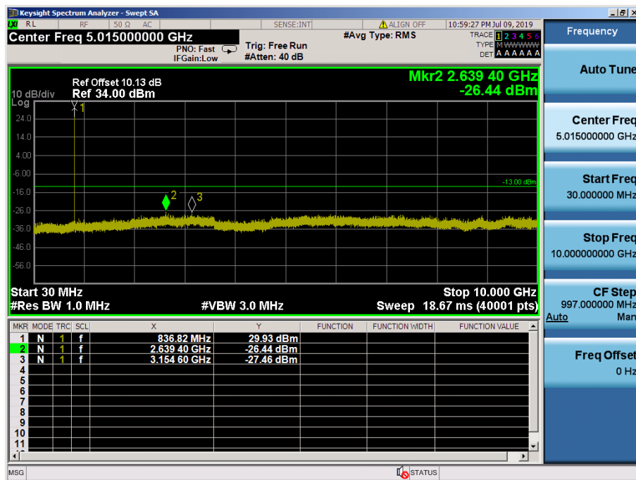
LTE Band 5, 26 / 10MHz / 64QAM - RB Size/Offset (1/25) – Mid Channel
