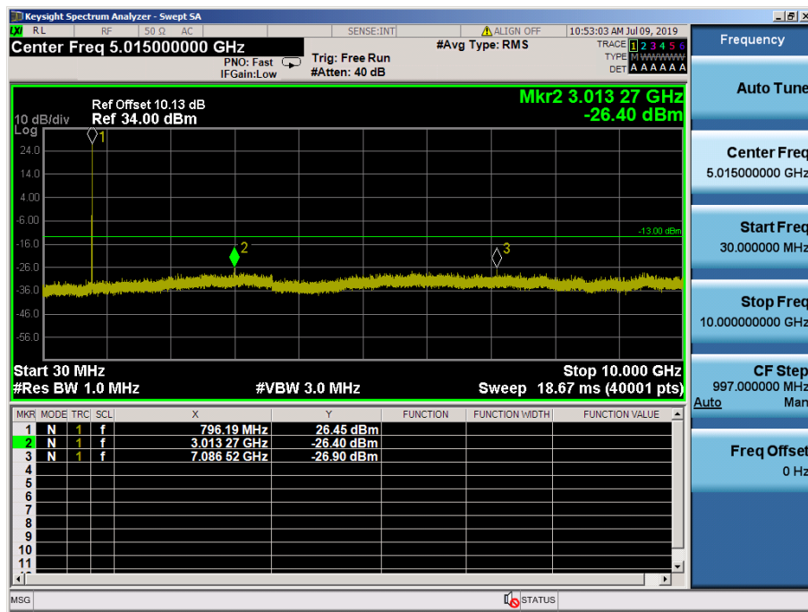
LTE Band 14 / 5MHz / 16QAM - RB Size/Offset (12/13) – High Channel
