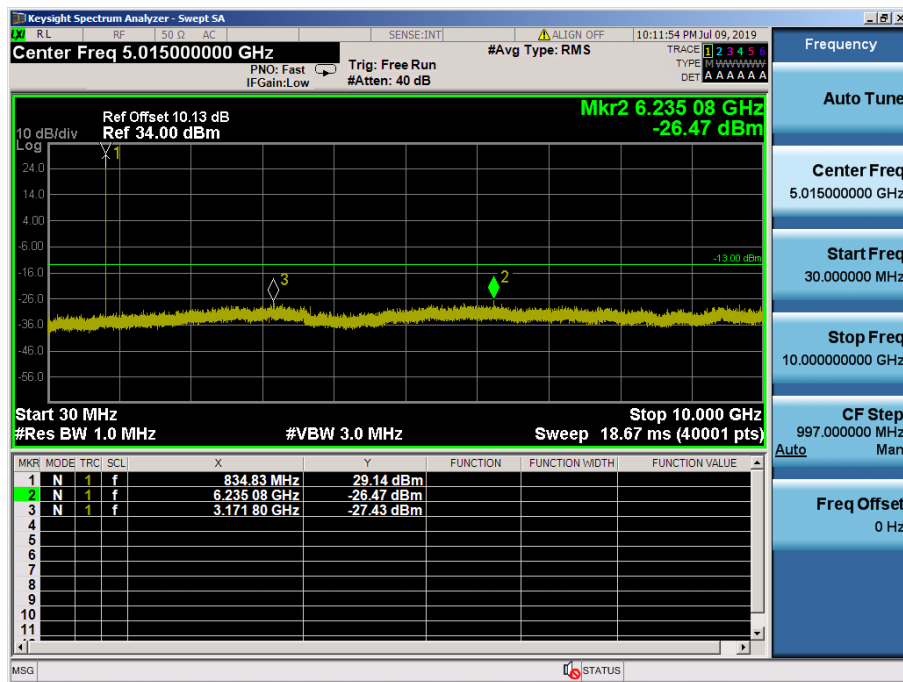
LTE Band 5, 26 / 5MHz / 64QAM - RB Size/Offset (1/0) – Mid Channel
