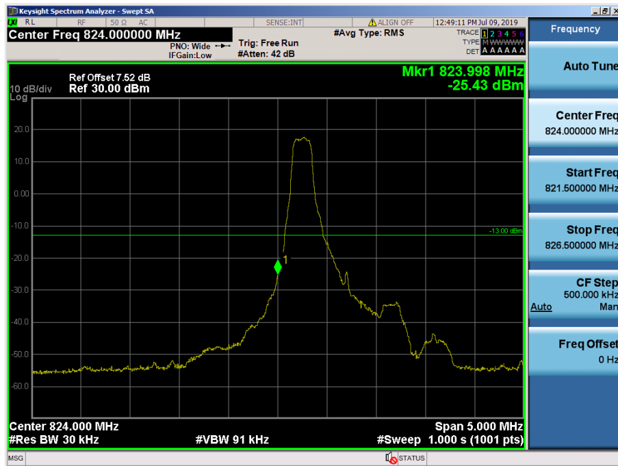
LTE Band 26 / 1.4MHz / QPSK - RB Size/Offset (1/0)
