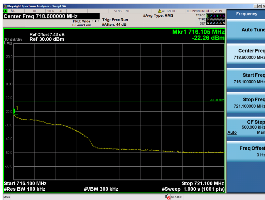
LTE Band 12, 17 / 5MHz / QPSK - RB Size/Offset (12/13)
