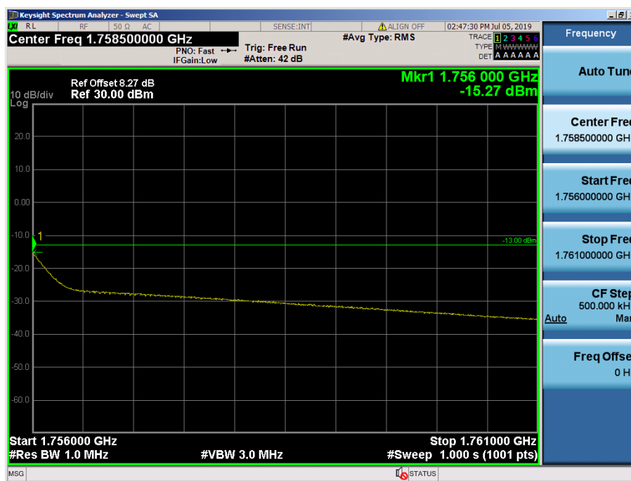
LTE Band 4 / 5MHz / 64QAM - RB Size/Offset (25/0)
