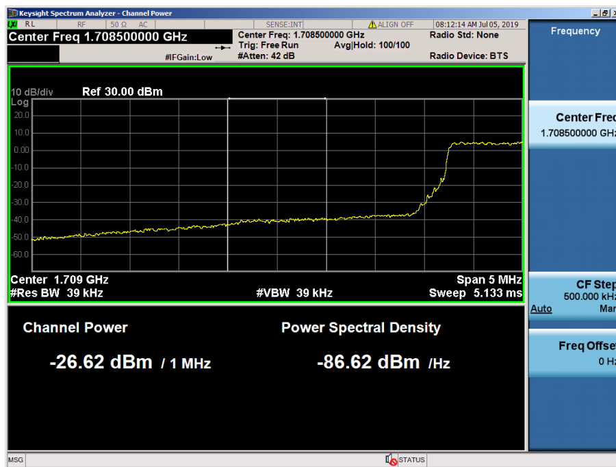
LTE Band 4 / 5MHz / 16QAM Offset/Size (12/0)
