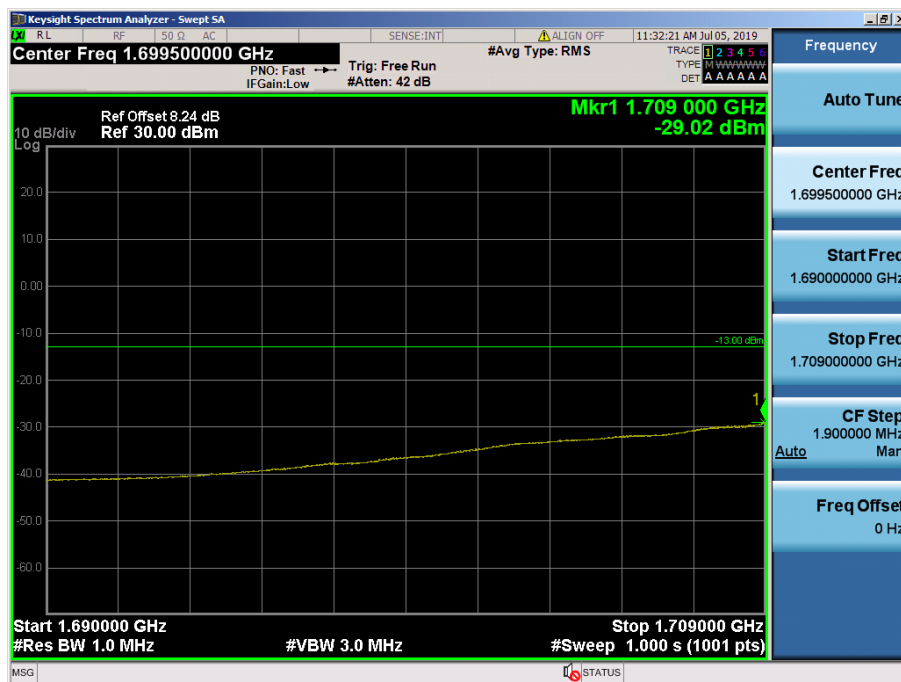
LTE Band 4 / 20MHz / 16QAM - RB Size/Offset (50/0)
