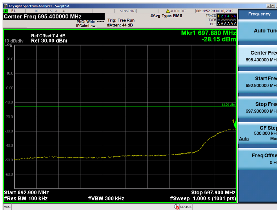
LTE Band 12, 17 / 5MHz / QPSK RB - Size/Offset (12/0)
