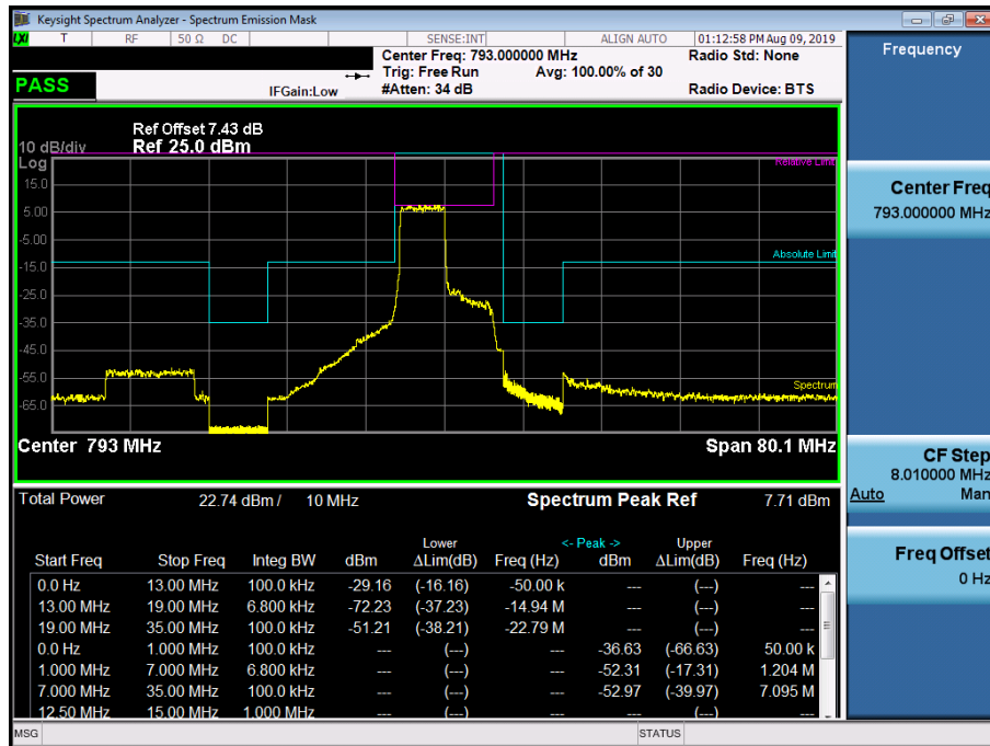
LTE Band 14 / 10MHz / QPSK - RB Size/Offset (25/0)
