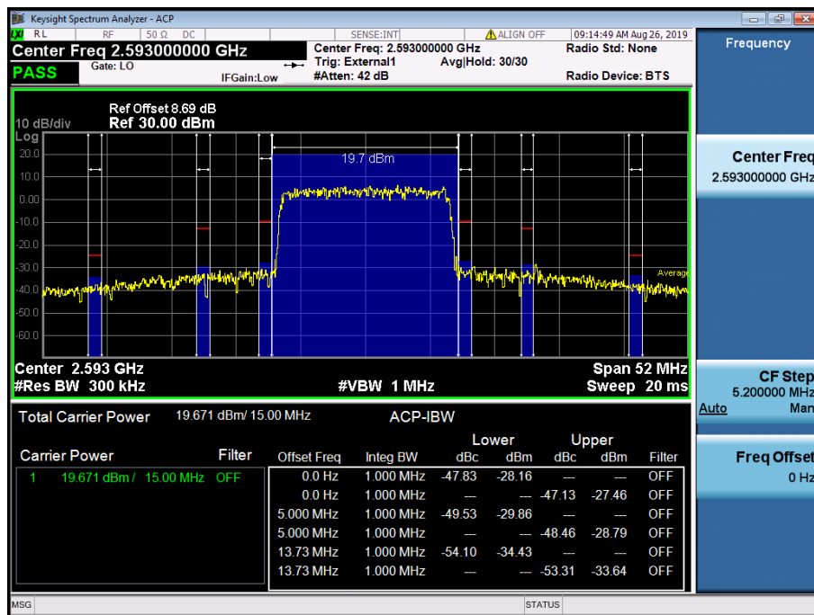
LTE Band 41 / 15MHz / 64QAM - RB Size/Offset (75/0)
