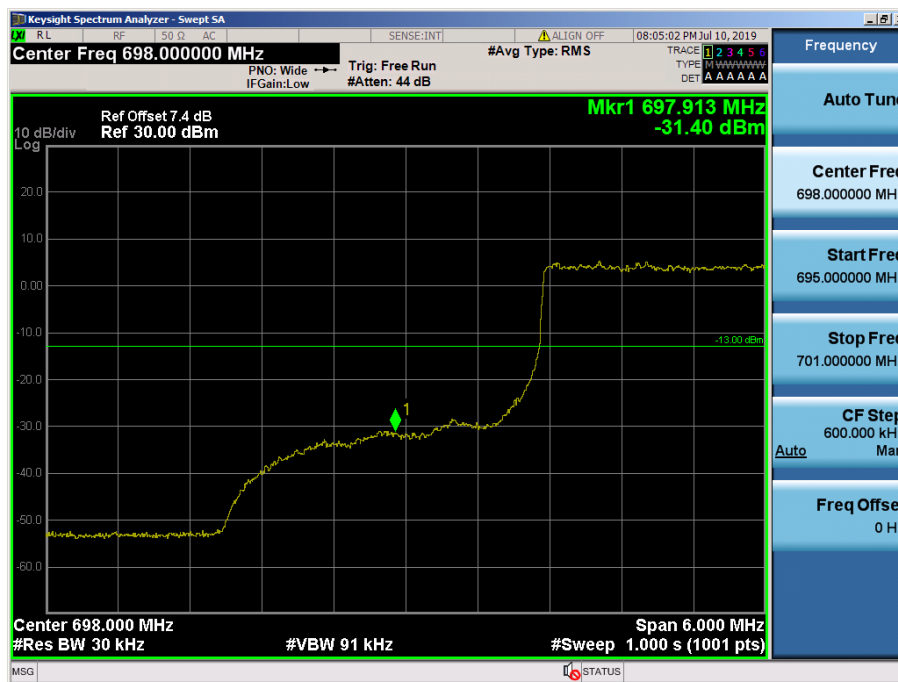
LTE Band 12 / 3MHz / 16QAM - RB Size/Offset (15/0)
