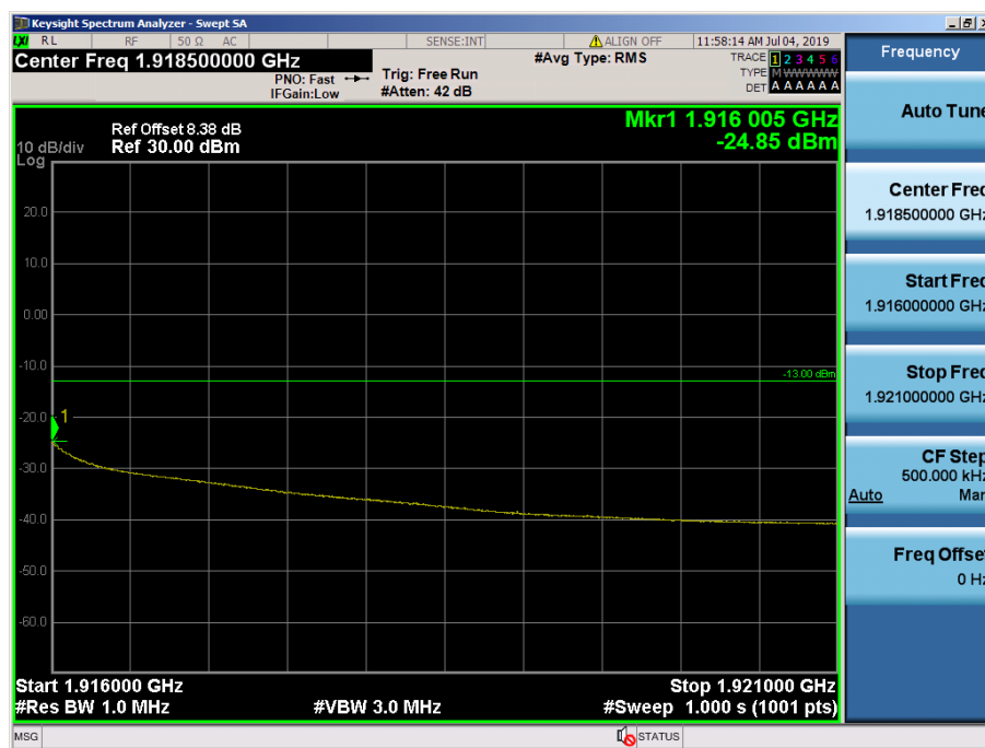
LTE Band 25 / 3MHz / QPSK - RB Size/Offset (8/4)
