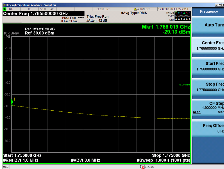
LTE Band 4 / 20MHz / 16QAM - RB Size/Offset (50/50)
