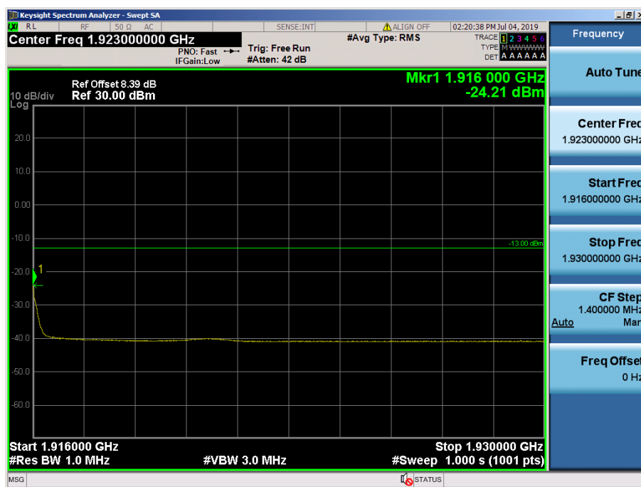
LTE Band 25 / 15MHz / QPSK - RB Size/Offset (1/74)
