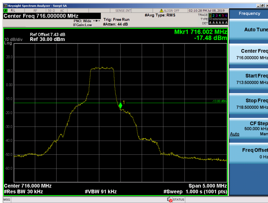
LTE Band 12 / 1.4MHz / QPSK - RB Size/Offset (3/3)
