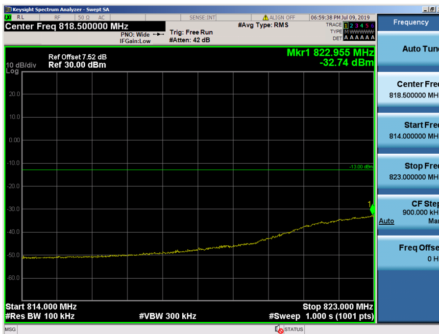
LTE Band 26 / 10MHz / 16QAM - RB Size/Offset (25/0)
