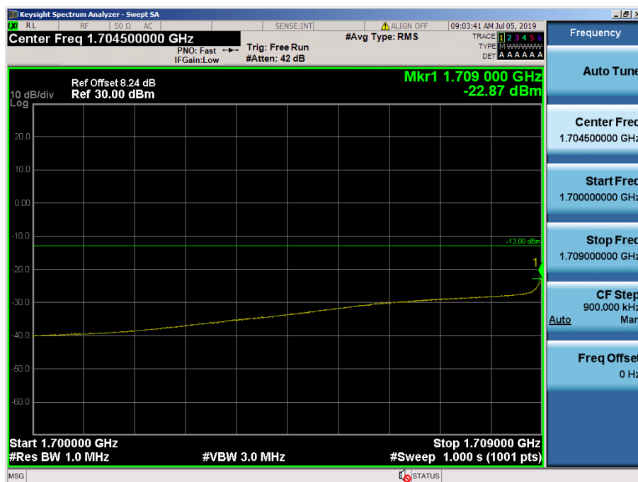
LTE Band 4 / 10MHz / 16QAM - RB Size/Offset (25/0)
