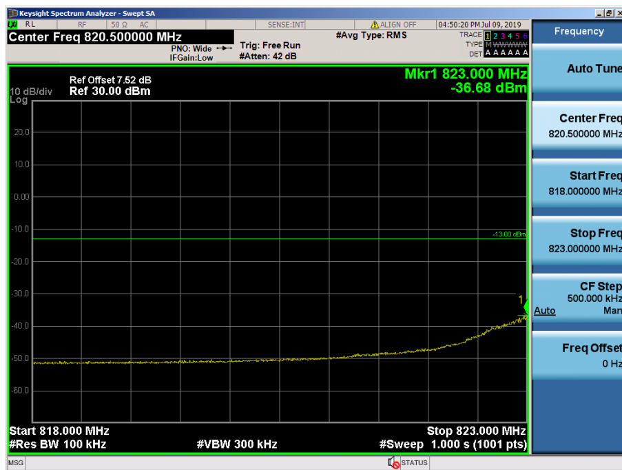
LTE Band 26 / 1.4MHz / 16QAM - RB Size/Offset (6/0)
