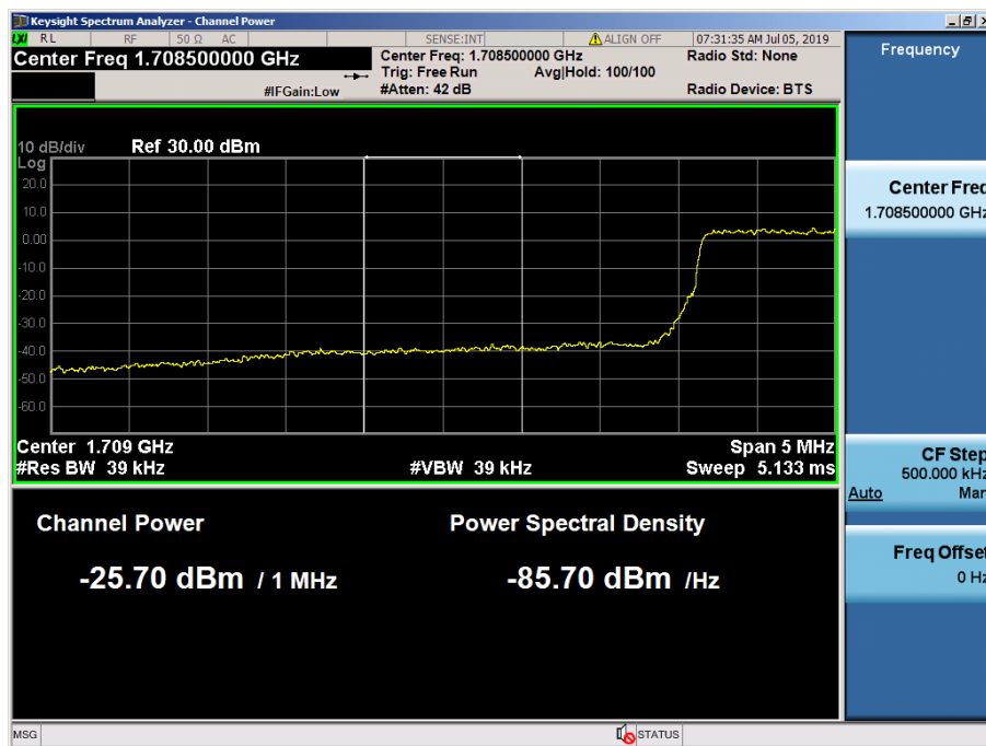
LTE Band 4 / 3MHz / 16QAM - RB Size/Offset (15/0)
