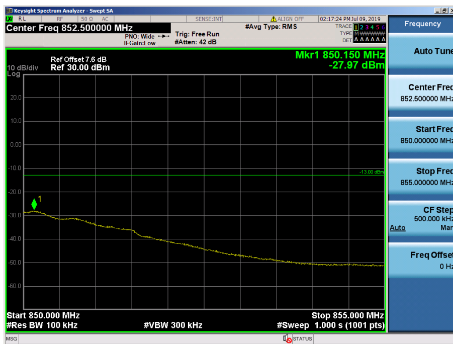
LTE Band 26 / 3MHz / QPSK - RB Size/Offset (15/0)
