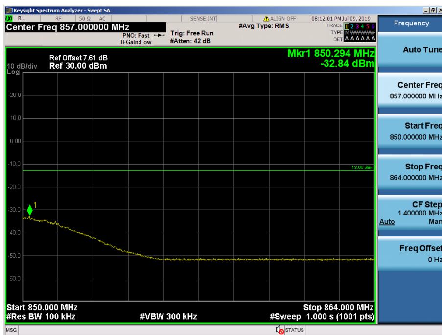
LTE Band 26 / 15MHz / 16QAM - RB Size/Offset (36/39)
