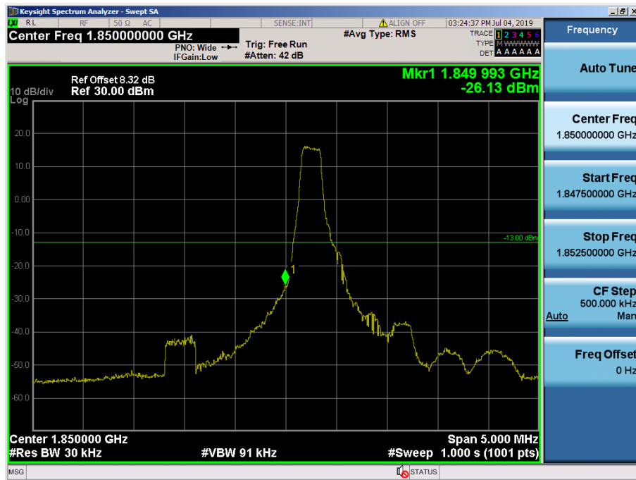
LTE Band 25 / 1.4MHz / 16QAM - RB Size/Offset (1/0)
