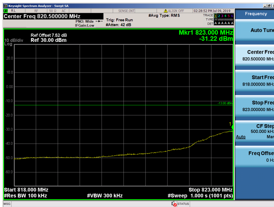
LTE Band 26 / 5MHz / QPSK - RB Size/Offset (12/0)
