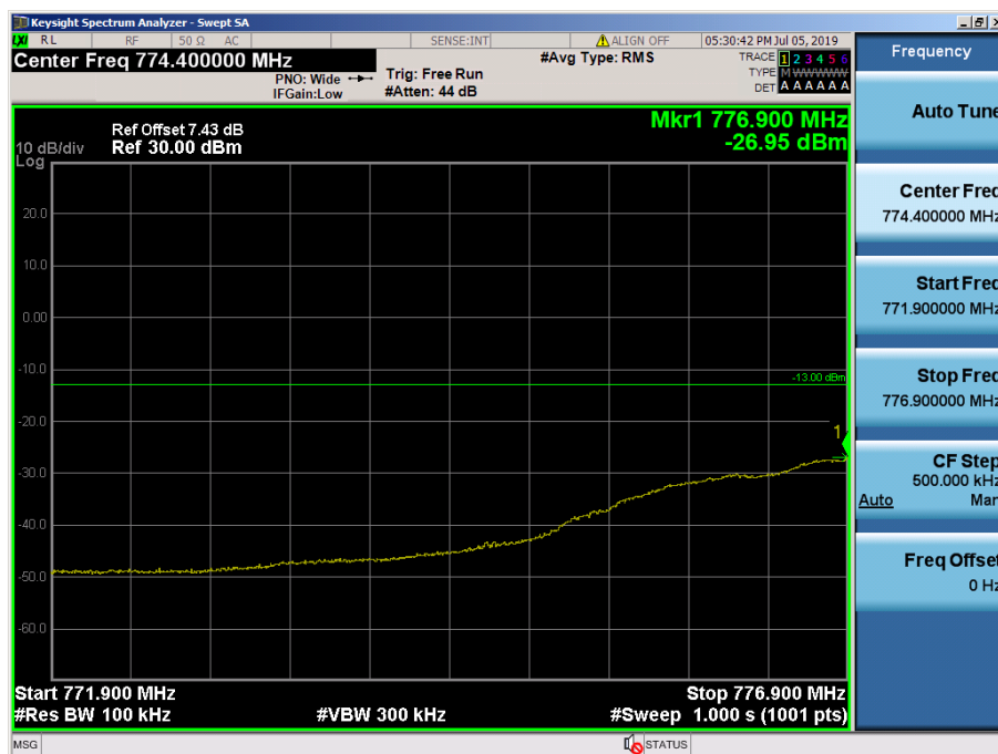
LTE Band 13 / 5MHz / QPSK - RB Size/Offset (12/0)
