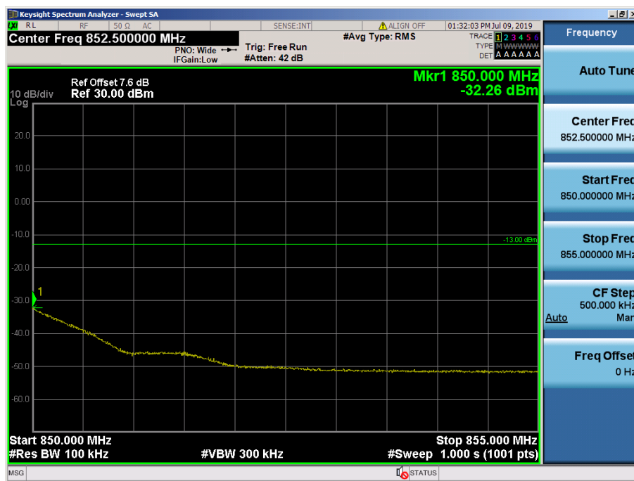
LTE Band 26 / 1.4MHz / QPSK - RB Size/Offset (6/0)
