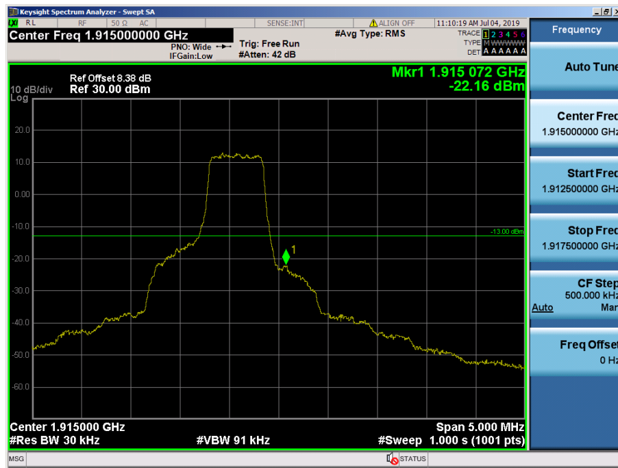
LTE Band 25 / 1.4MHz / QPSK - RB Size/Offset (3/3)
