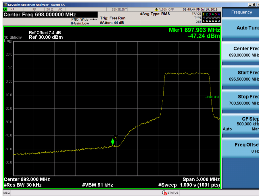
LTE Band 12 / 1.4MHz / 64QAM - RB Size/Offset (6/0)
