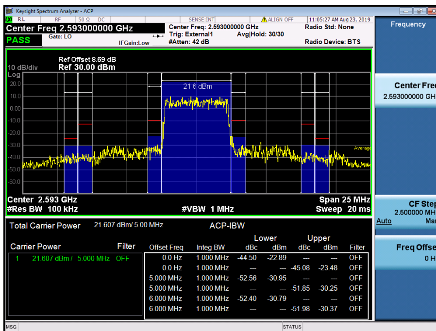
LTE Band 41 / 5MHz / QPSK - RB Size/Offset (25/0)
