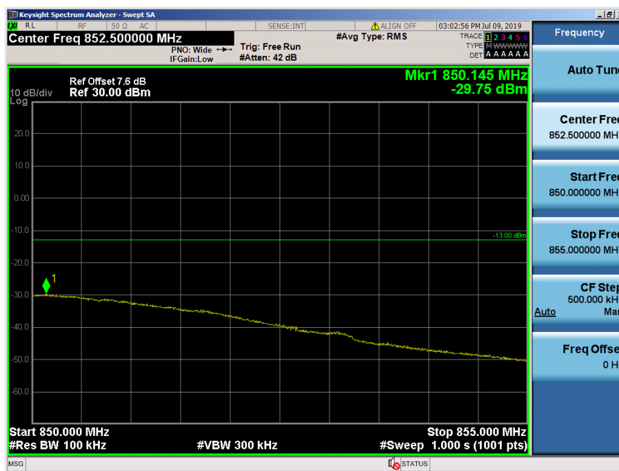
LTE Band 26 / 5MHz / QPSK - RB Size/Offset (25/0)
