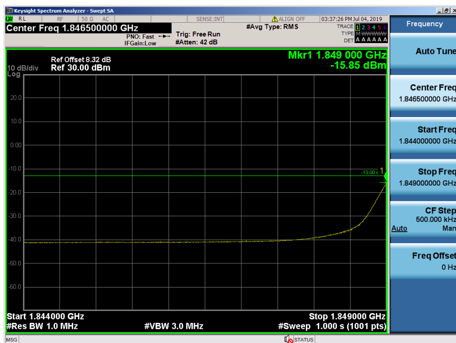
LTE Band 25 / 1.4MHz / 16QAM - RB Size/Offset (3/2)
