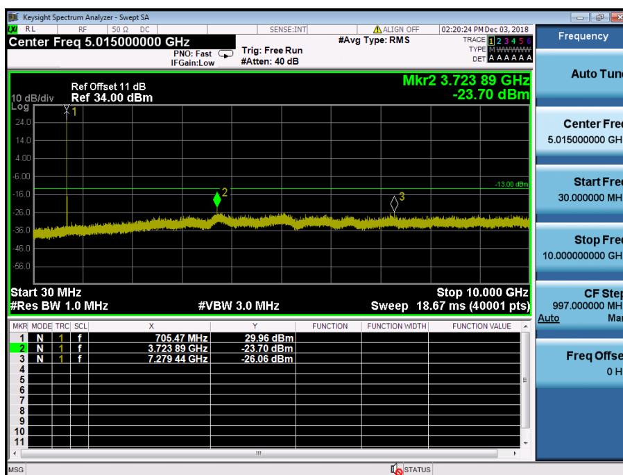
LTE Band 12, 17 / 5MHz / QPSK - RB Size/Offset (1/0) – Mid Channel
