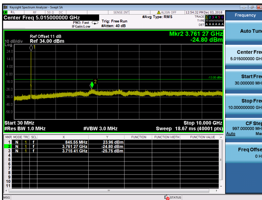
LTE Band 5 / 10MHz / 16QAM - RB Size/Offset (50/0) – High Channel
