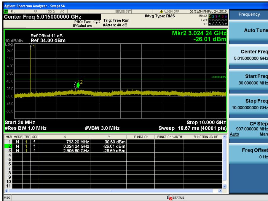
LTE Band 14 / 10MHz / QPSK - RB Size/Offset (1/25) – Low Channel
