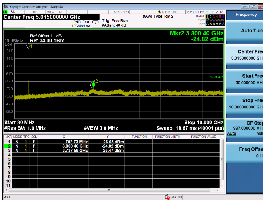
LTE Band 12, 17 / 5MHz / 16QAM - RB Size/Offset (25/0) – Low Channel
