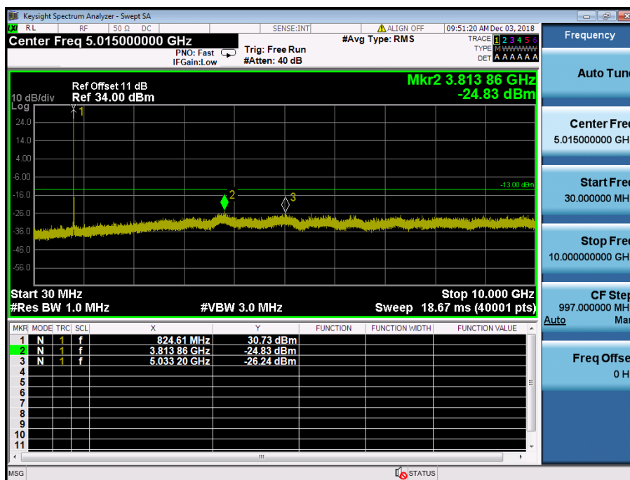
LTE Band 5 / 10MHz / QPSK - RB Size/Offset (1/0) – Low Channel
