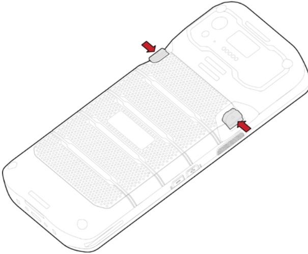
Figure 13 Removing battery – 1
