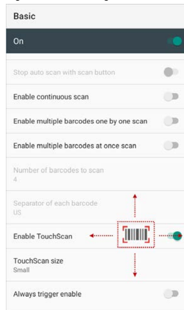
Figure 55 ScanSettings - TouchScan
