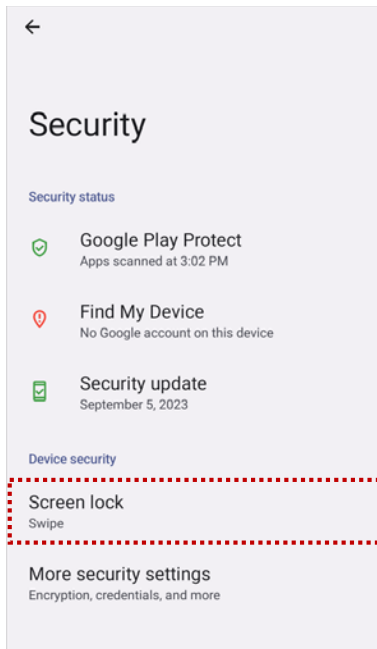
Figure 46 Screen lock
