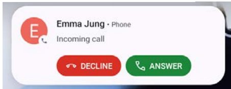
Figure 35 Receiving call
