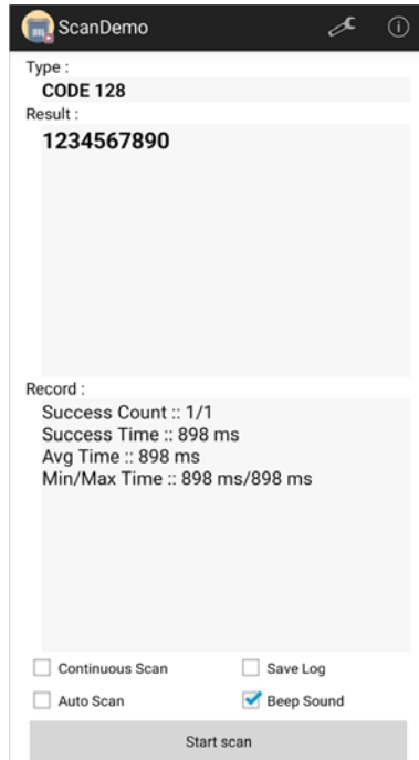
Figure 68 ScanDemo
