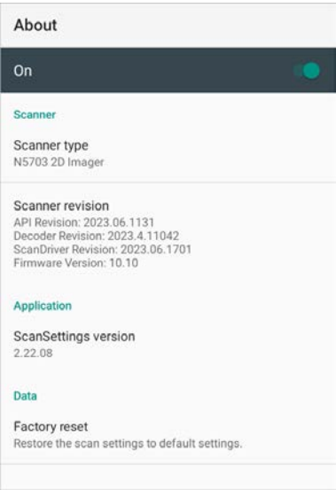
Figure 66 ScanSettings - About
