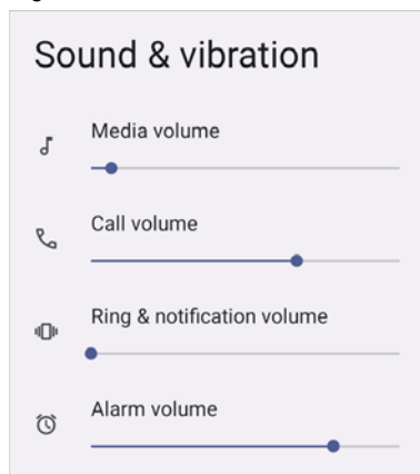
Figure 49 Volume bars
