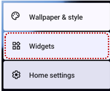
Figure 32 Widget menus
