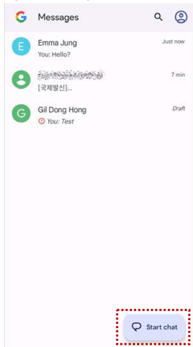
Figure 39 Message list
