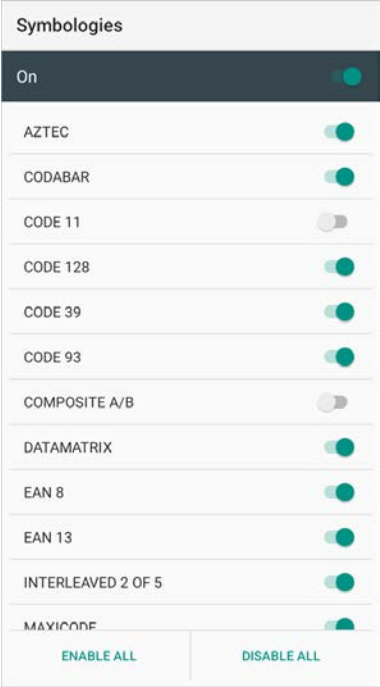
Figure 65 ScanSettings - Symbologies
