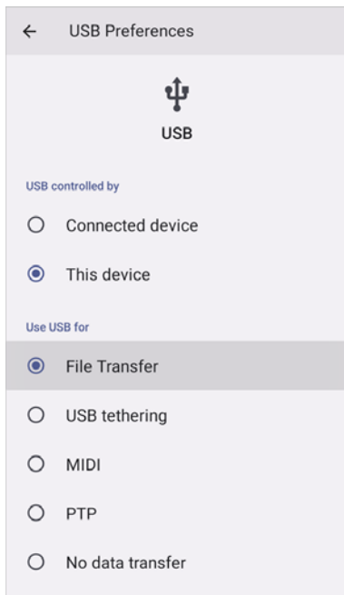
Figure 42 USB Preferences
