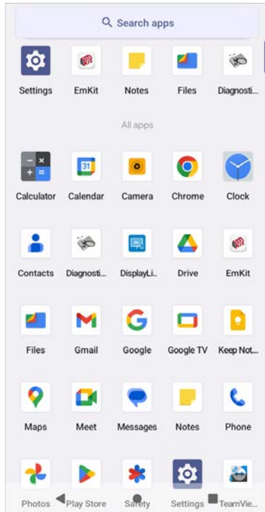
Figure 28 App drawer
