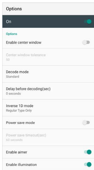
Figure 56 ScanSettings - Options
