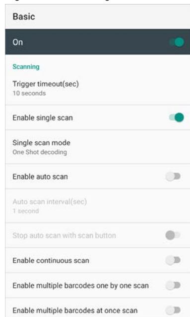
Figure 54 ScanSettings - Basic
