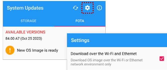
Figure 86 FOTA Settings
