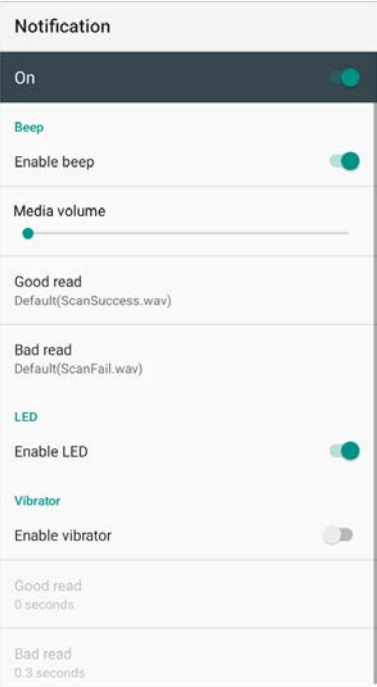
Figure 57 ScanSettings - Notification
