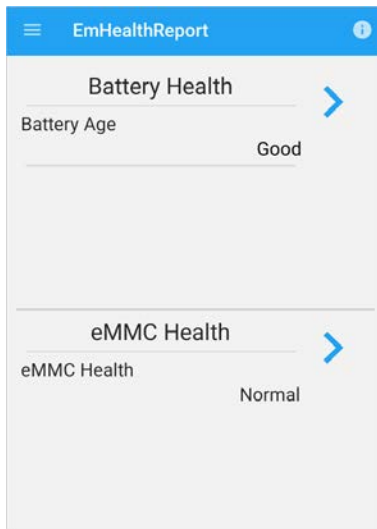
Figure 83 EmHealthReport
