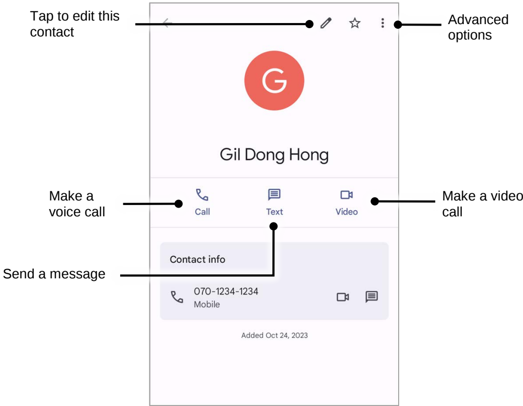
Figure 37 Contact detail
