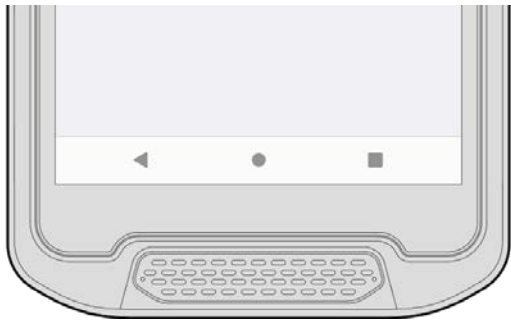
Figure 19 Navigation bar
