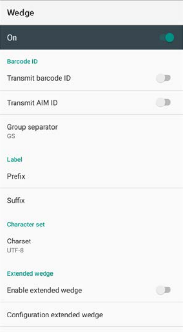
Figure 58 ScanSettings - Wedge
