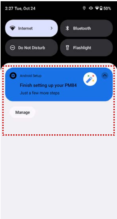
Figure 24 Notification panel
