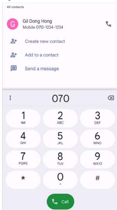
Figure 33 Dialer
