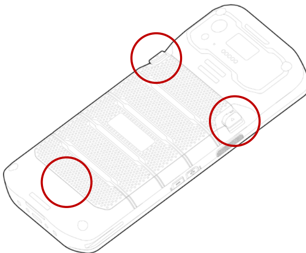
Figure 12 Installing battery – 2
