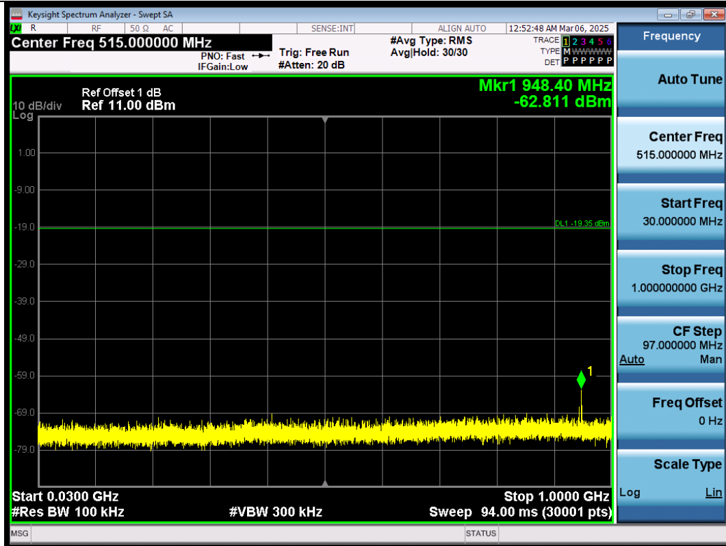
11B-Ant1-2437-30~1000-PASS
