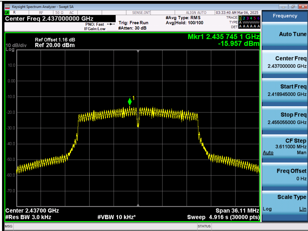
11N20SISO-Ant1-2437-PASS
