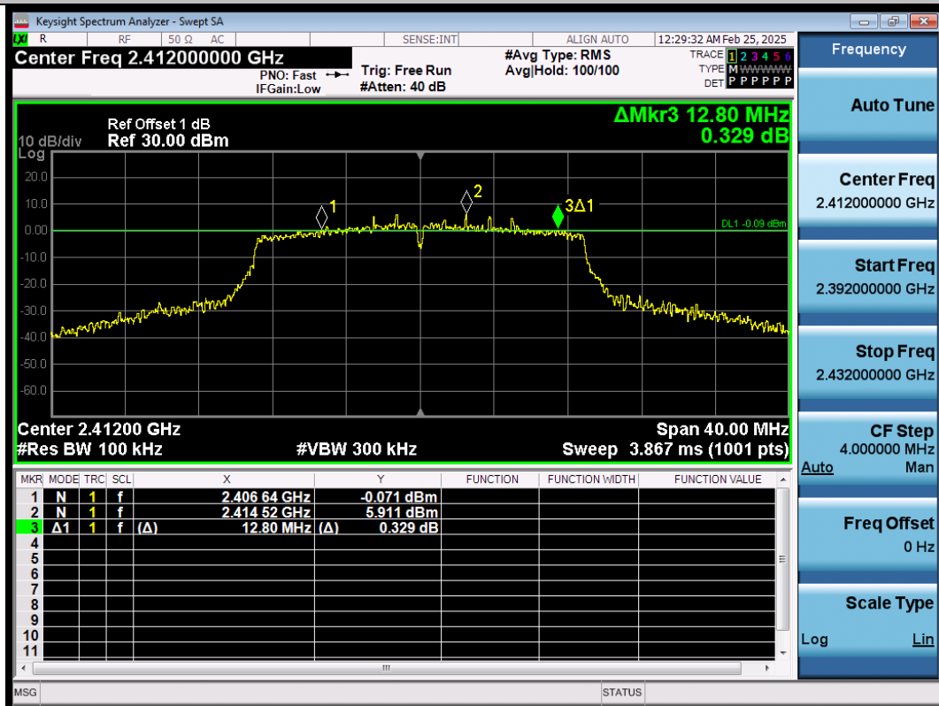
11N20SISO-Ant1-2412-PASS
