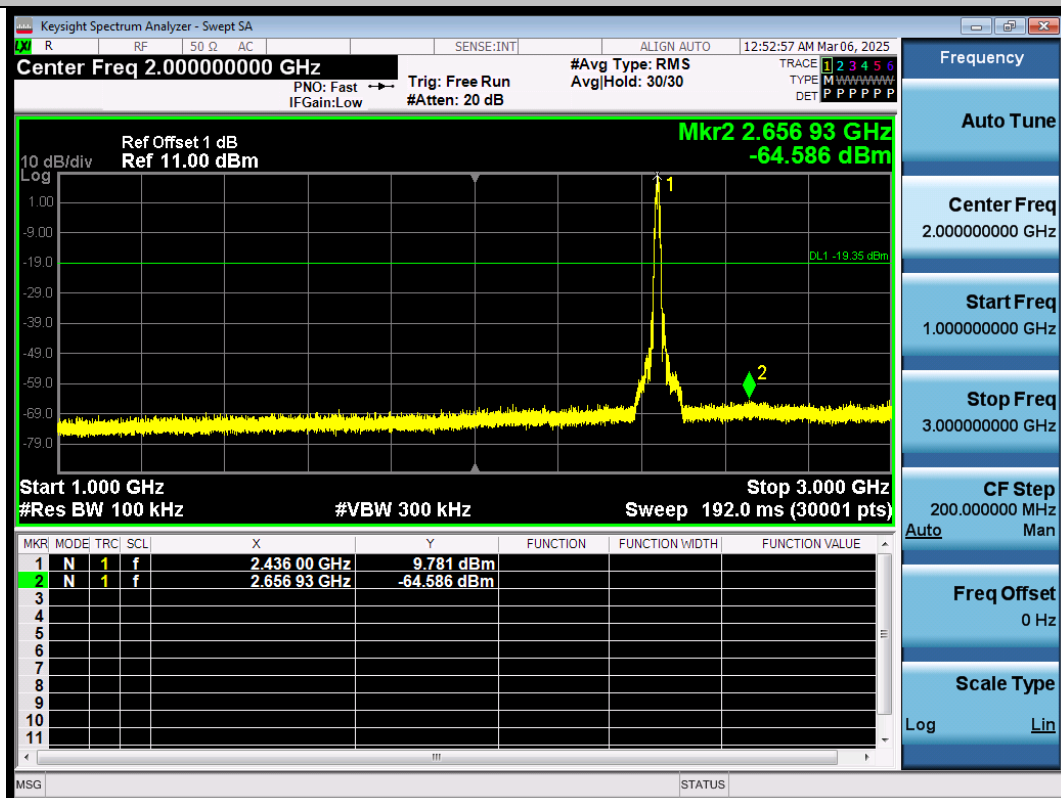
11B-Ant1-2437-1000~3000-PASS
