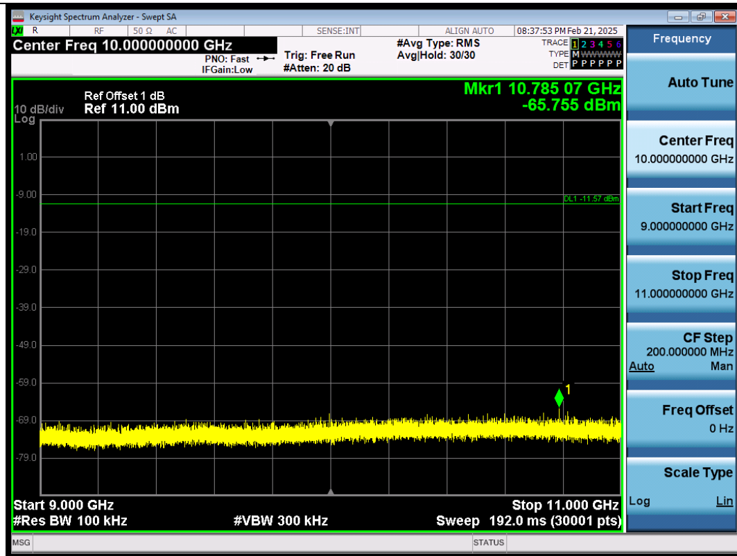
DH5-Ant1-2402-9000~11000-PASS
