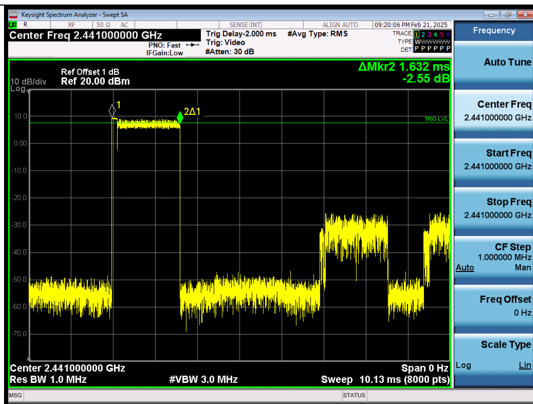
3DH3-Ant1-Hop-PASS
