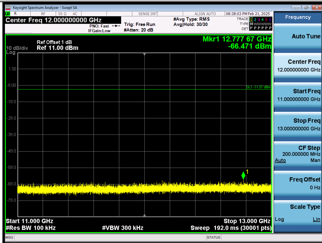
DH5-Ant1-2402-11000~13000-PASS
