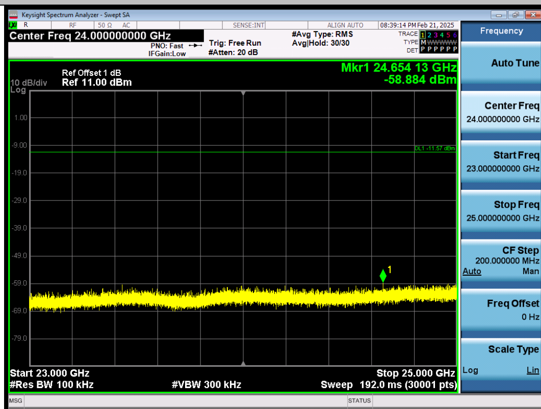
DH5-Ant1-2402-23000~25000-PASS
