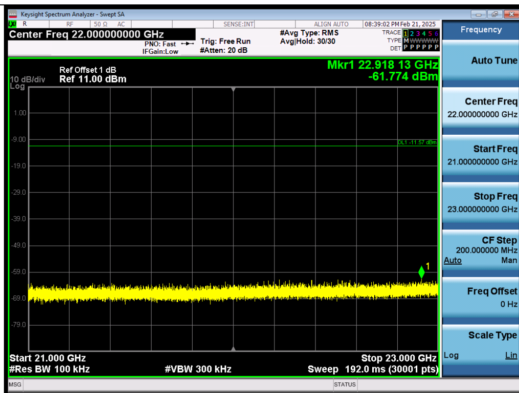
DH5-Ant1-2402-21000~23000-PASS
