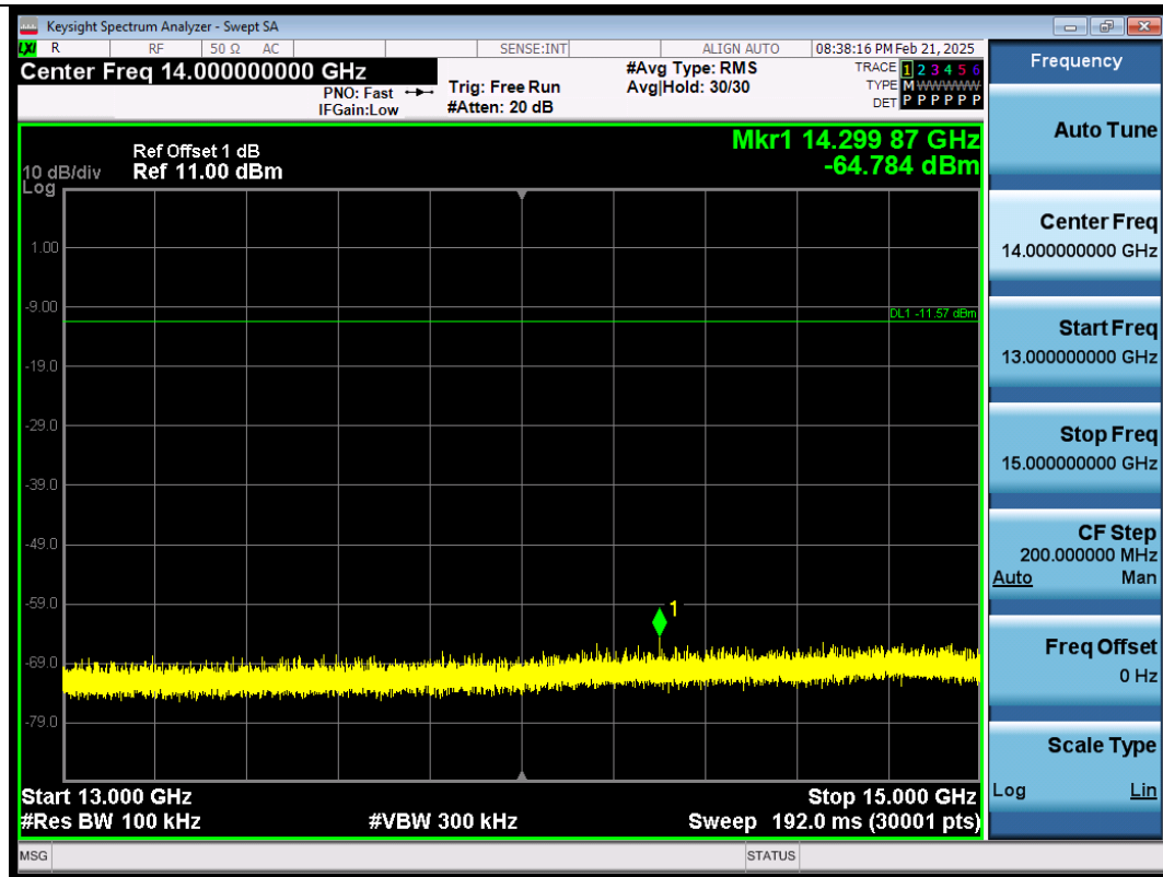
DH5-Ant1-2402-13000~15000-PASS
