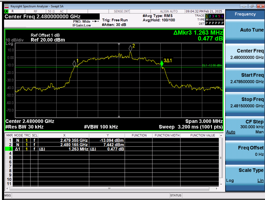
3DH5-Ant1-2480
