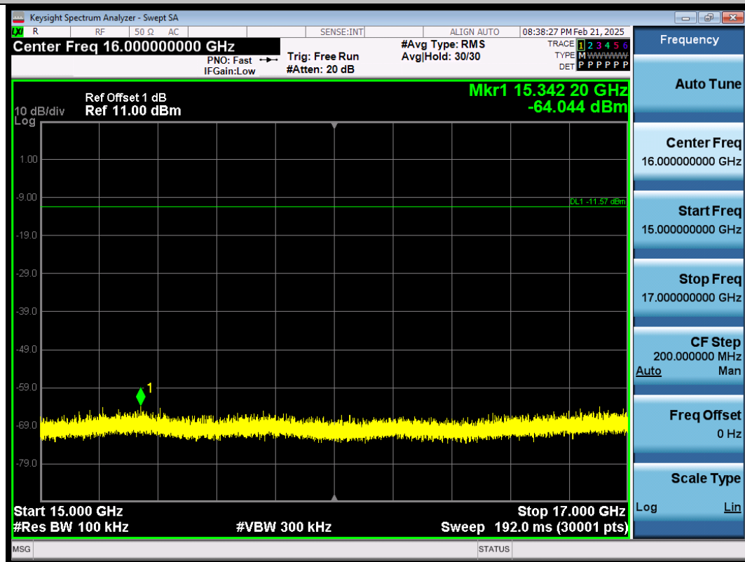
DH5-Ant1-2402-15000~17000-PASS
