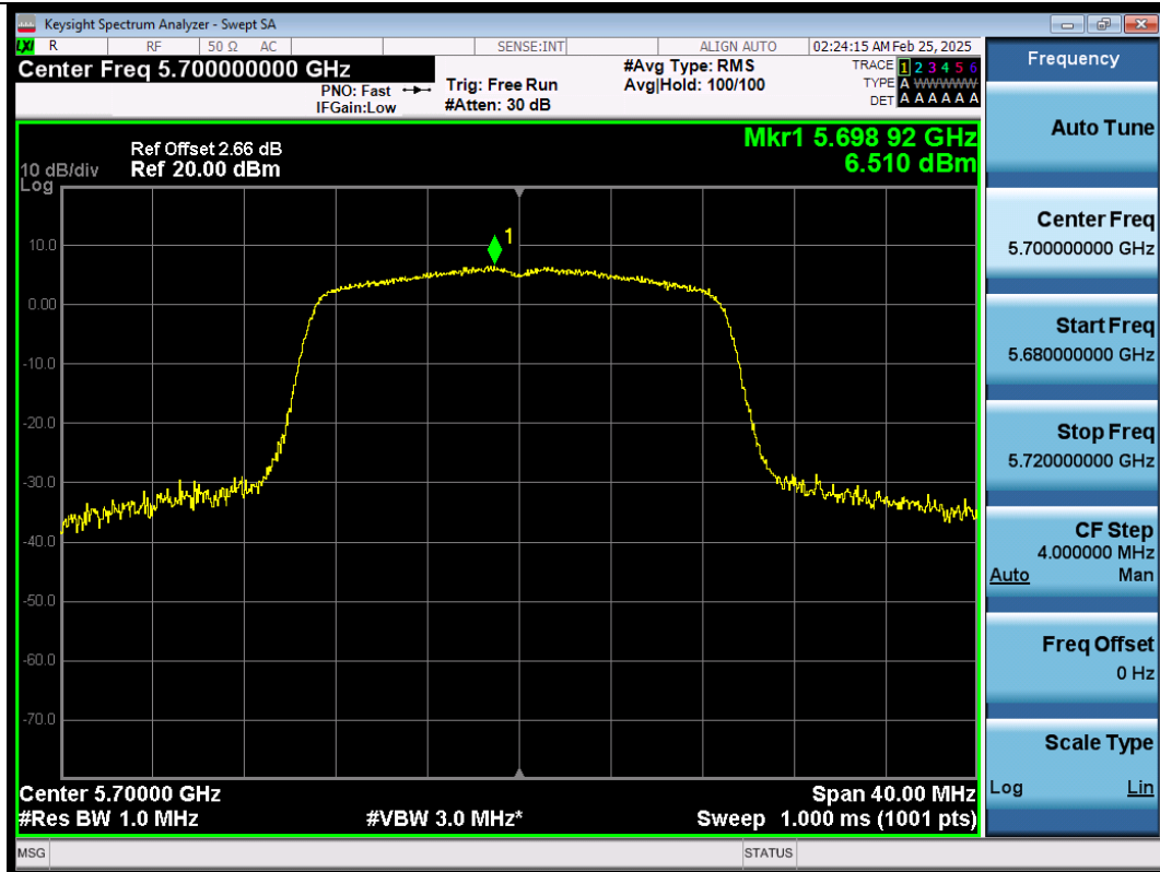
11AC20SISO-Ant1-5700-PASS
