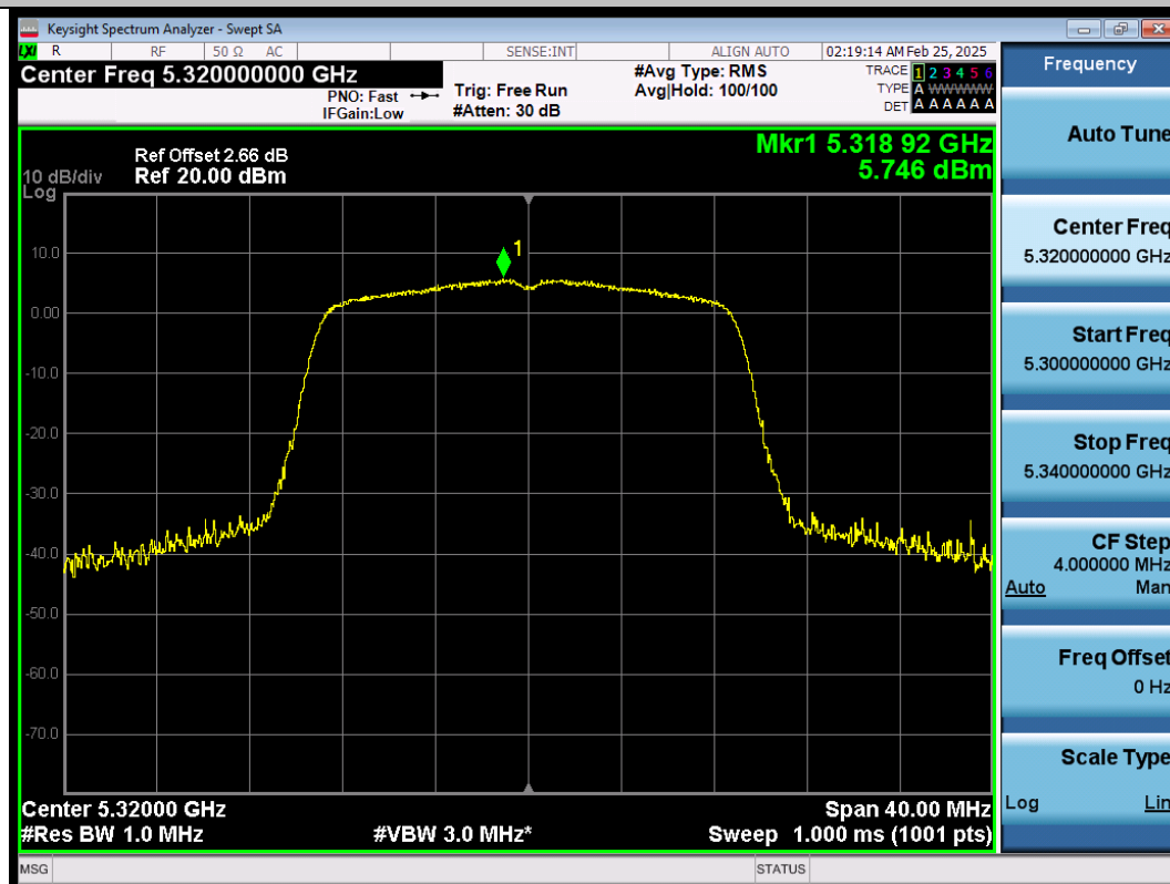
11AC20SISO-Ant1-5320-PASS
