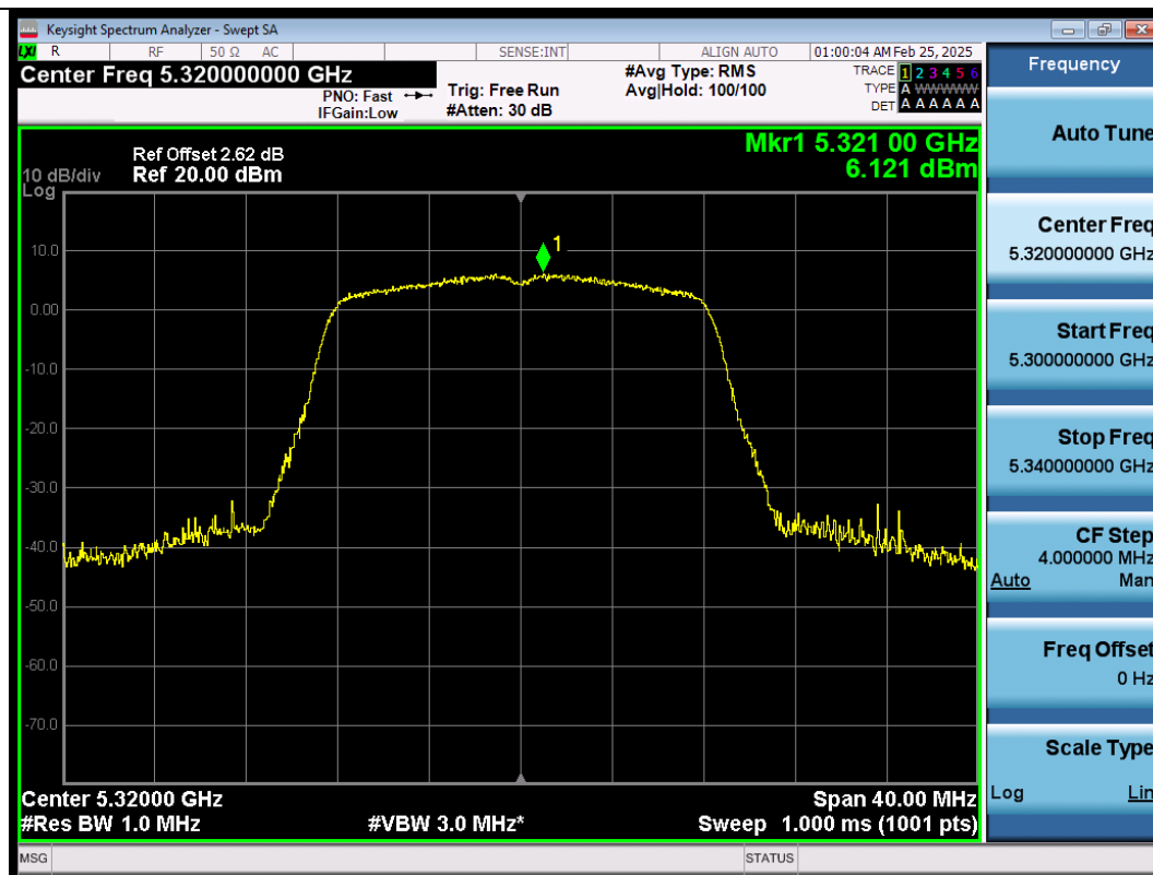
11A-Ant1-5320-PASS
