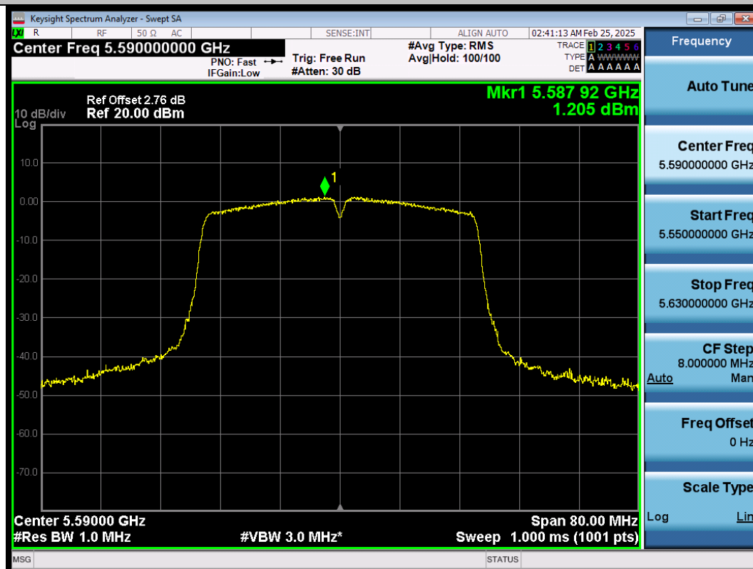
11AC40SISO-Ant1-5590-PASS
