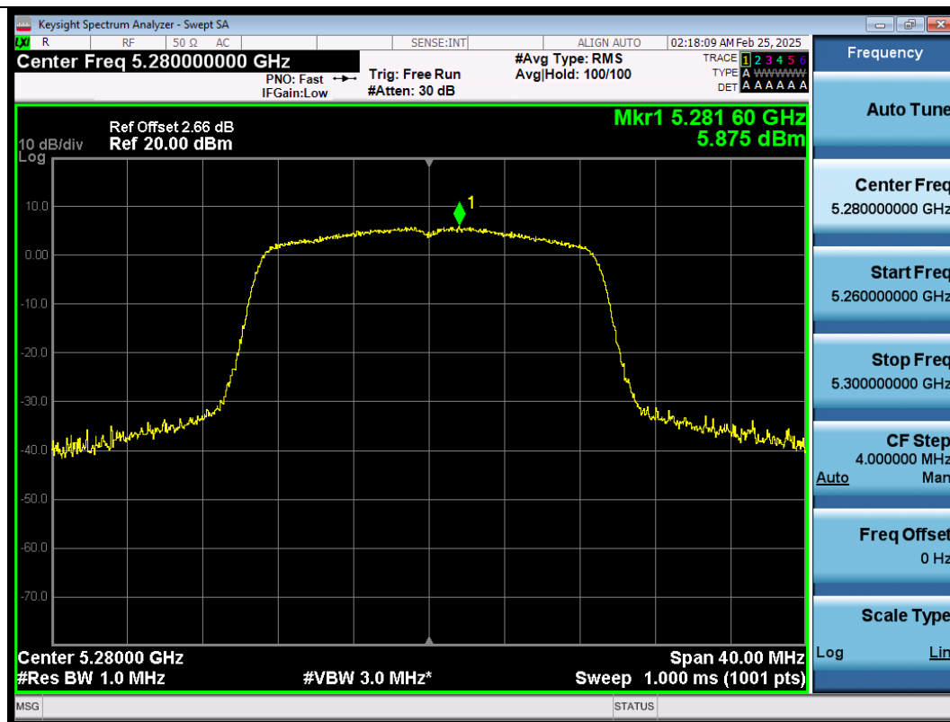
11AC20SISO-Ant1-5280-PASS
