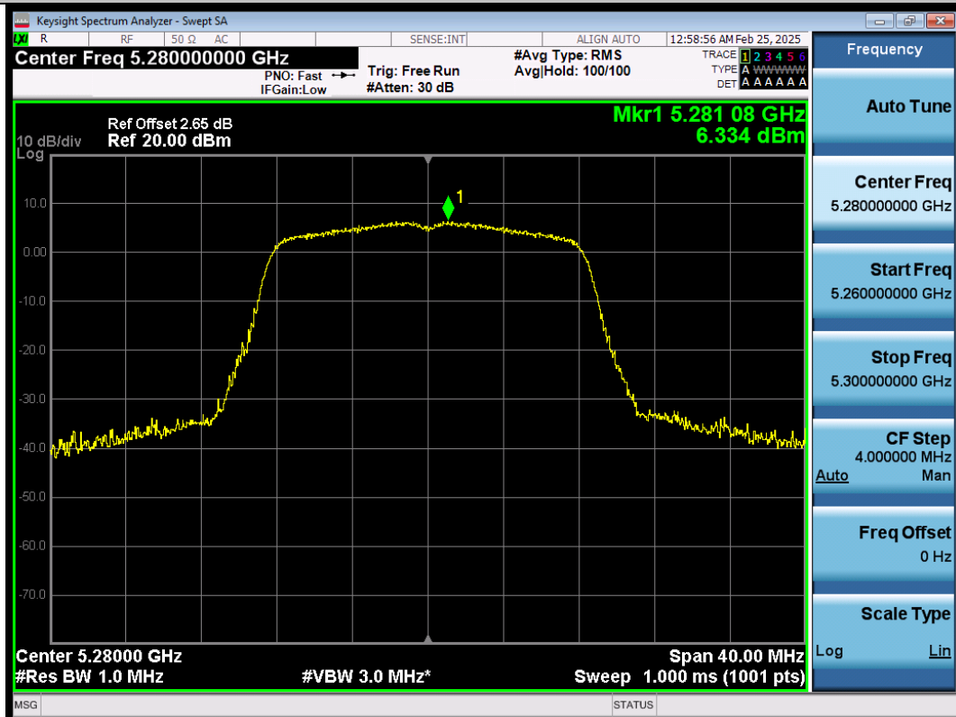
11A-Ant1-5280-PASS
