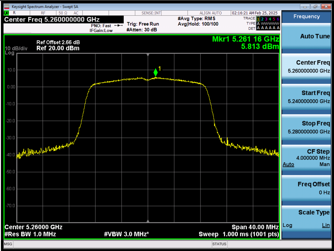
11AC20SISO-Ant1-5260-PASS
