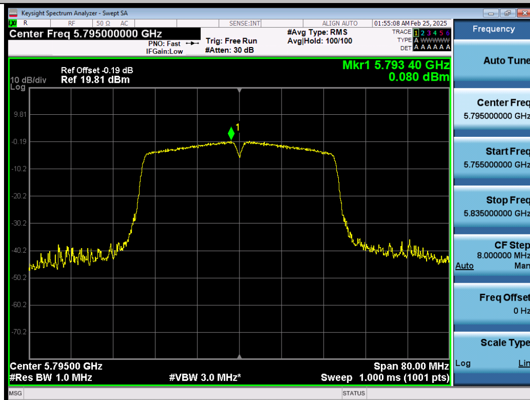
11N40SISO-Ant1-5795-PASS
