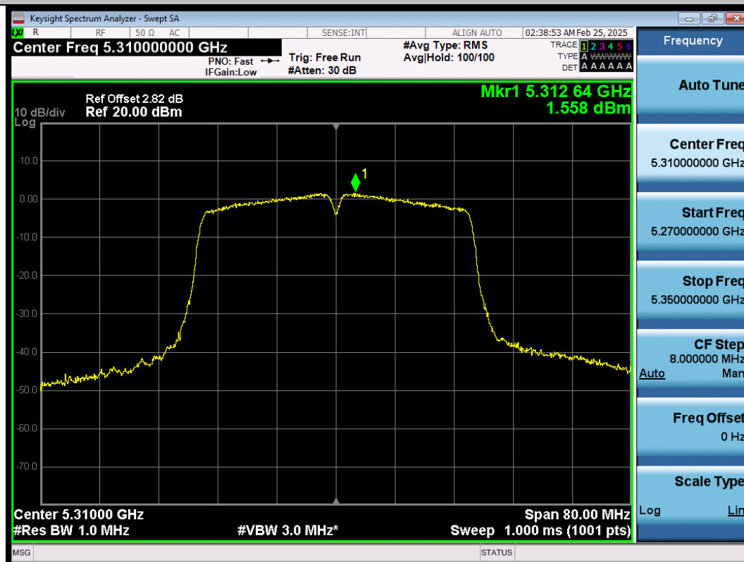
11AC40SISO-Ant1-5310-PASS
