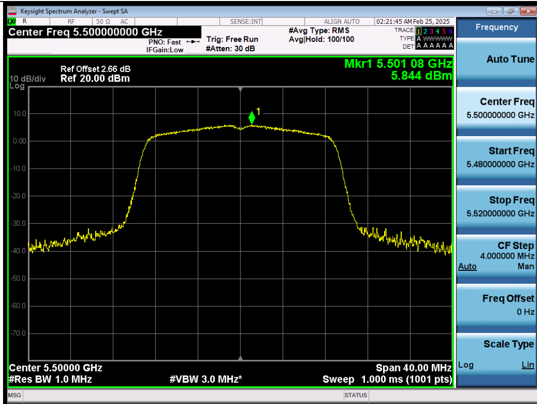
11AC20SISO-Ant1-5500-PASS
