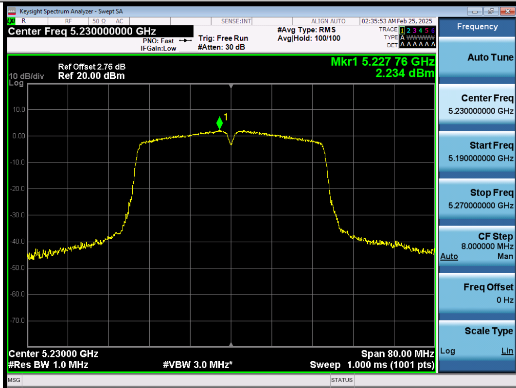
11AC40SISO-Ant1-5230-PASS
