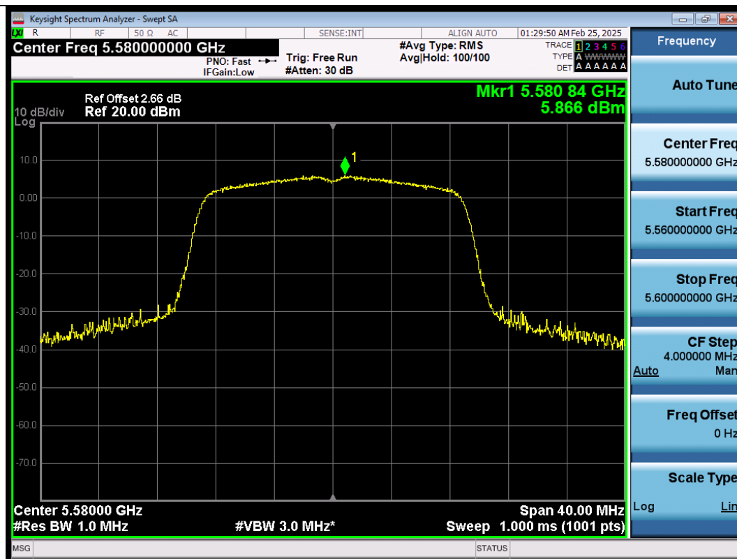
11N20SISO-Ant1-5580-PASS
