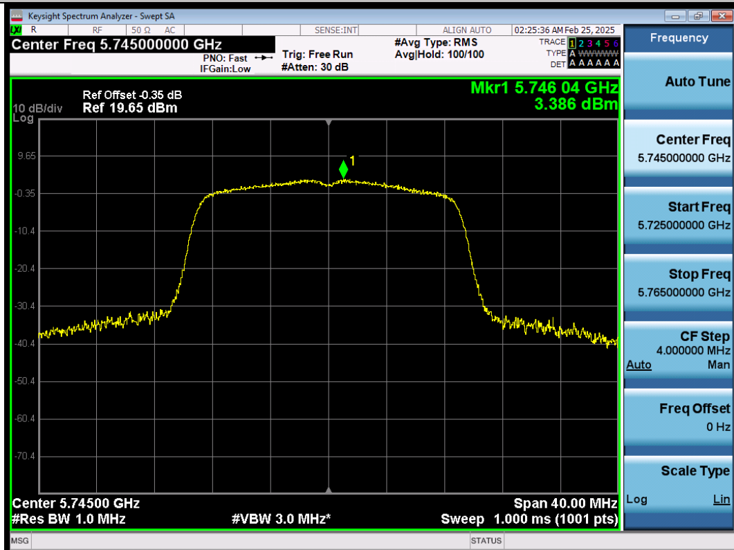
11AC20SISO-Ant1-5745-PASS
