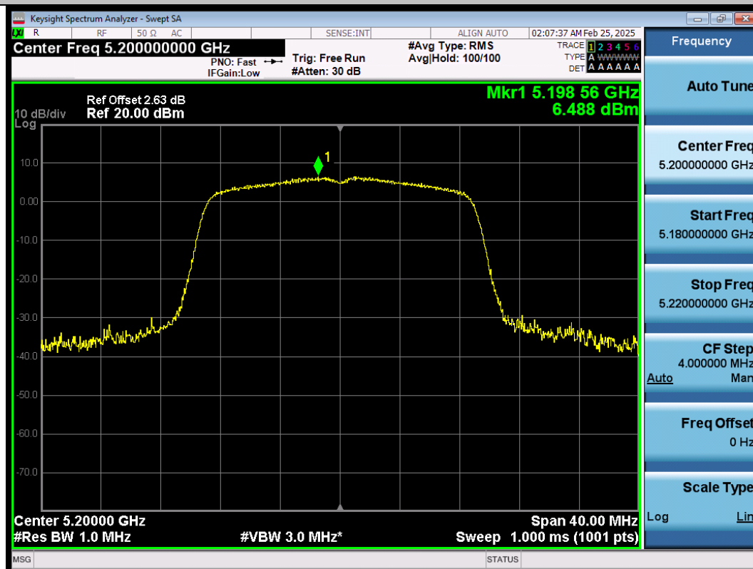
11AC20SISO-Ant1-5200-PASS
