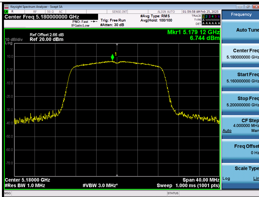
11AC20SISO-Ant1-5180-PASS
