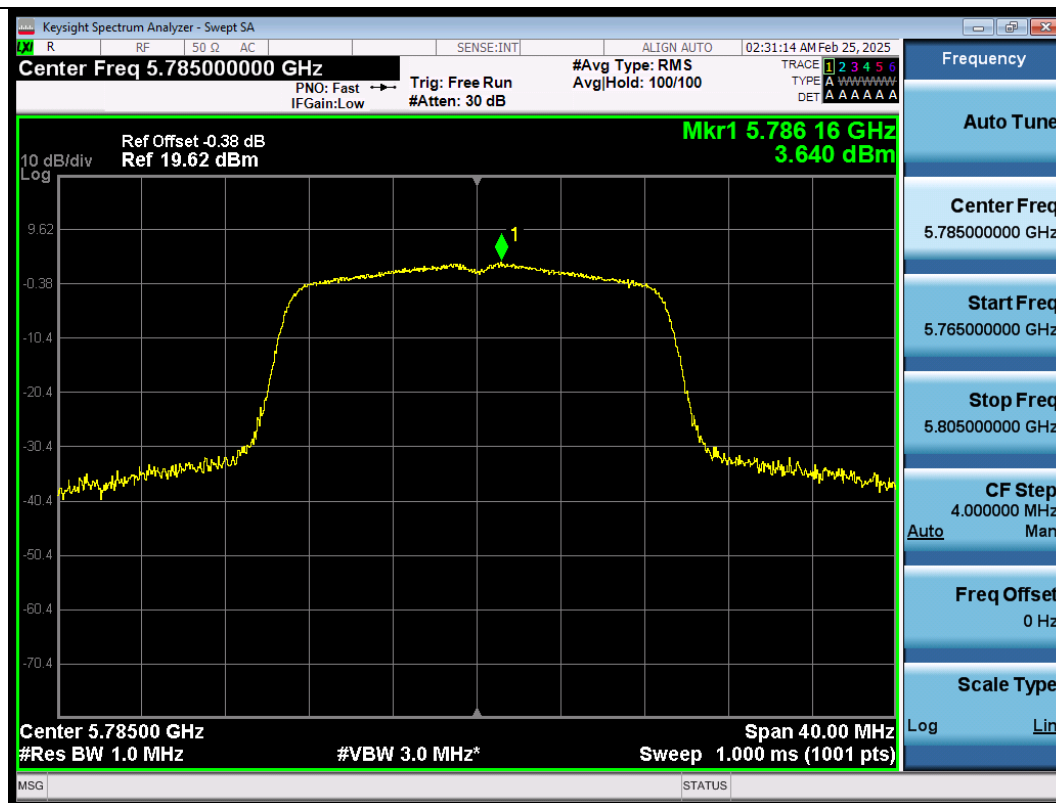
11AC20SISO-Ant1-5785-PASS
