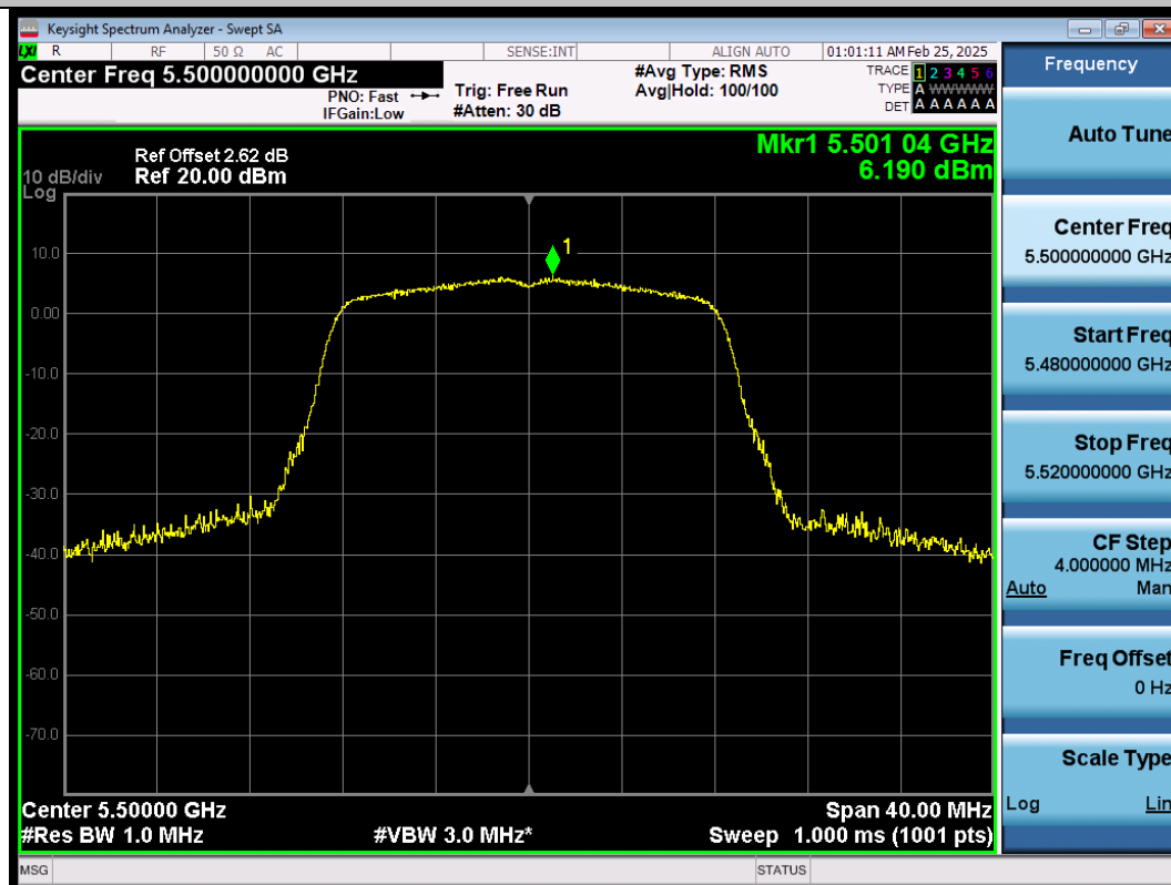
11A-Ant1-5500-PASS
