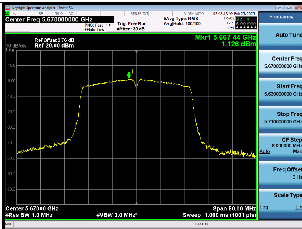
11AC40SISO-Ant1-5670-PASS
