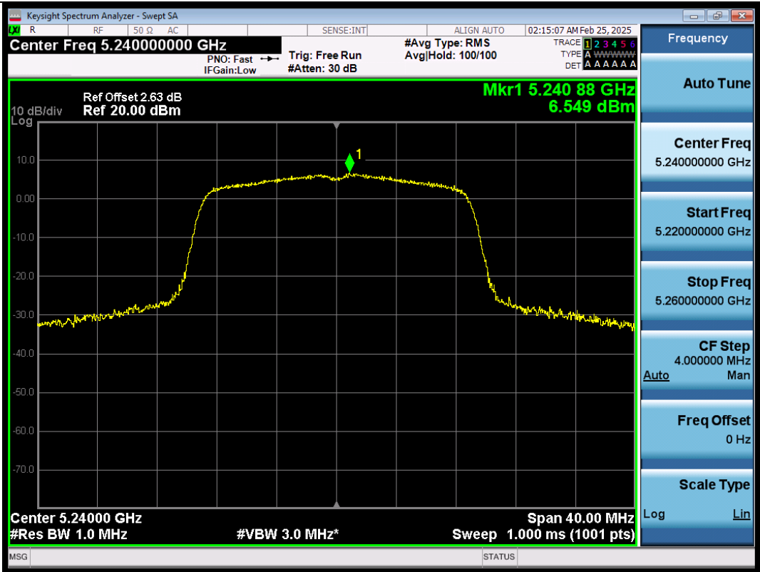
11AC20SISO-Ant1-5240-PASS
