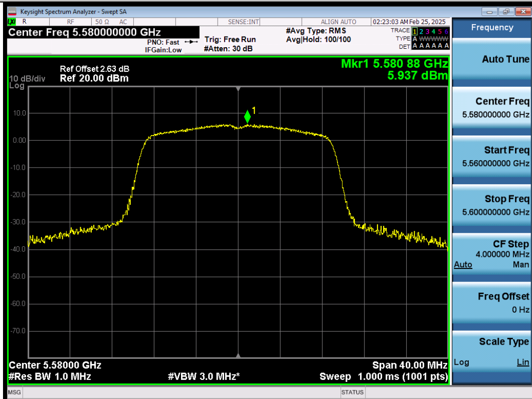
11AC20SISO-Ant1-5580-PASS
