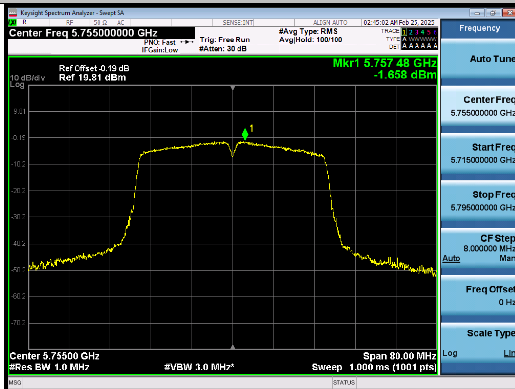
11AC40SISO-Ant1-5755-PASS
