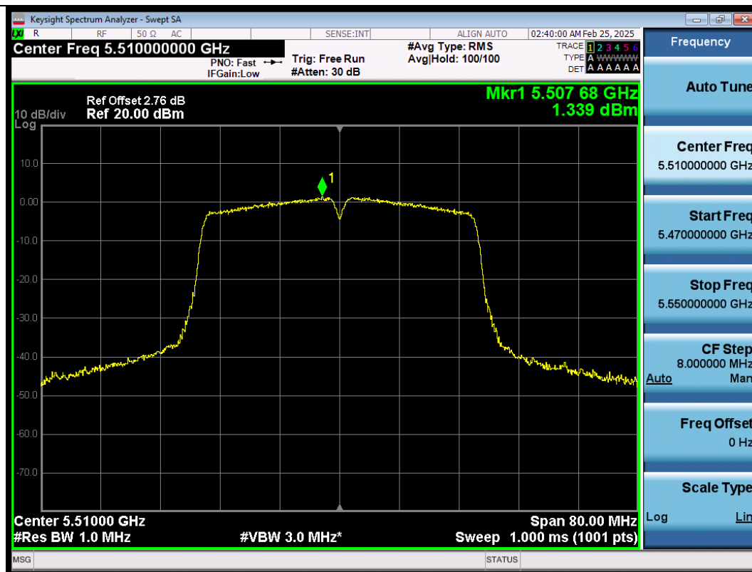
11AC40SISO-Ant1-5510-PASS
