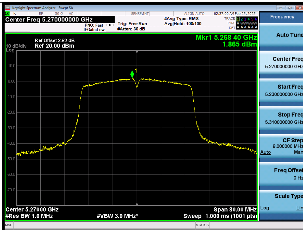
11AC40SISO-Ant1-5270-PASS
