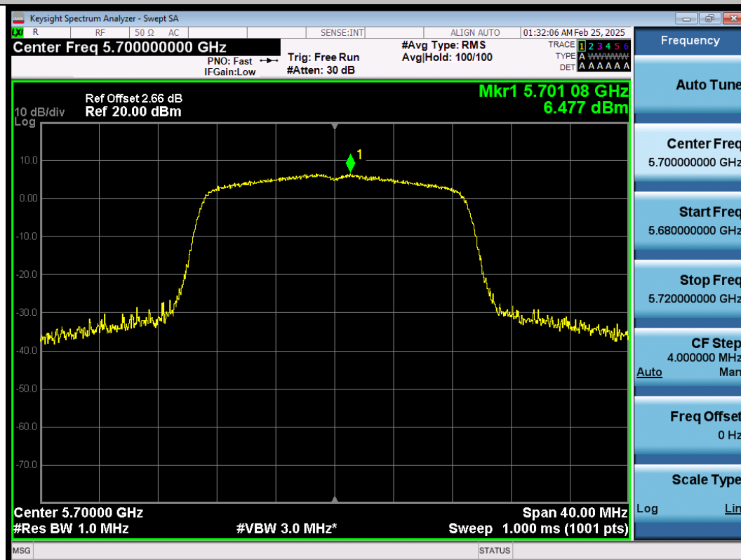
11N20SISO-Ant1-5700-PASS
