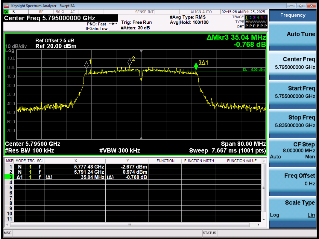
11AC40SISO-Ant1-5795-PASS
