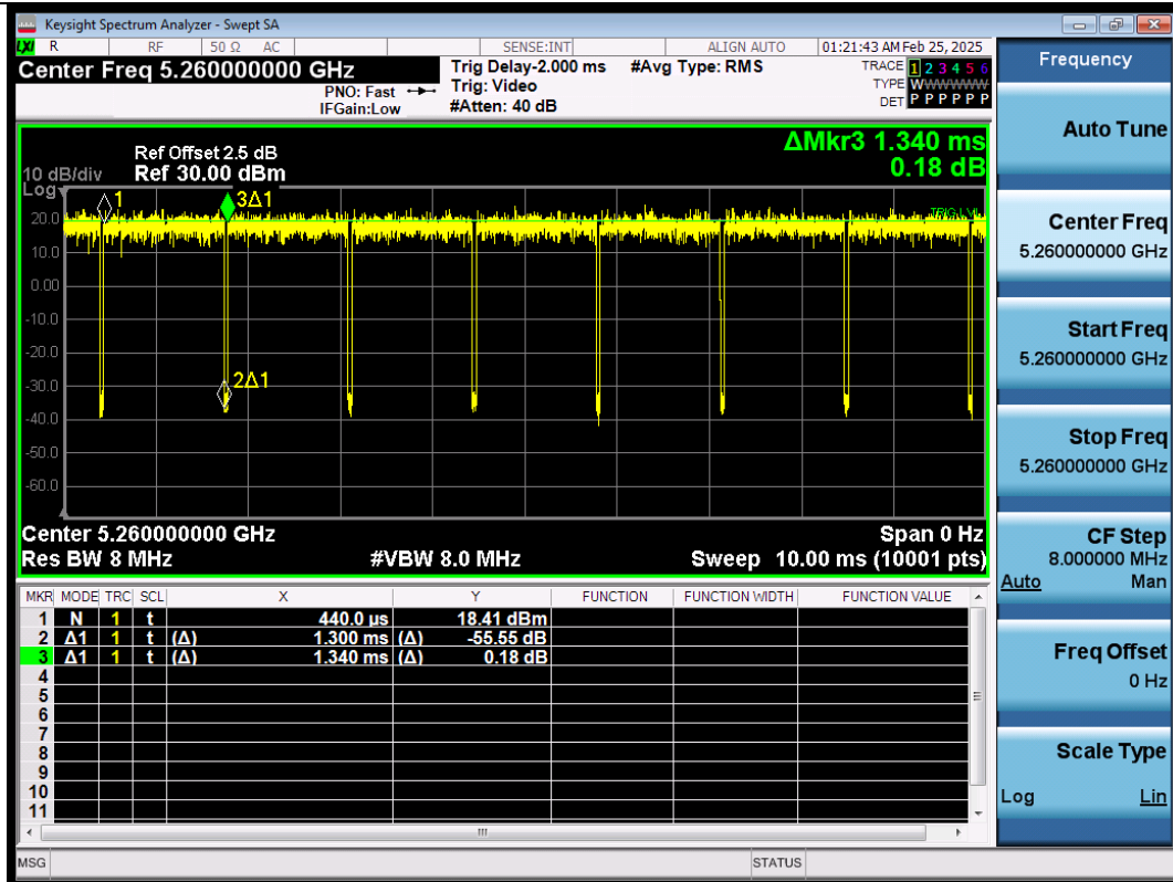
NTNV-11N20SISO-Ant1-5260
