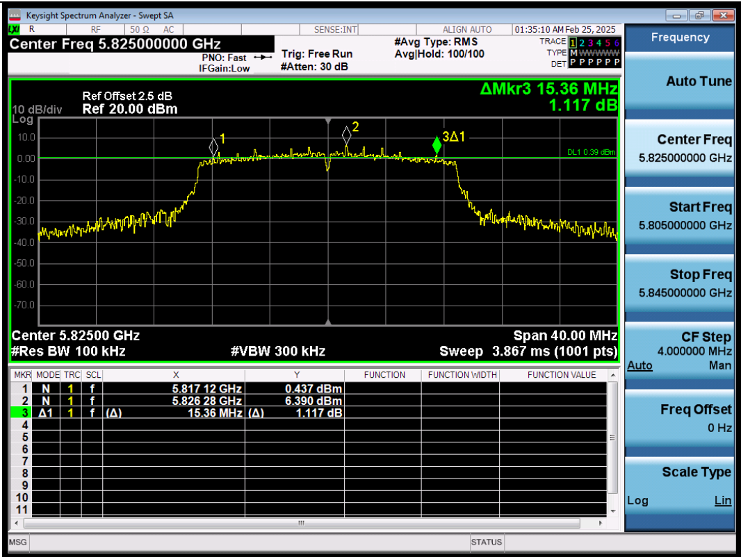
11N20SISO-Ant1-5825-PASS
