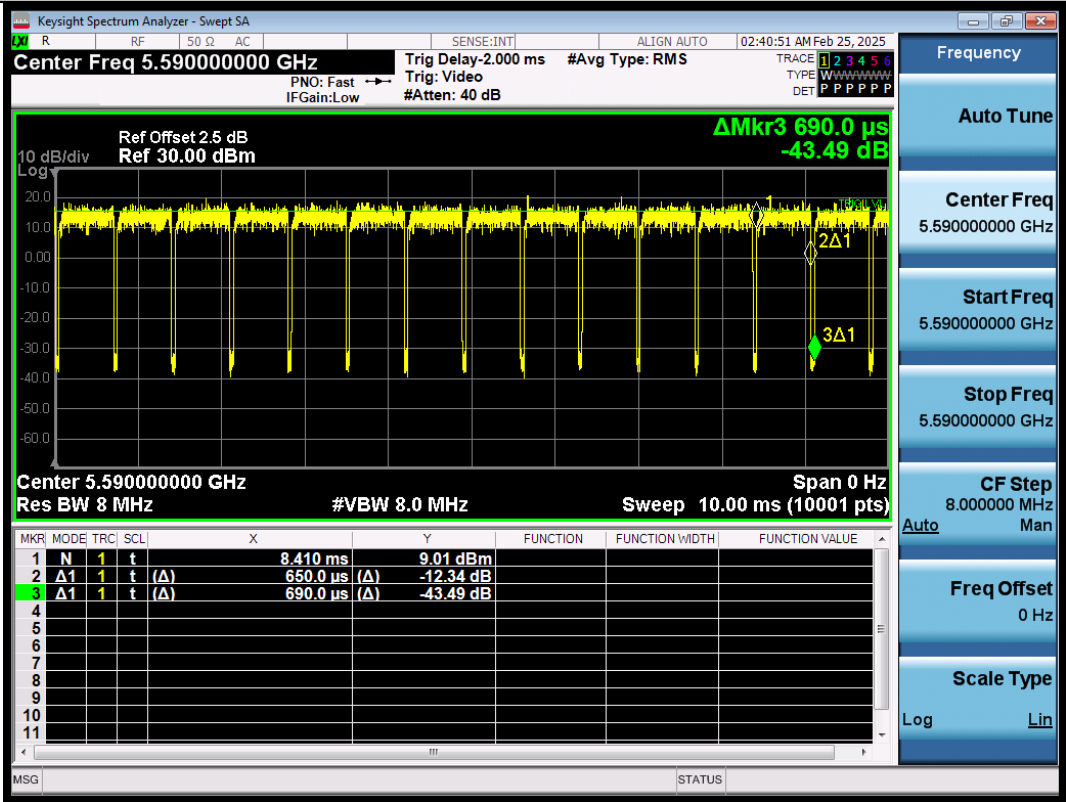
NTNV-11AC40SISO-Ant1-5590
