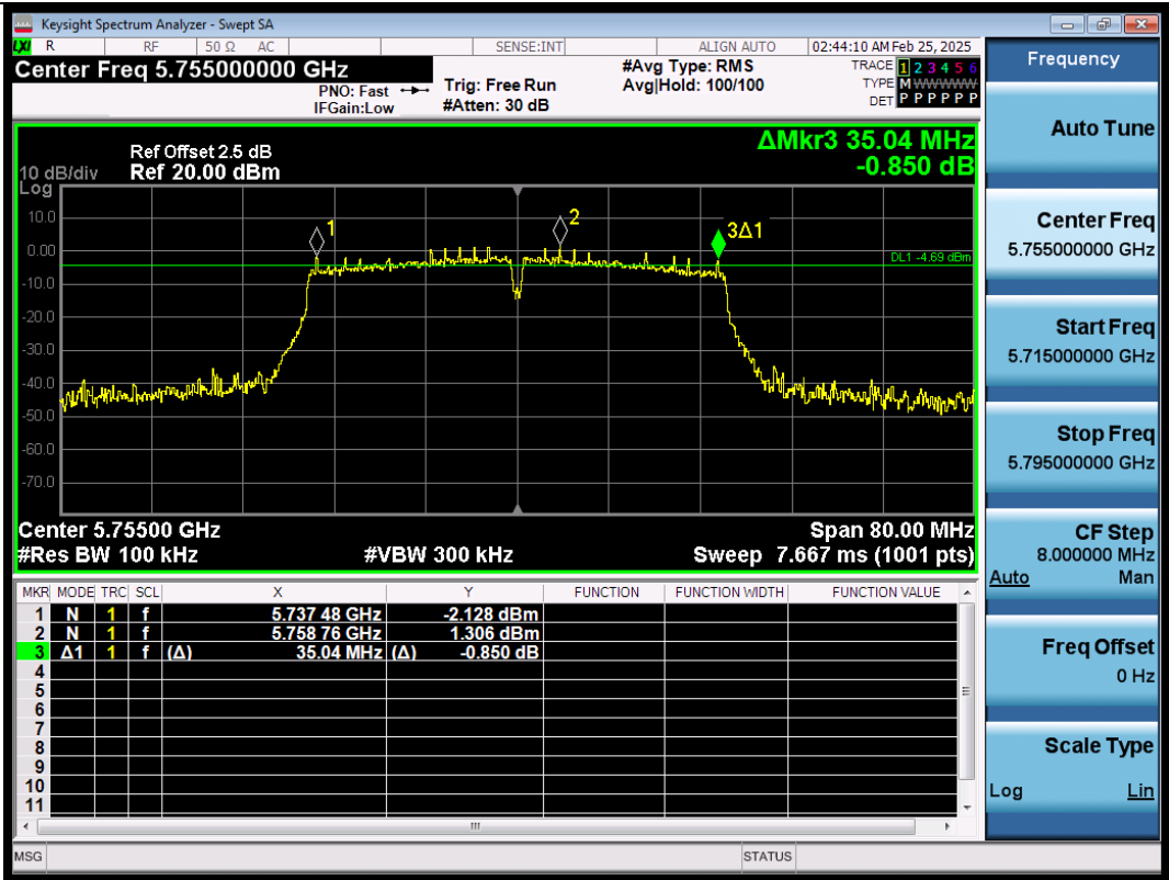
11AC40SISO-Ant1-5755-PASS
