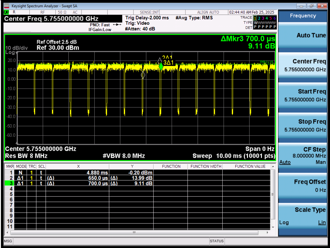
NTNV-11AC40SISO-Ant1-5755
