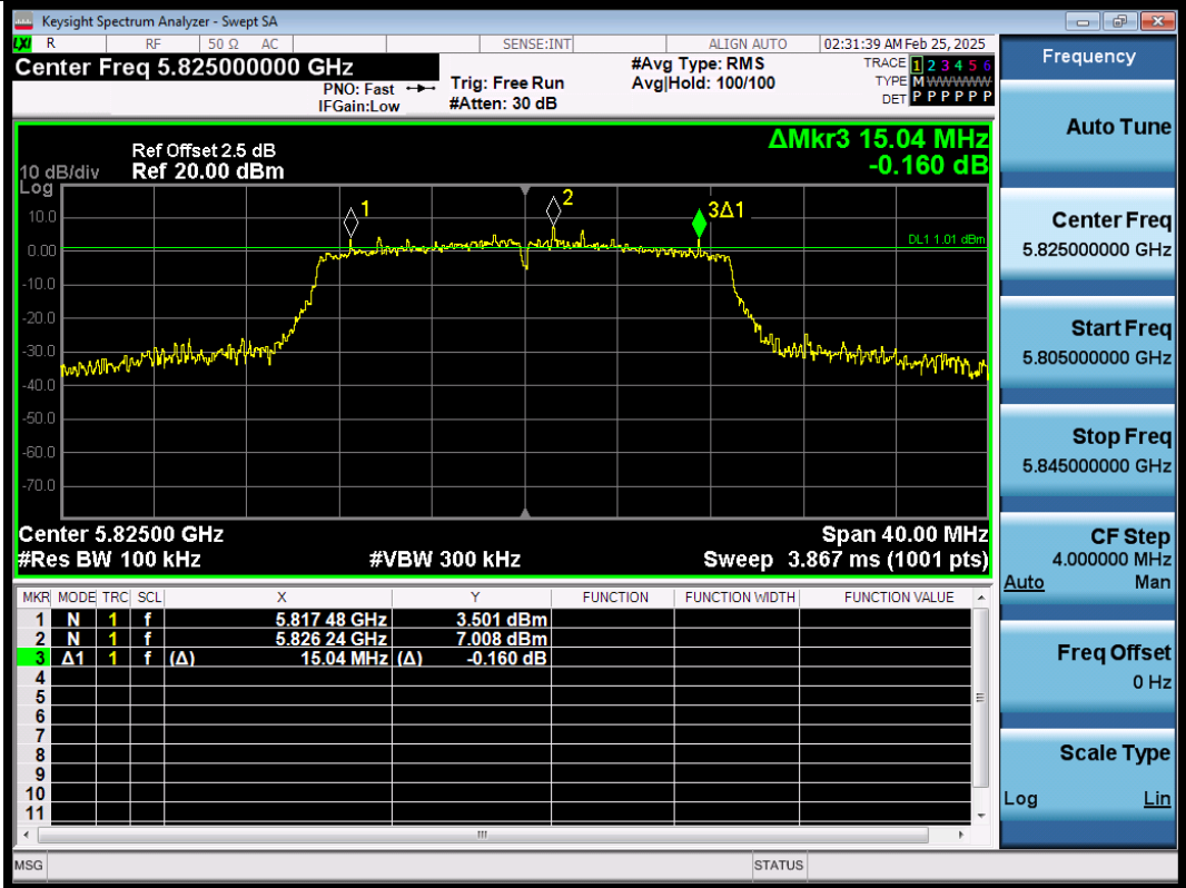
11AC20SISO-Ant1-5825-PASS
