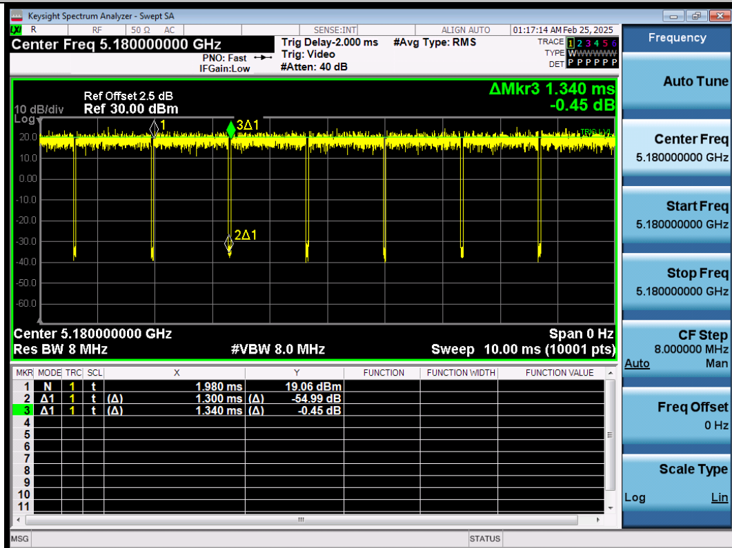
NTNV-11N20SISO-Ant1-5180
