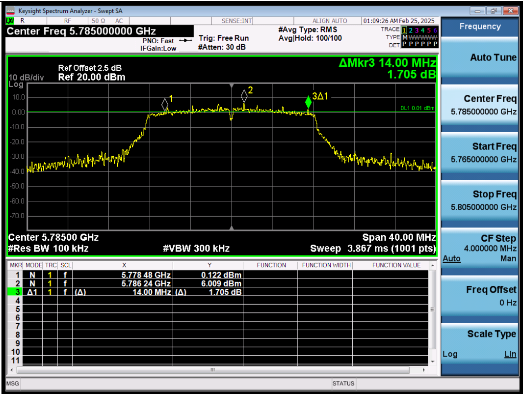
11A-Ant1-5785-PASS
