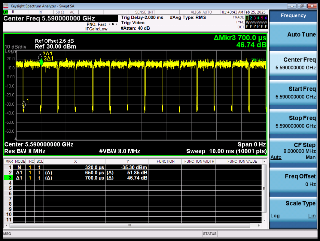
NTNV-11N40SISO-Ant1-5590
