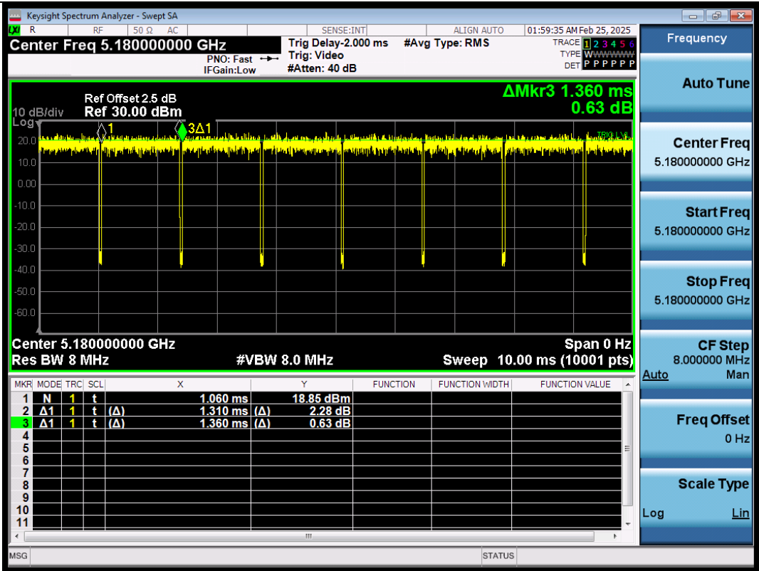
NTNV-11AC20SISO-Ant1-5180
