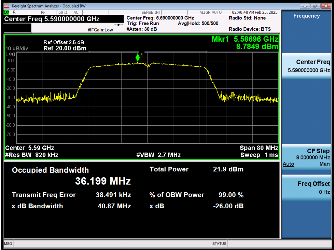
11AC40SISO-Ant1-5590
