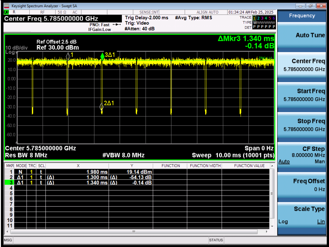
NTNV-11N20SISO-Ant1-5785
