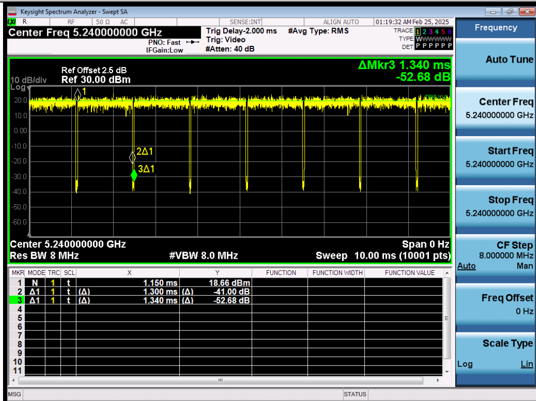
NTNV-11N20SISO-Ant1-5240
