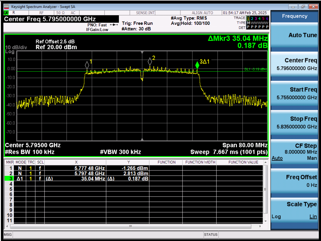
11N40SISO-Ant1-5795-PASS
