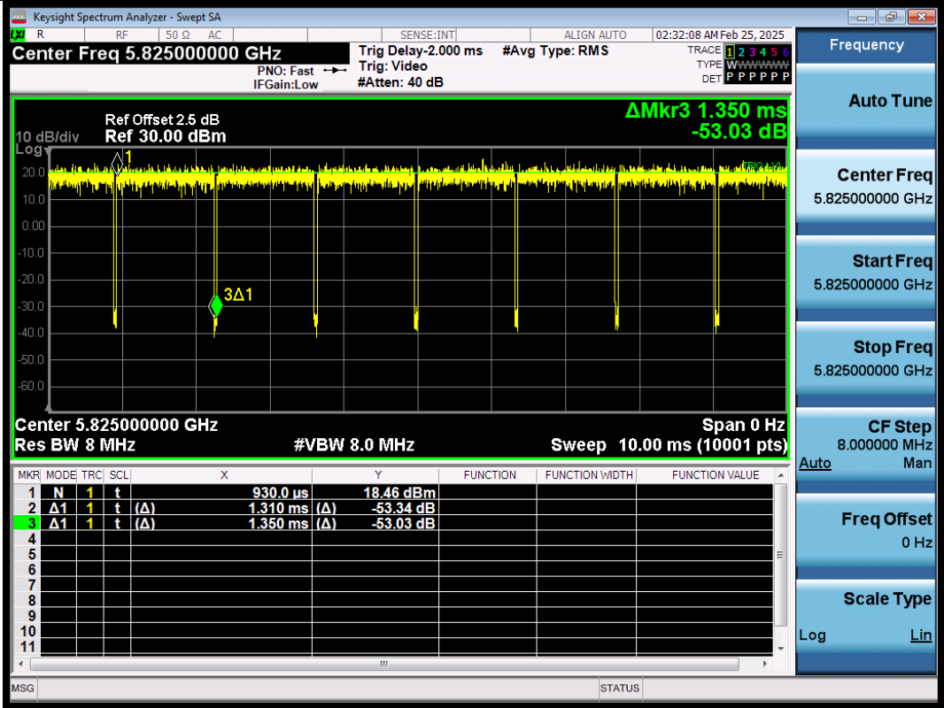
NTNV-11AC20SISO-Ant1-5825
