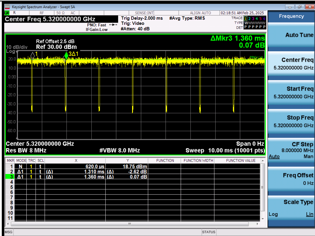
NTNV-11AC20SISO-Ant1-5320
