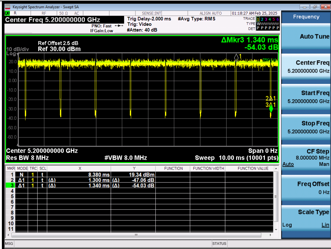
NTNV-11N20SISO-Ant1-5200
