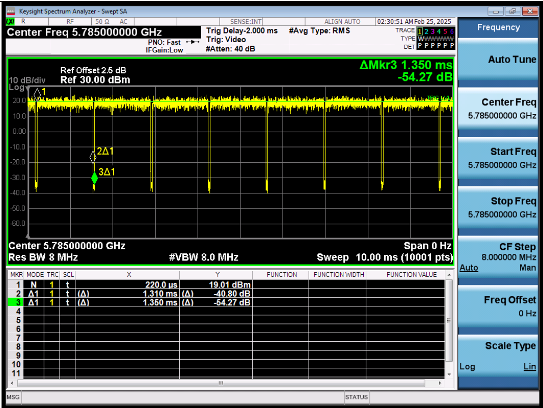
NTNV-11AC20SISO-Ant1-5785
