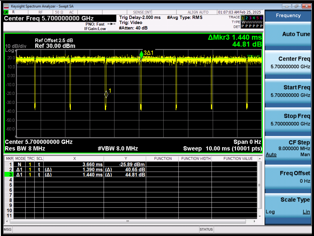
NTNV-11A-Ant1-5700
