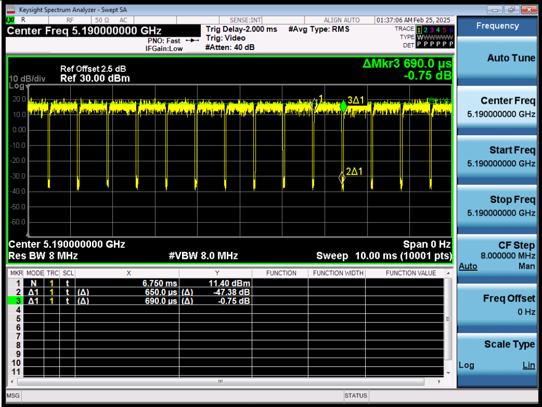
NTNV-11N40SISO-Ant1-5190
