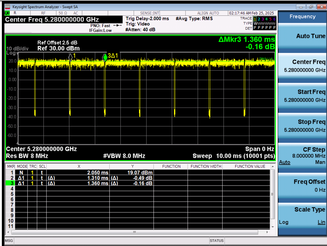
NTNV-11AC20SISO-Ant1-5280
