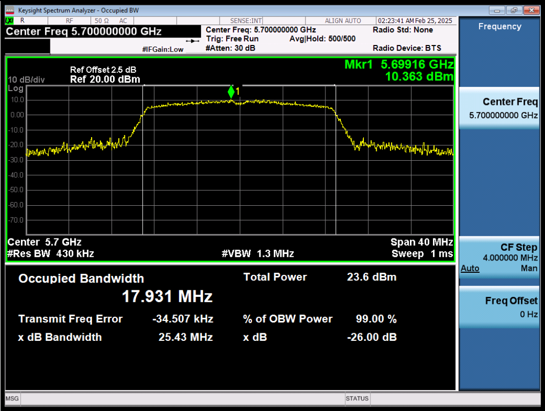
11AC20SISO-Ant1-5700
