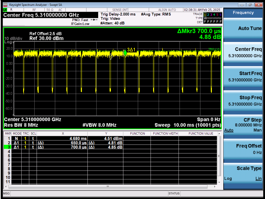
NTNV-11AC40SISO-Ant1-5310
