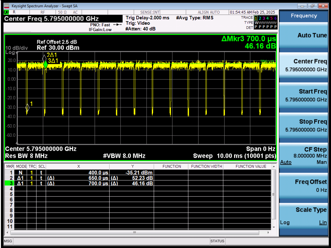
NTNV-11N40SISO-Ant1-5795
