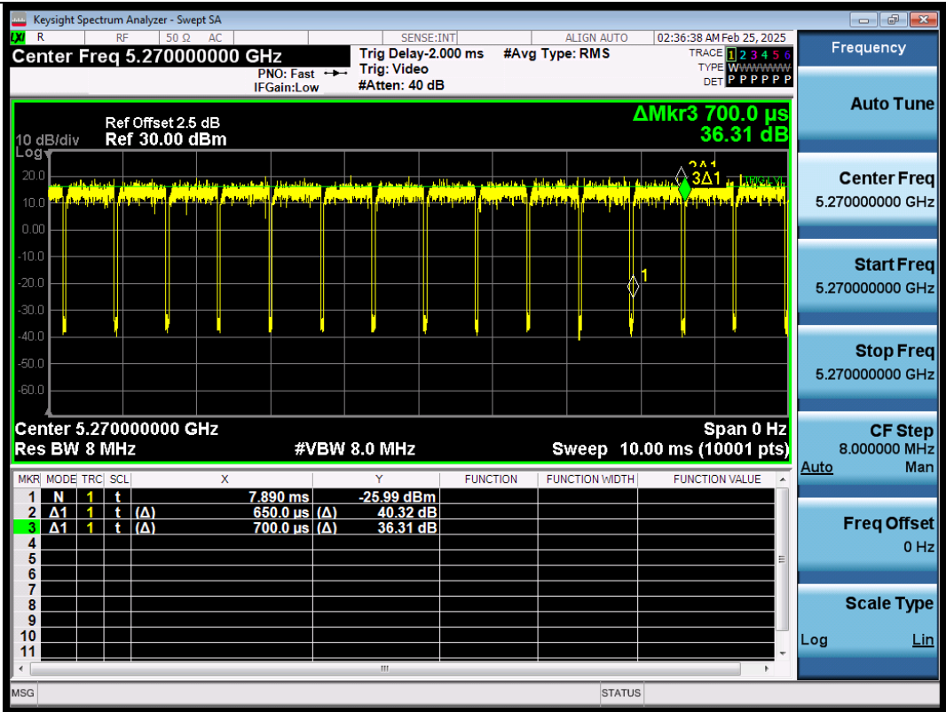
NTNV-11AC40SISO-Ant1-5270
