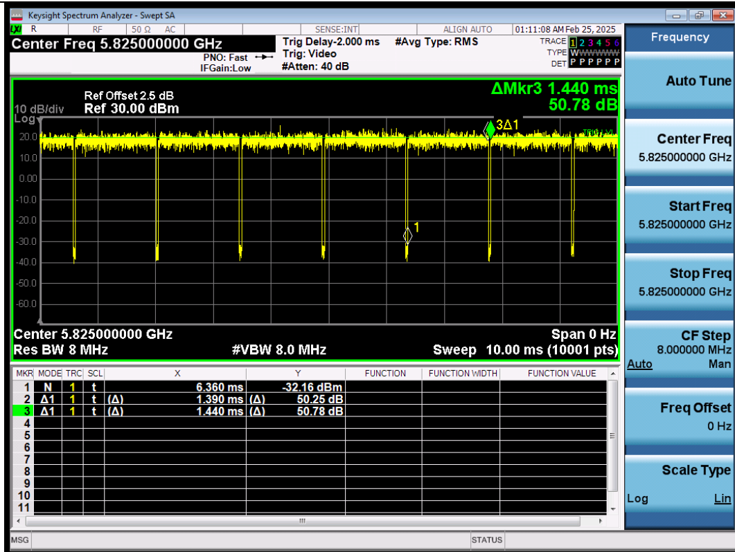
NTNV-11A-Ant1-5825
