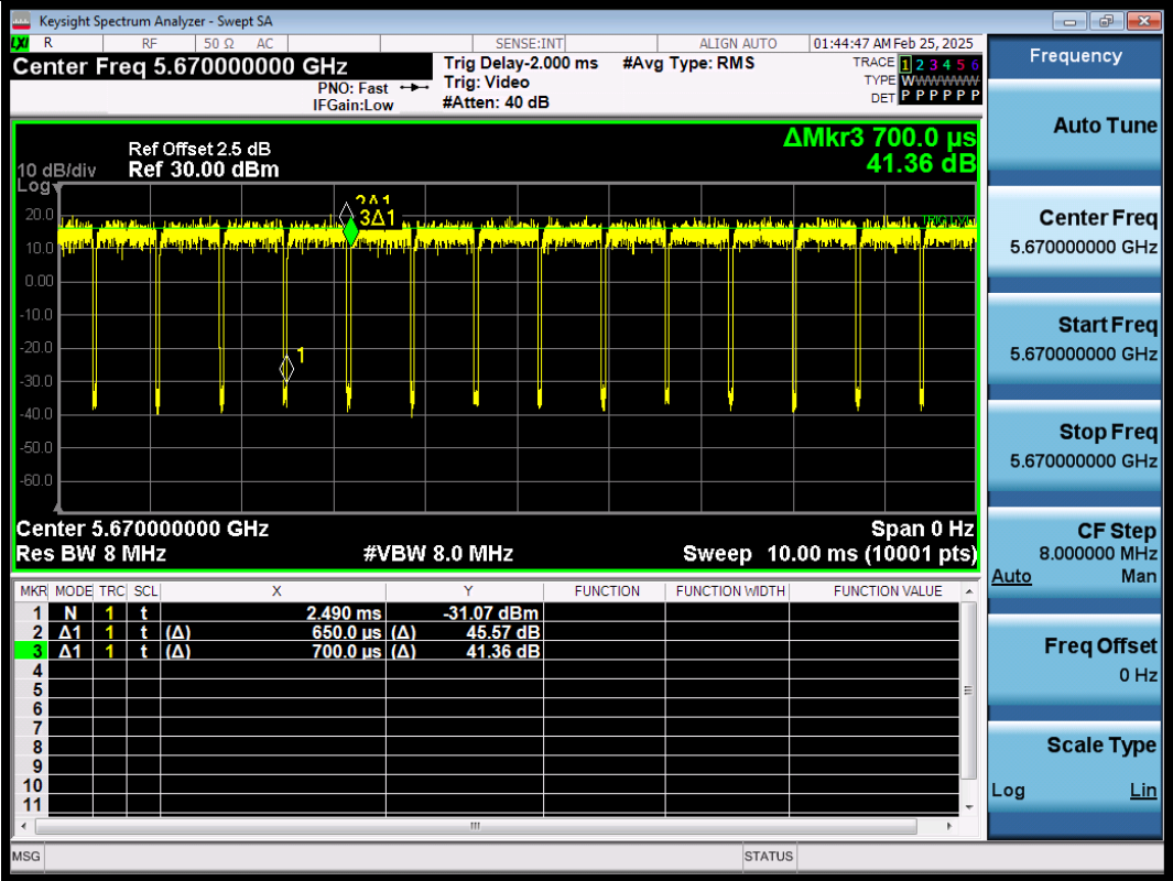
NTNV-11N40SISO-Ant1-5670
