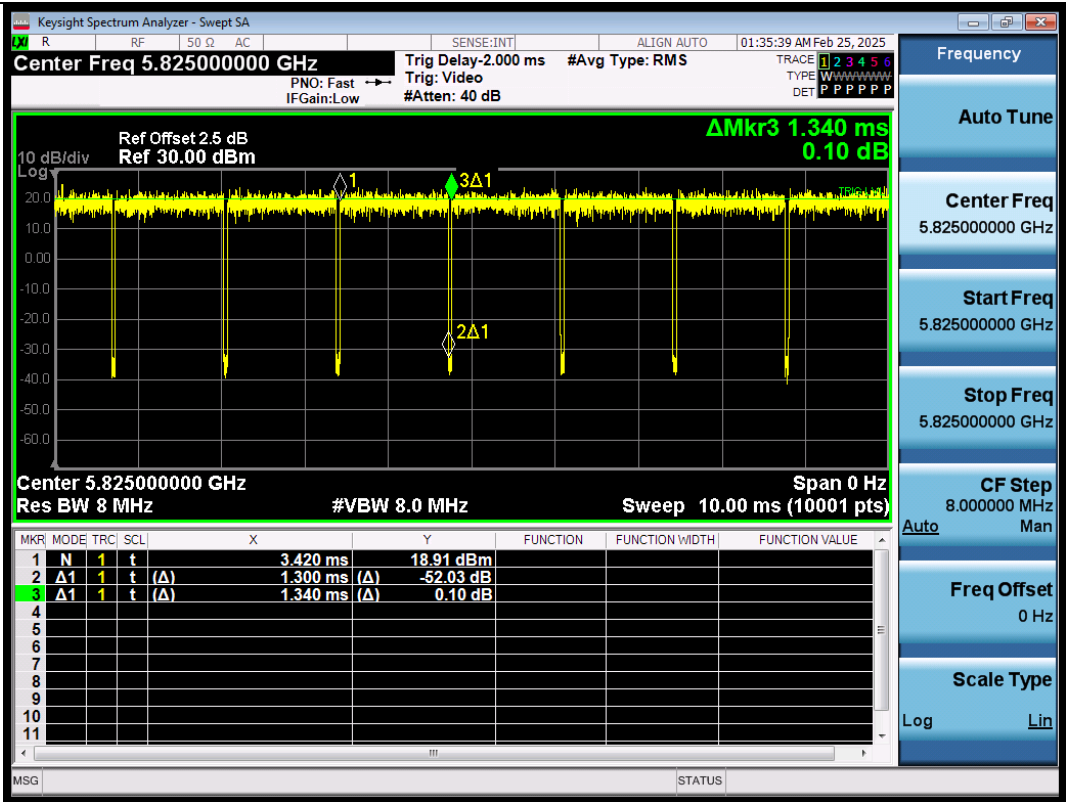
NTNV-11N20SISO-Ant1-5825
