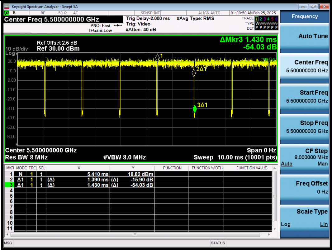
NTNV-11A-Ant1-5500
