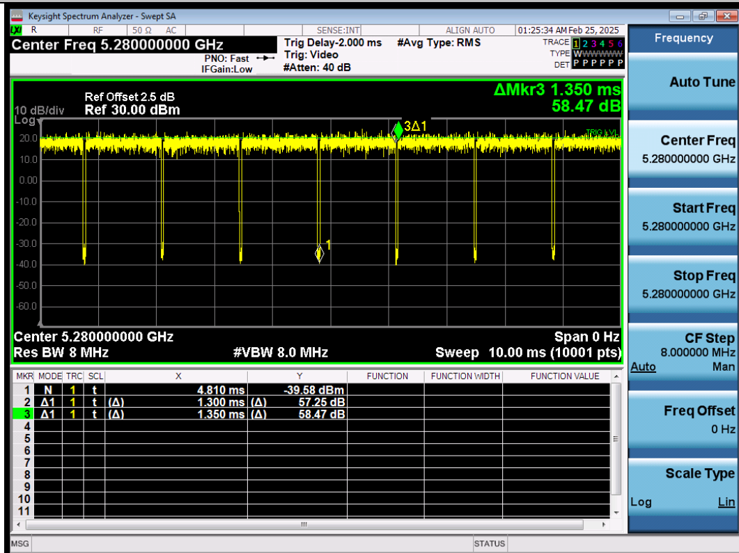
NTNV-11N20SISO-Ant1-5280
