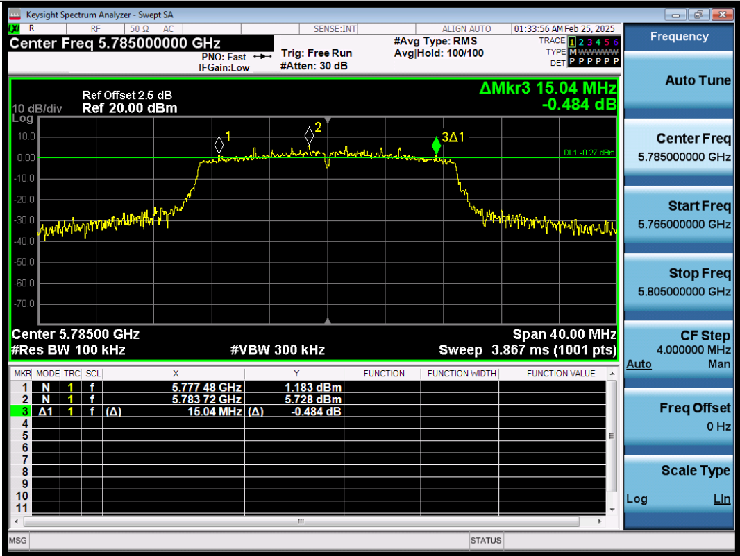
11N20SISO-Ant1-5785-PASS
