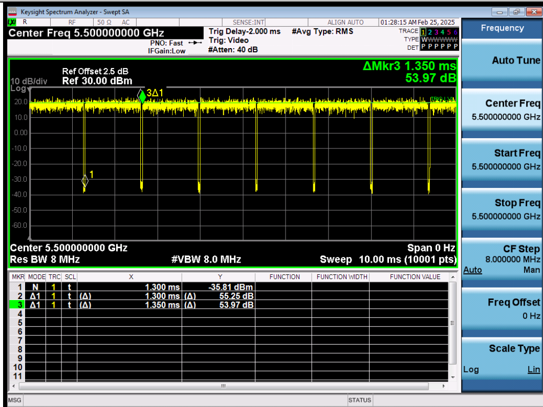
NTNV-11N20SISO-Ant1-5500
