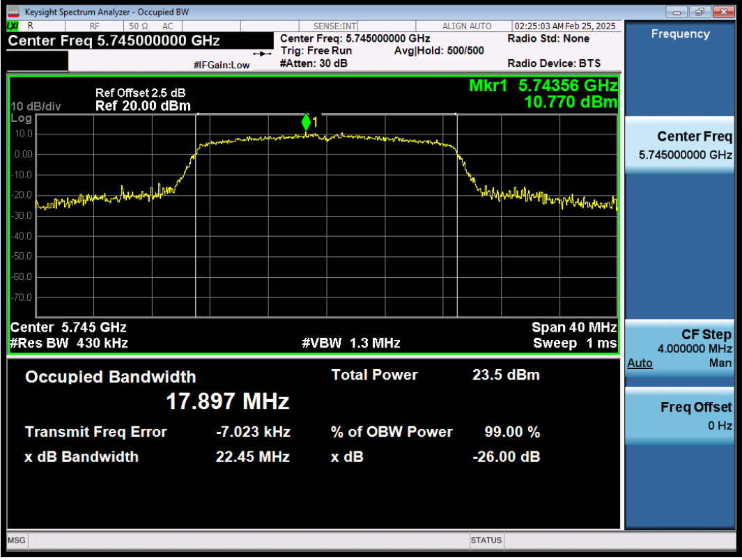
11AC20SISO-Ant1-5745
