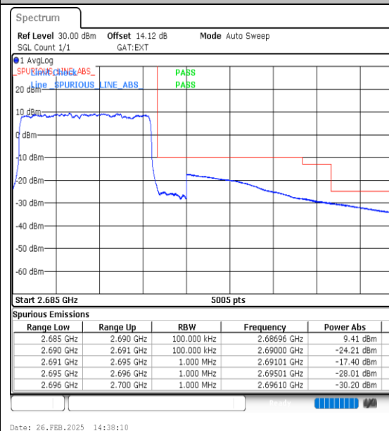
Band41_5MHz_16QAM_41565_25RB#0
