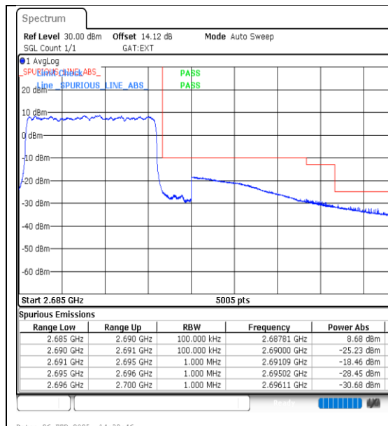
Band41_5MHz_64QAM_41565_25RB#0
