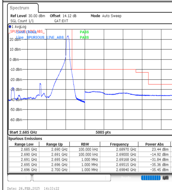
Band41_5MHz_16QAM_41565_1RB#24
