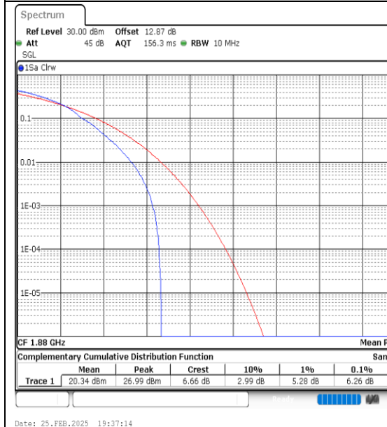
Band2-10MHz-64QAM-18900-1RB#0-PASS
