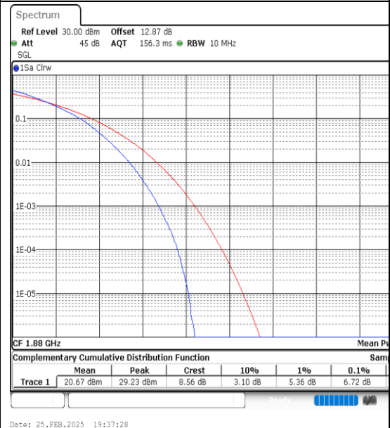
Band2-10MHz-64QAM-18900-50RB#0-PASS
