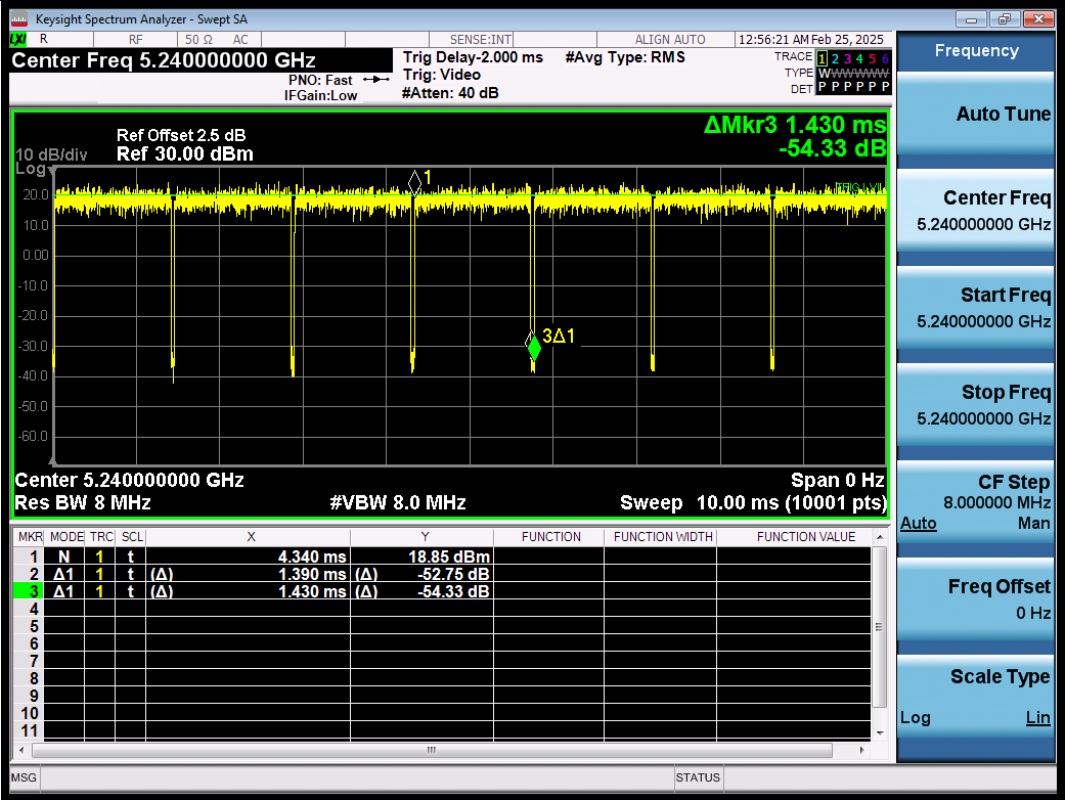
NTNV-11A-Ant1-5240
