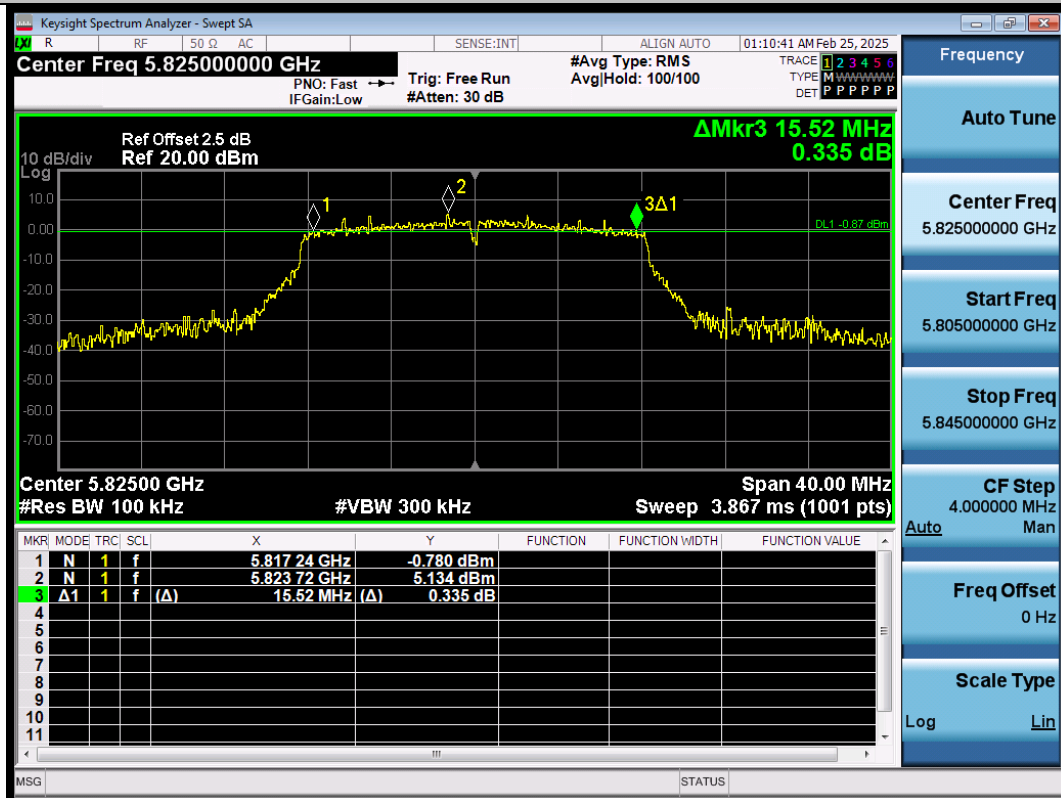
11A-Ant1-5825-PASS
