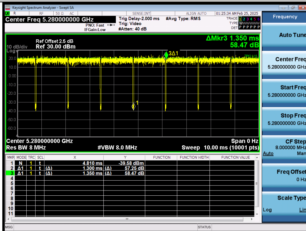
NTNV-11N20SISO-Ant1-5280
