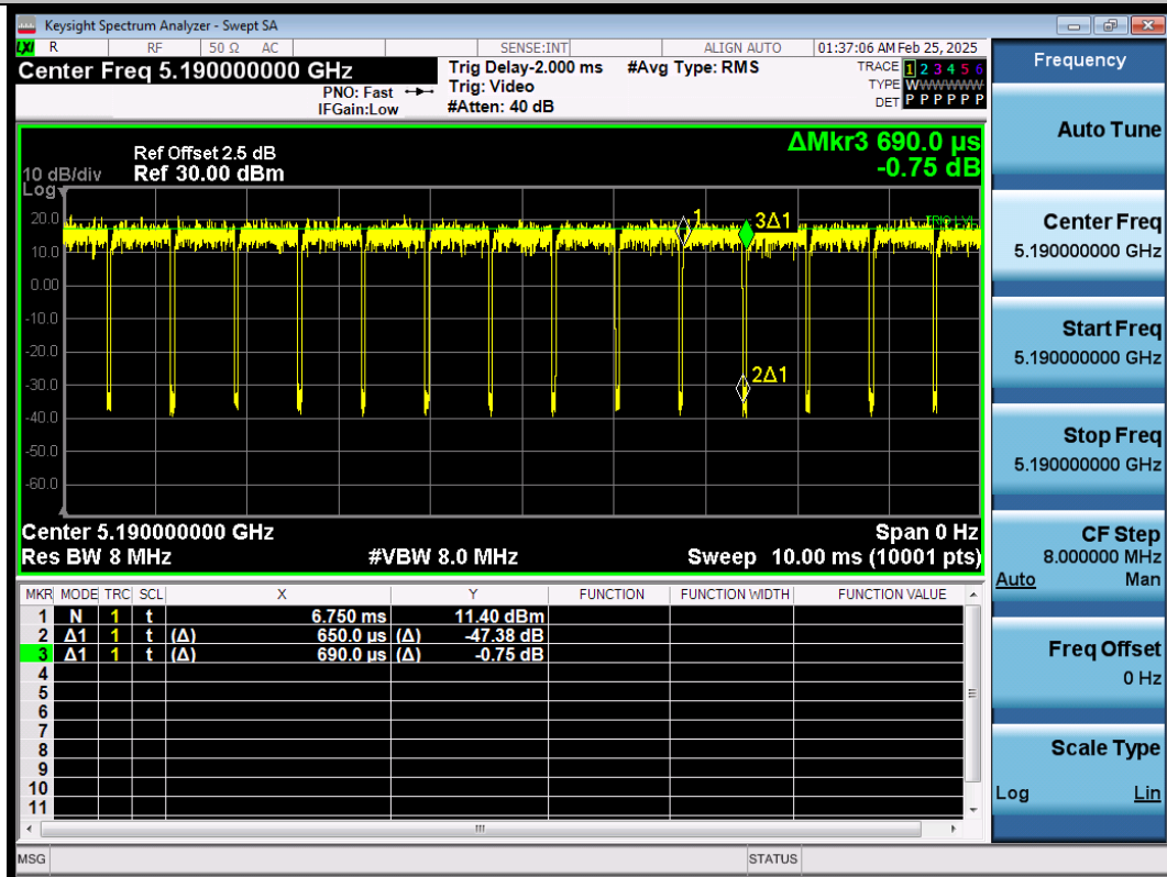
NTNV-11N40SISO-Ant1-5190
