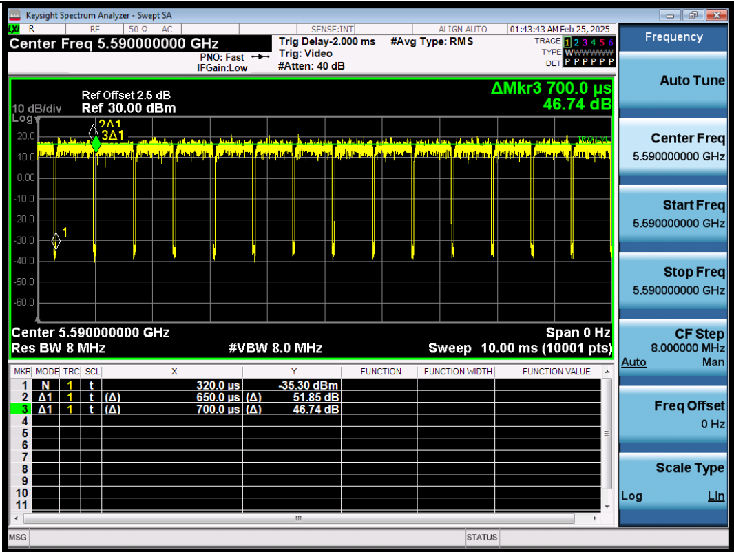
NTNV-11N40SISO-Ant1-5590
