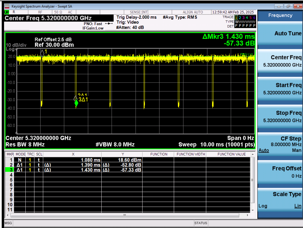
NTNV-11A-Ant1-5320
