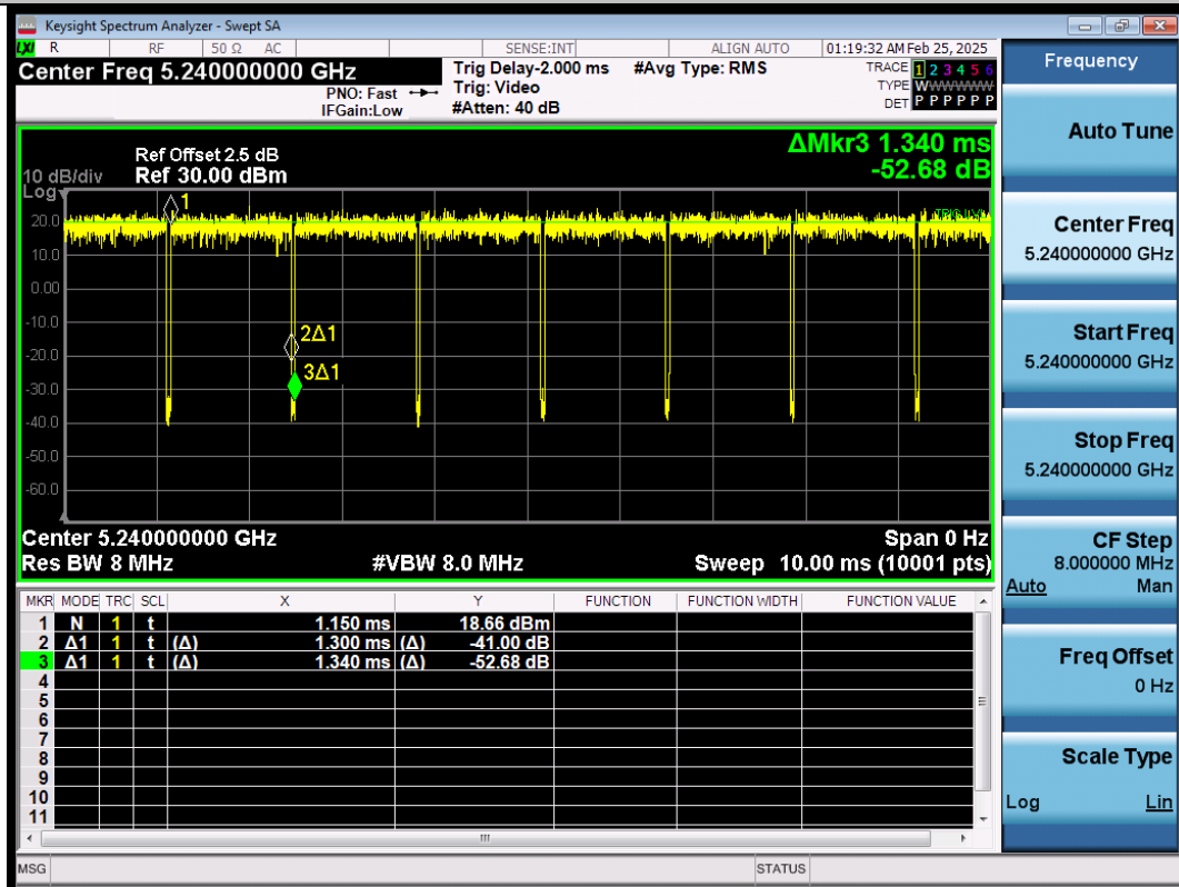
NTNV-11N20SISO-Ant1-5240
