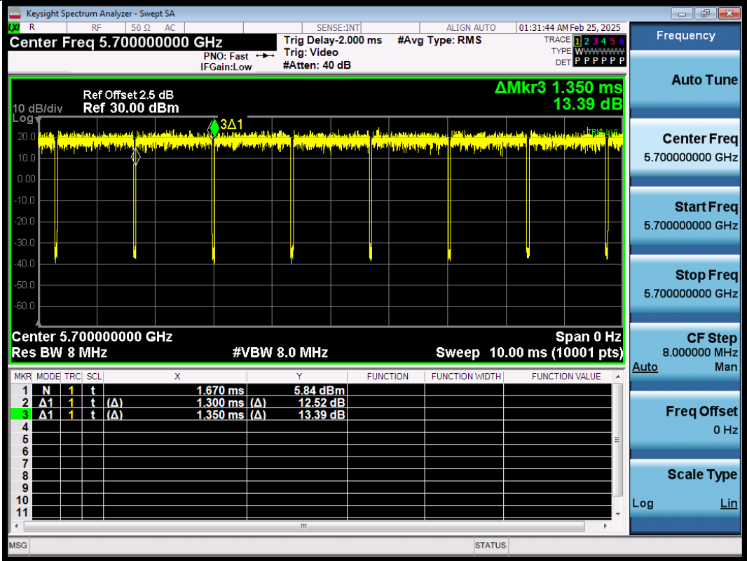
NTNV-11N20SISO-Ant1-5700
