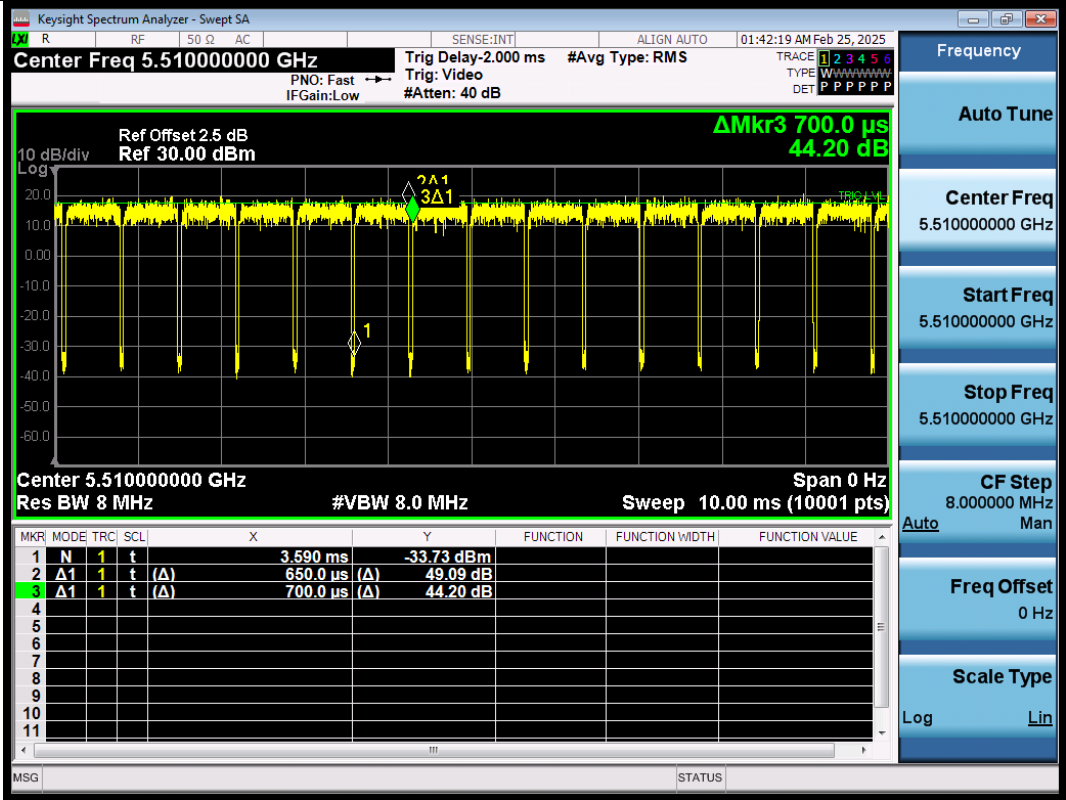
NTNV-11N40SISO-Ant1-5510
