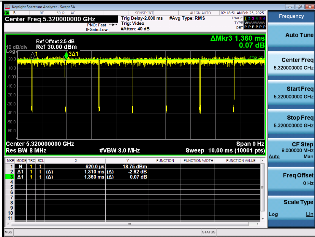
NTNV-11AC20SISO-Ant1-5320
