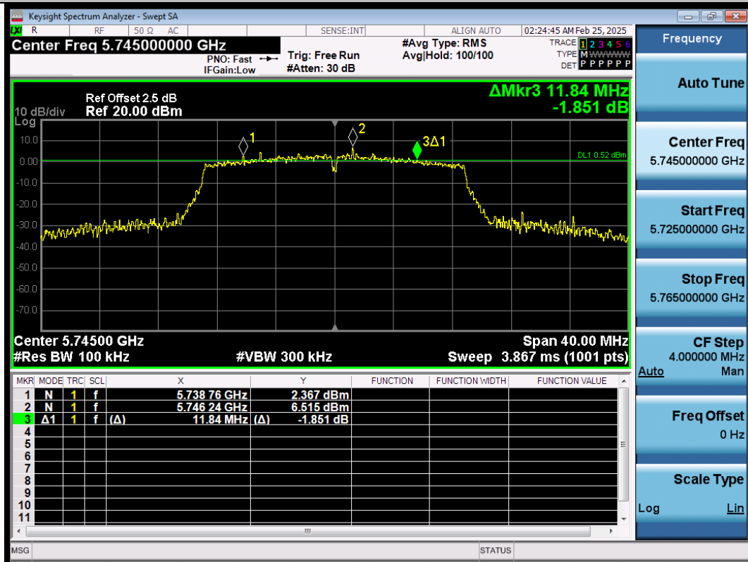
11AC20SISO-Ant1-5745-PASS
