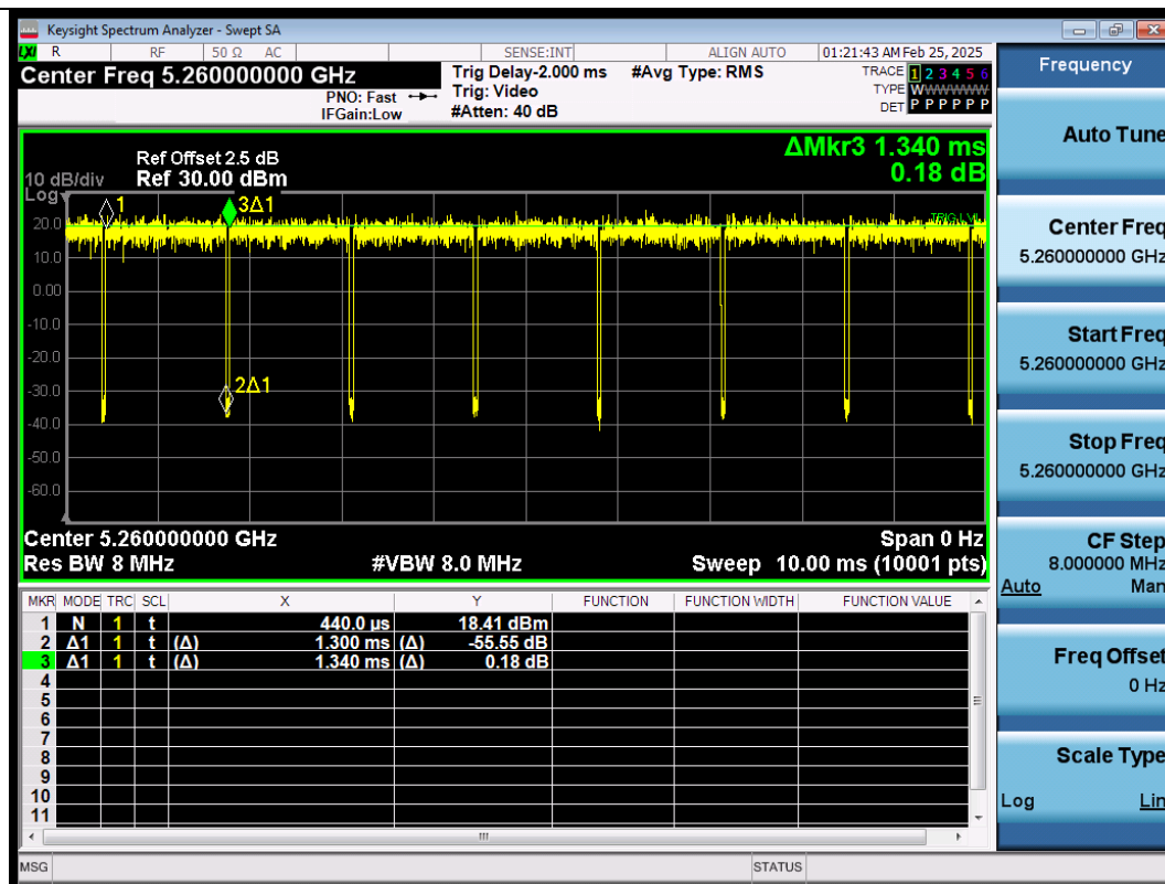
NTNV-11N20SISO-Ant1-5260
