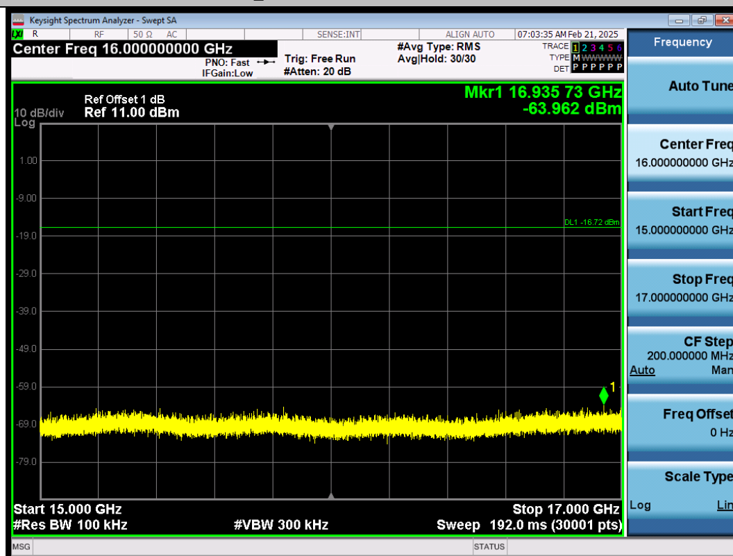
BLE_1M-Ant1-2440-15000~17000-PASS
