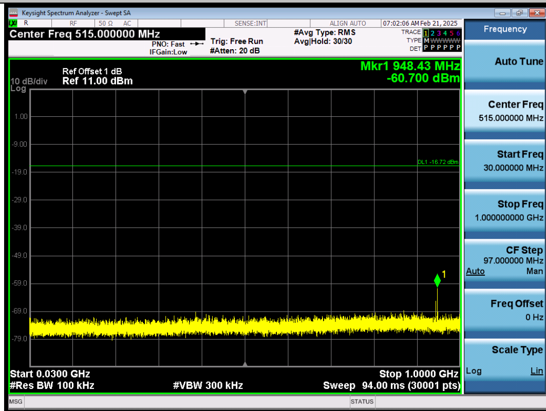
BLE_1M-Ant1-2440-30~1000-PASS
