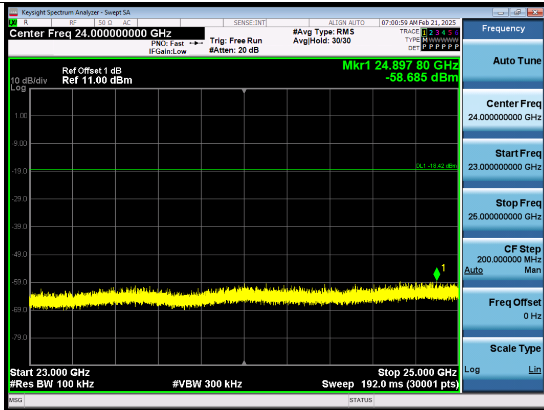
BLE_1M-Ant1-2402-23000~25000-PASS
