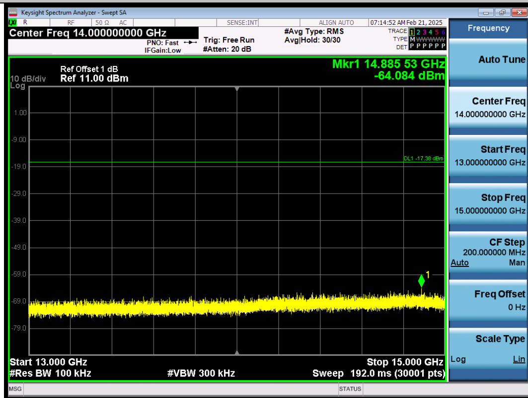
BLE_2M-Ant1-2440-13000~15000-PASS
