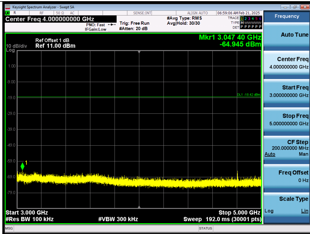
BLE_1M-Ant1-2402-3000~5000-PASS
