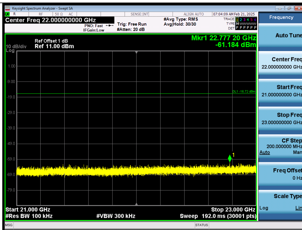
BLE_1M-Ant1-2440-21000~23000-PASS
