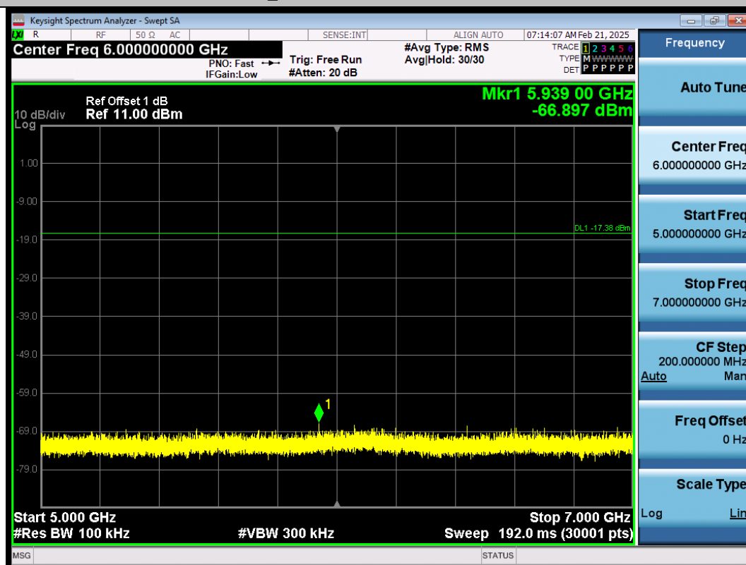
BLE_2M-Ant1-2440-5000~7000-PASS
