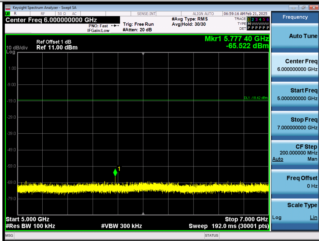
BLE_1M-Ant1-2402-5000~7000-PASS
