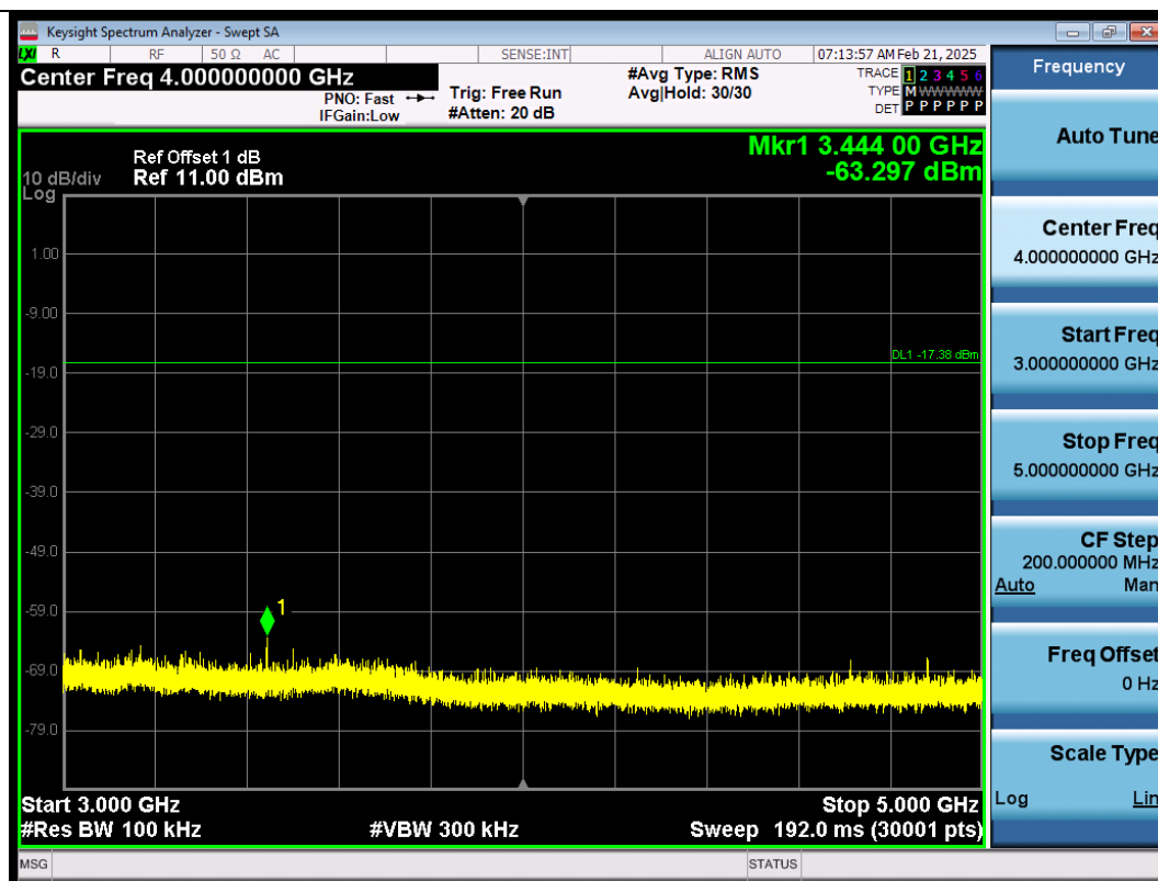
BLE_2M-Ant1-2440-3000~5000-PASS
