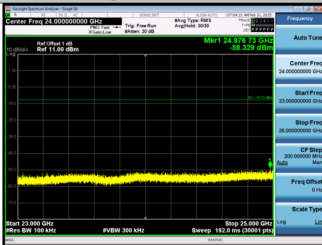
BLE_1M-Ant1-2440-23000~25000-PASS
