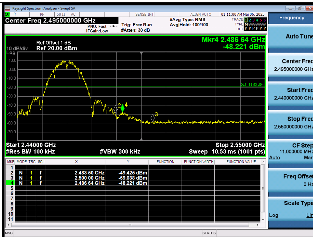
11B-Ant1-2462-PASS
