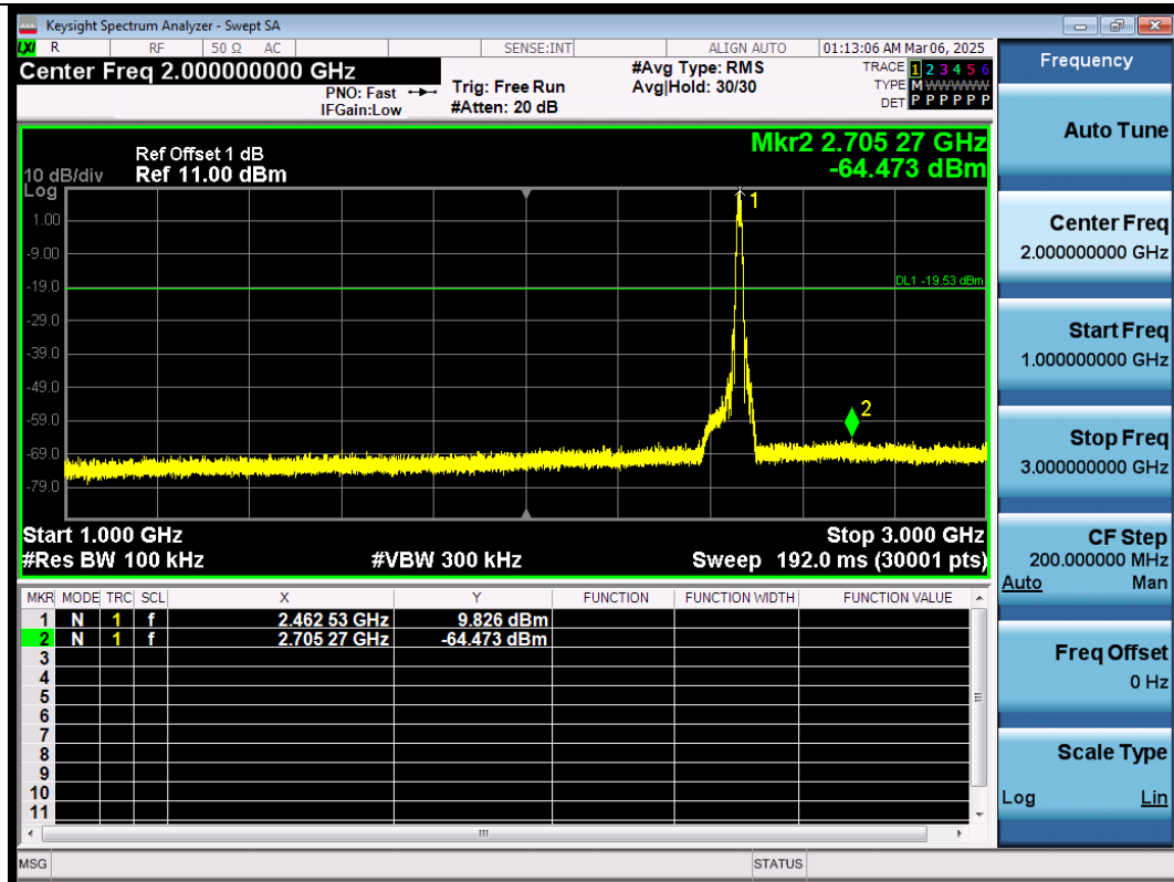
11B-Ant1-2462-1000~3000-PASS
