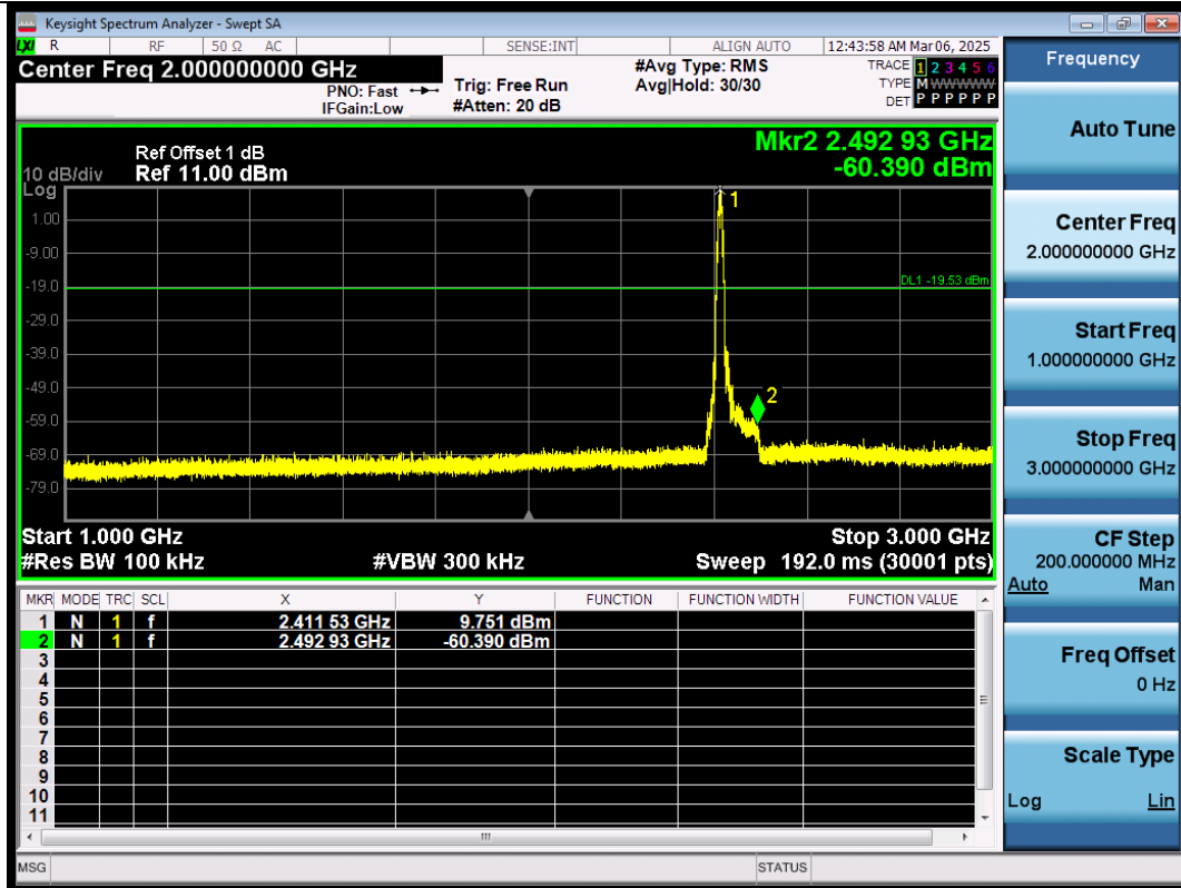
11B-Ant1-2412-1000~3000-PASS
