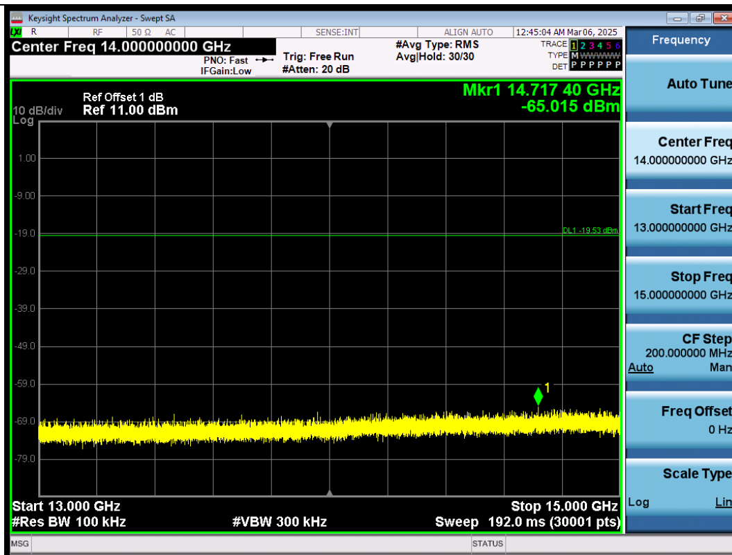
11B-Ant1-2412-13000~15000-PASS
