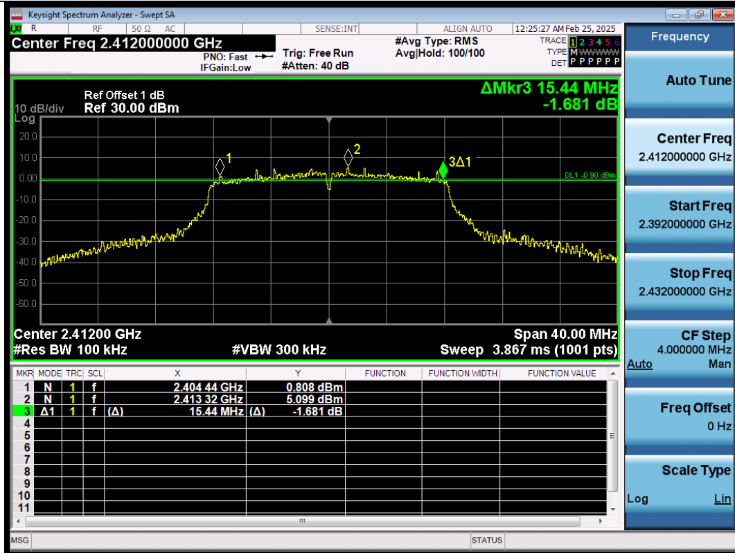
11G-Ant1-2412-PASS
