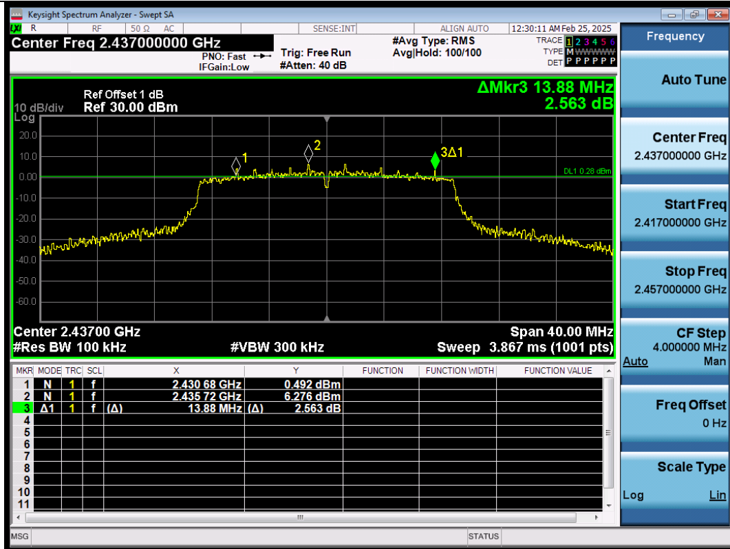
11N20SISO-Ant1-2437-PASS
