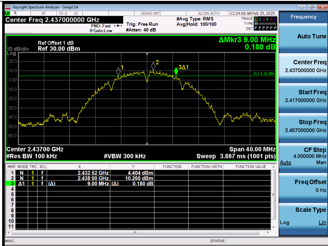
11B-Ant1-2437-PASS
