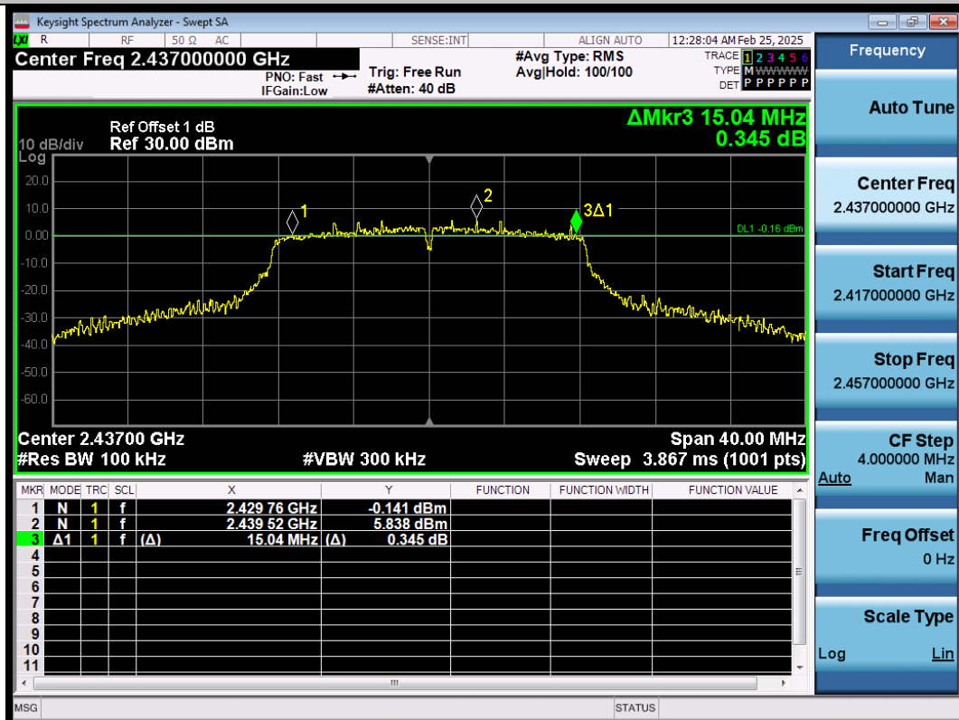
11G-Ant1-2437-PASS
