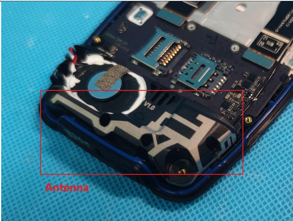
EUT Photo(12) - WWAN Div Antenna
