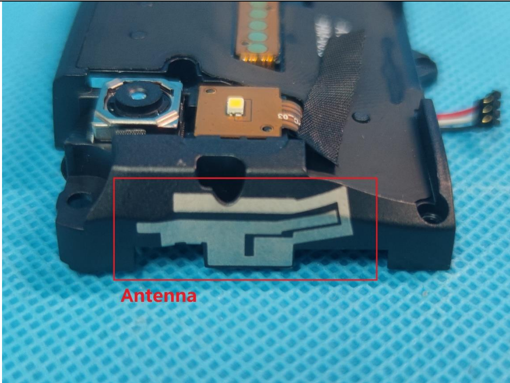
EUT Photo(10) - BT&WIFI&GNSS Antenna
