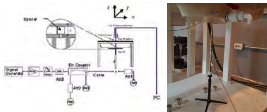
Figure 11.1 Dipole Verification Test Setup Diagram &amp; Photo
