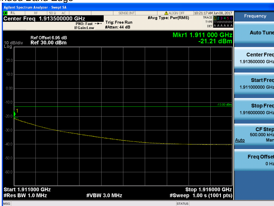
LTE Band 2 / 3MHz / QPSK - RB Size/Offset (8/3)
