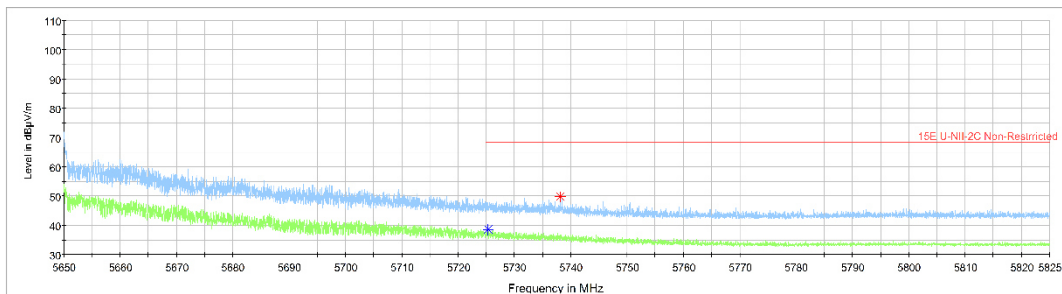
Fig. 24 Band Edges (802.11ac-HT80 , Ch122, 5610MHz)
