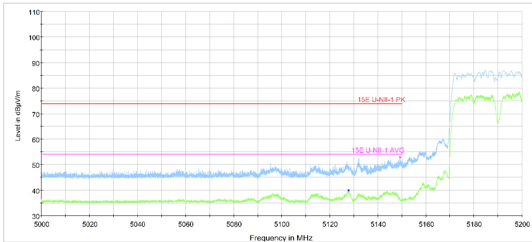
Fig. 37 Band Edges (802.11ax-HT160 , full RU, Ch50, 5250MHz)
