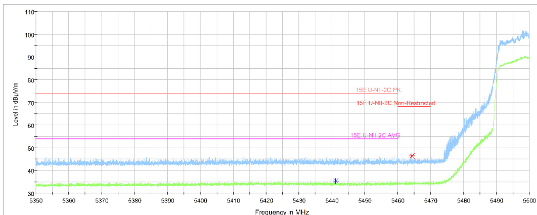
Fig. 27 Band Edges (802.11ax-HT20 , full RU, Ch100, 5500MHz)
