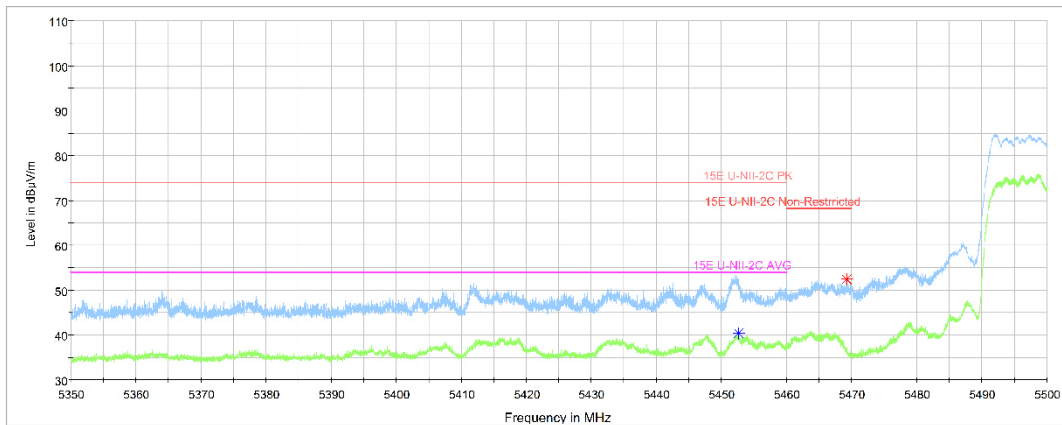
Fig. 38 Band Edges (802.11ax-HT160 , full RU, Ch114, 5570MHz)
