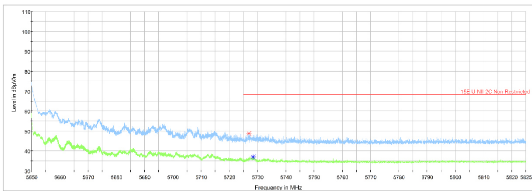
Fig. 36 Band Edges (802.11ax-HT80 , full RU, Ch122, 5610MHz)
