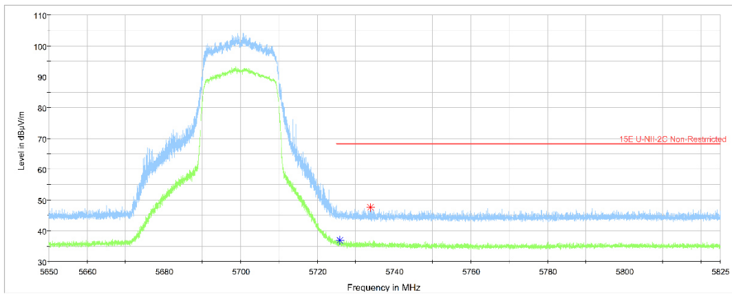
Fig. 28 Band Edges (802.11ax-HT20 , full RU, Ch140, 5700MHz)
