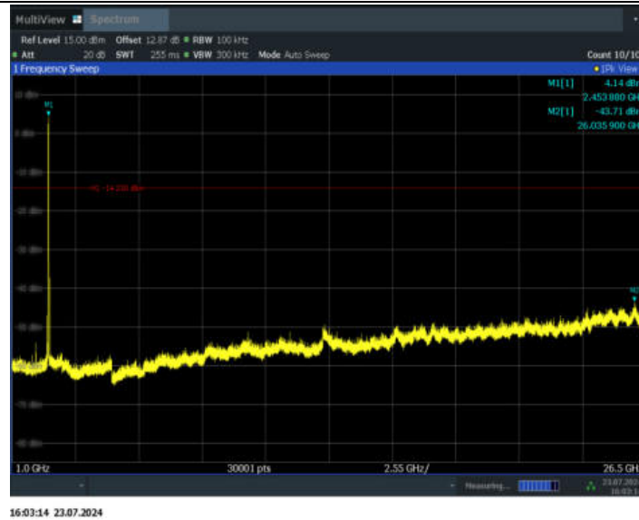
11AX20SISO_Ant2_2462_52Tone_RU40_0~Reference
