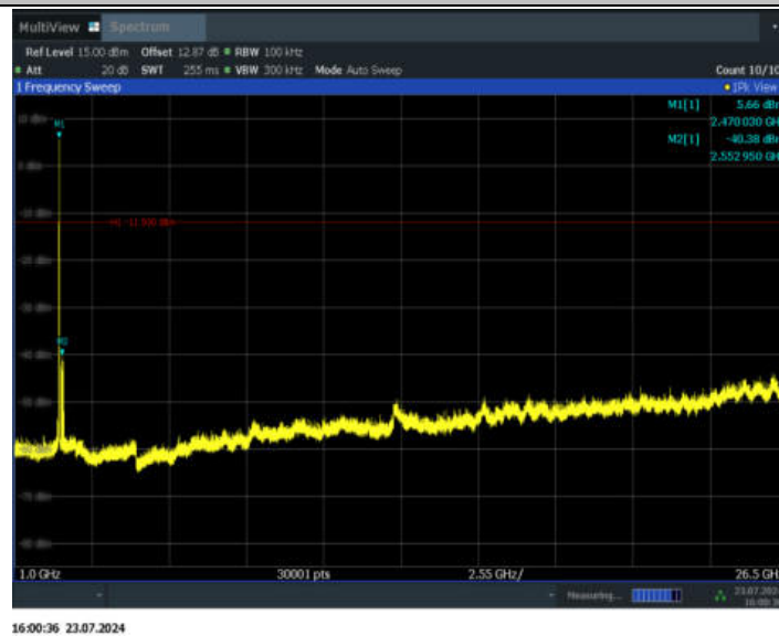
11AX20SISO_Ant2_2462_52Tone_RU37_0~Reference
