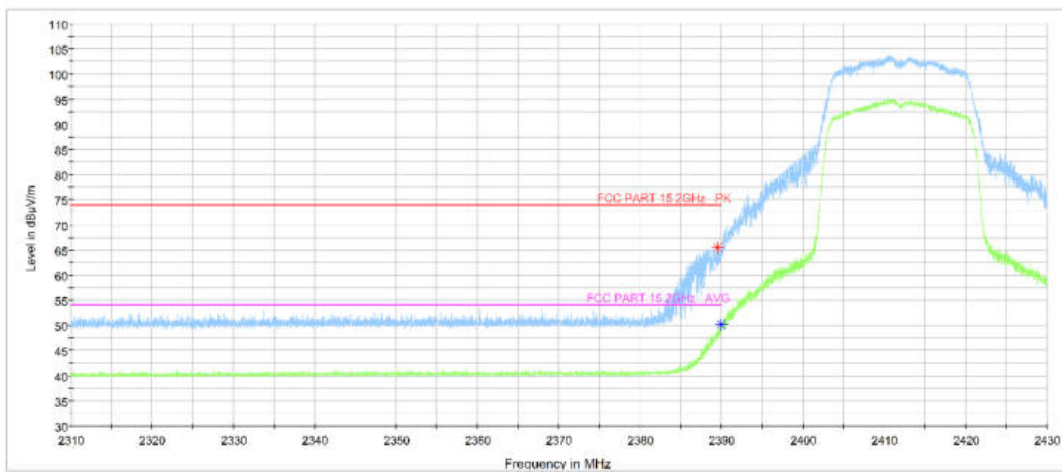
Fig.A.6.2.5 Transmitter Spurious Emission - Radiated (Power): 802.11n-HT20, ch1, 2.31 GHz - 2.43GHz
