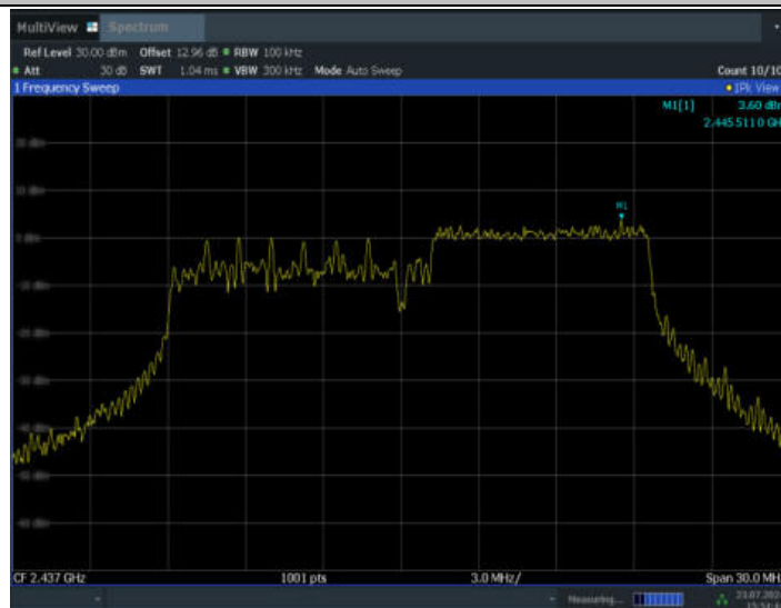
11AX20SISO_Ant2_2437_106Tone_RU54_0~Reference
