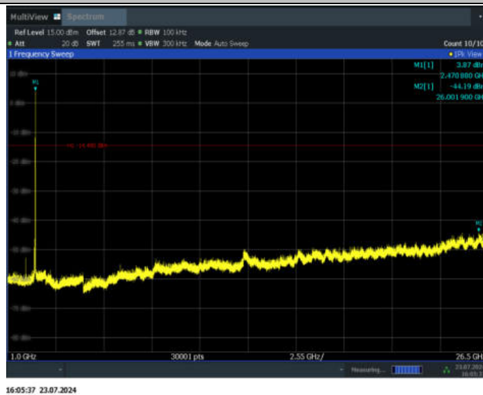
11AX20SISO_Ant2_2462_106Tone_RU53_0~Reference
