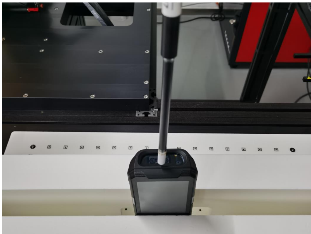
Picture 15: Top Side
