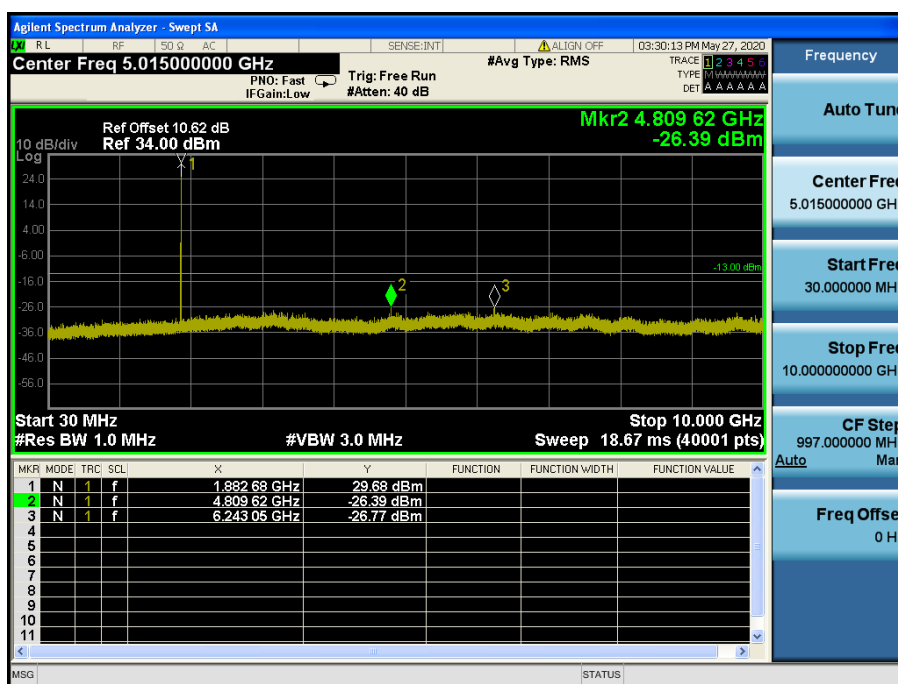
LTE Band 2, 25 / 1.4 MHz / 16QAM - RB Size/Offset (1/2) – Mid Channel
