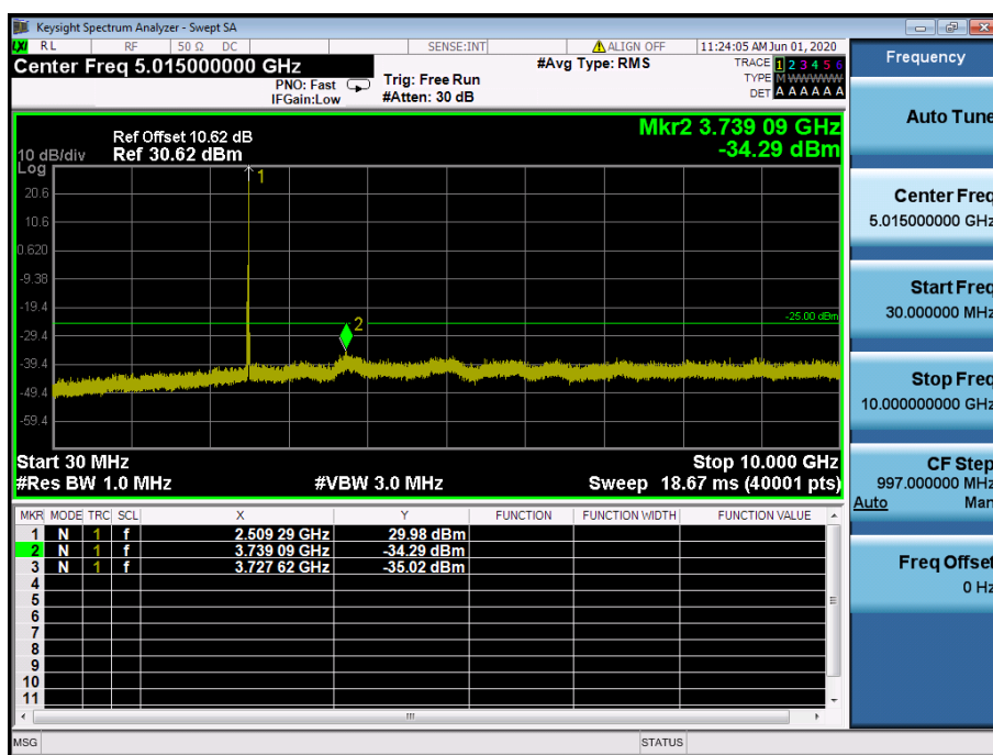
LTE Band 7 / 10 MHz / QPSK - RB Size/Offset (1/49) – Low Channel
