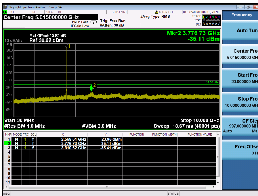
LTE Band 7 / 5 MHz / 16QAM - RB Size/Offset (25/0) – High Channel
