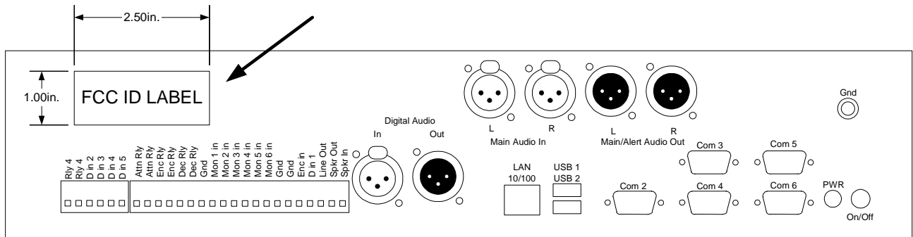
Rear Panel
