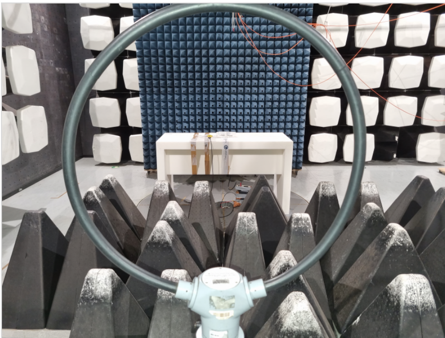
Photograph 2: EUT test setup in the semi anechoic chamber, overview_EUT elevation 0°, EUT in TX mode
