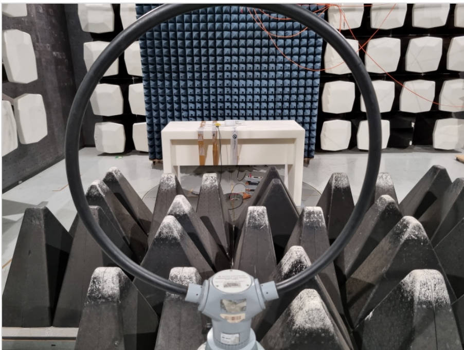
Photograph 4: EUT test setup in the semi anechoic chamber, overview_EUT elevation 0°, EUT in TXRX mode
