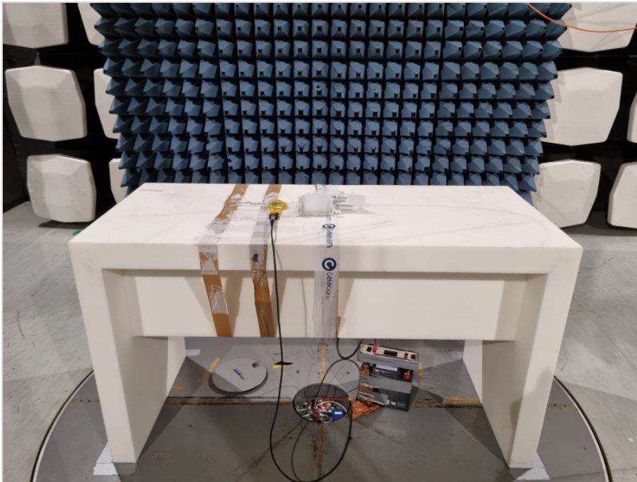
Photograph 5: EUT test setup in the semi anechoic chamber, close up view_EUT elevation 0°, EUT in TXRX mode
