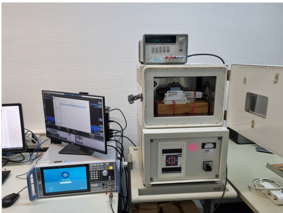
Photograph 8: EUT setup in the climatic chamber for test under extreme conditions, overview, EUT in TXRX mode
