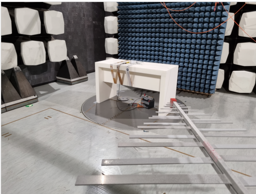
Photograph 6: EUT test setup in the semi anechoic chamber, overview_EUT elevation 0°, EUT in TXRX mode
