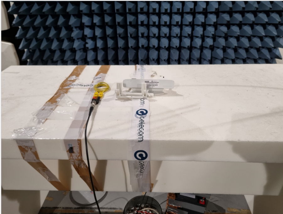
Photograph 1: EUT test setup in the semi anechoic chamber, close up view_EUT elevation 0°, EUT in TX mode
