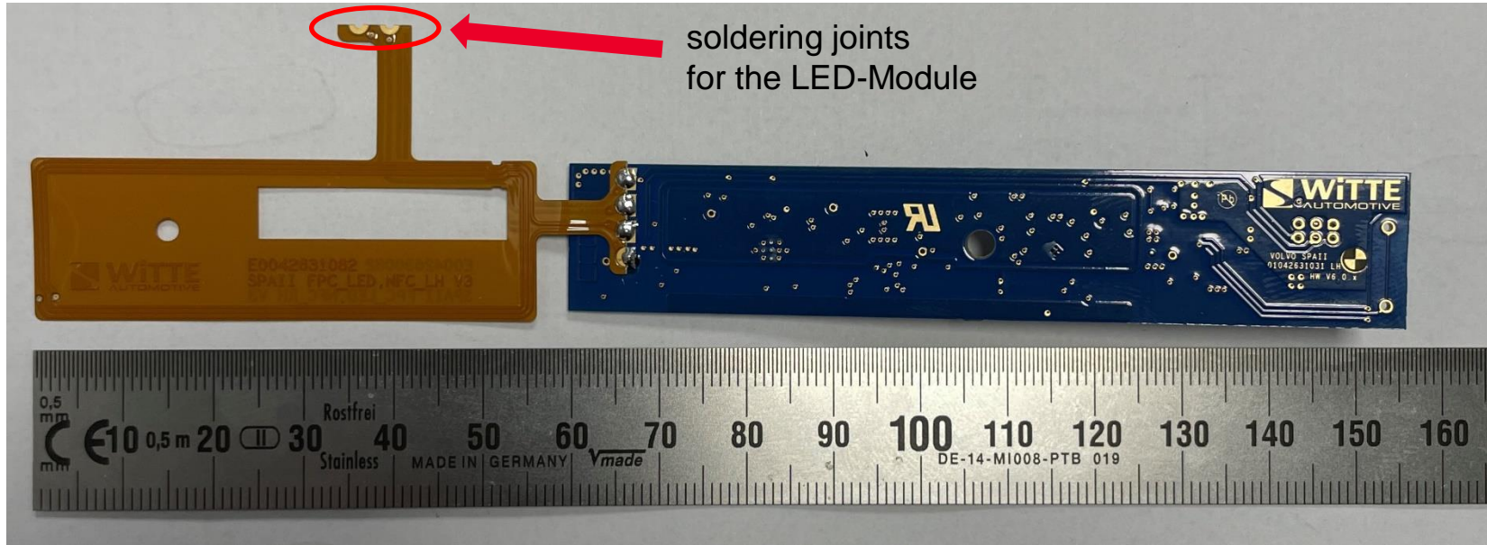
PCBA with NFC-Antenna and without LED-Module
