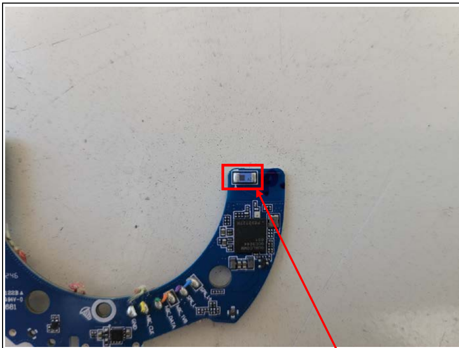
Bluetooth & Bluetooth Low Energy Antenna
