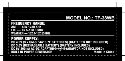
TF-38 RATING LABEL LABEL SIZE: 50.0L X 20.0W (mm) PRINT BLACK WHITE COLOR ON BLACK BACKGROUND LABEL + COATING
