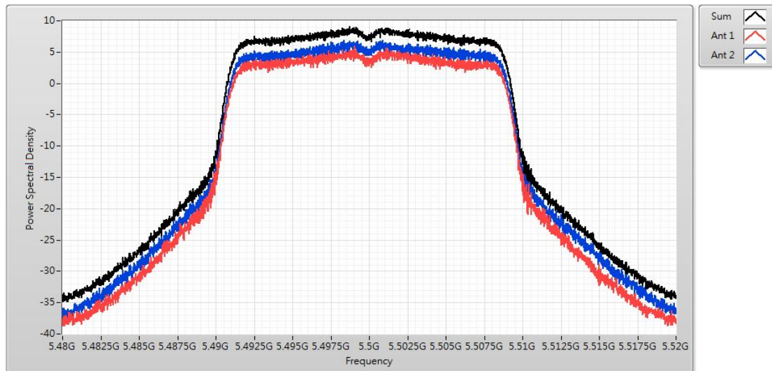
Channel 100
