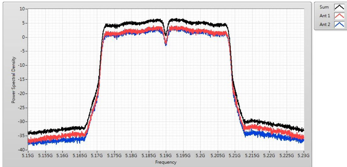
Channel 38
