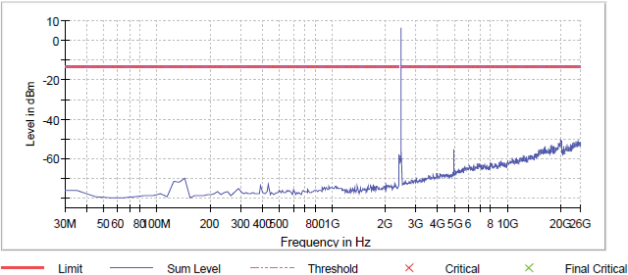
Spurious
