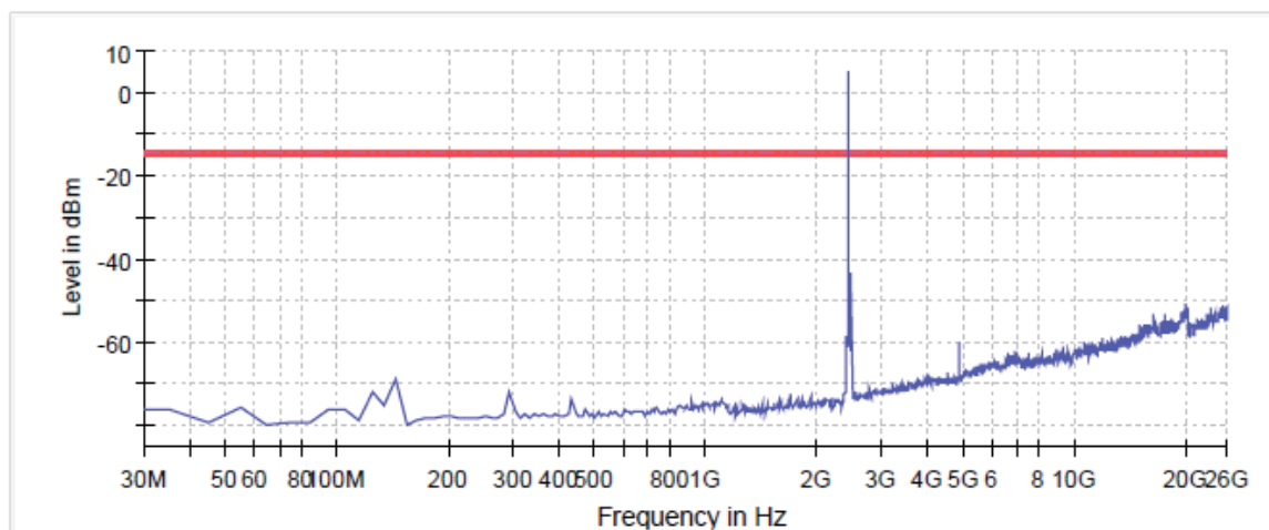
Spurious
