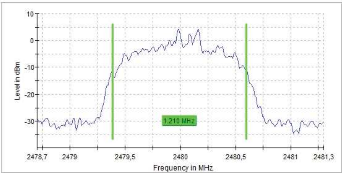
99% Bandwidth
