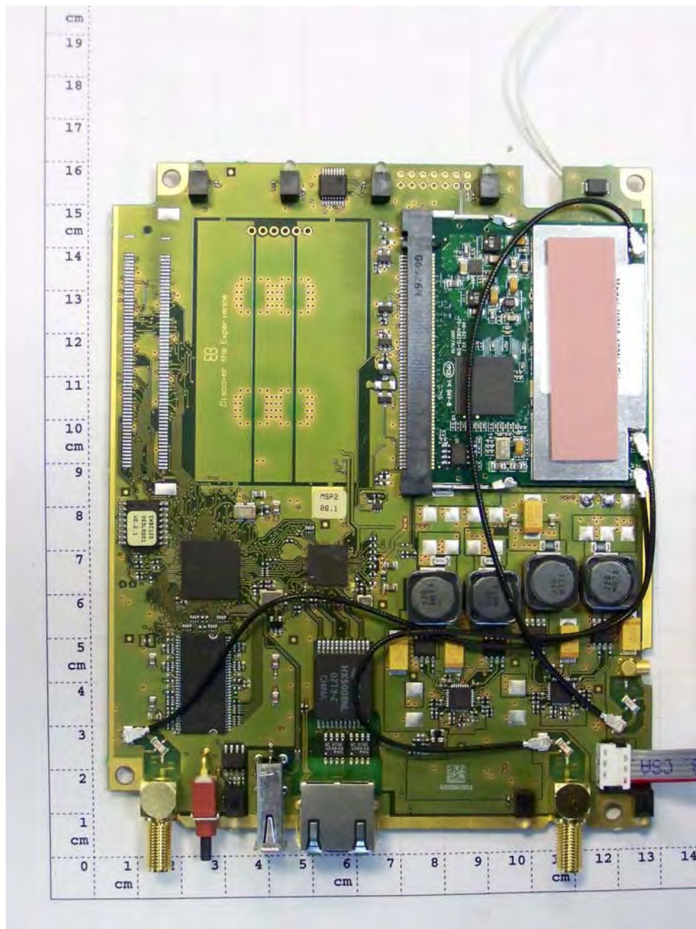
Photograph 8: view on top side of main PCB with radio PCB
