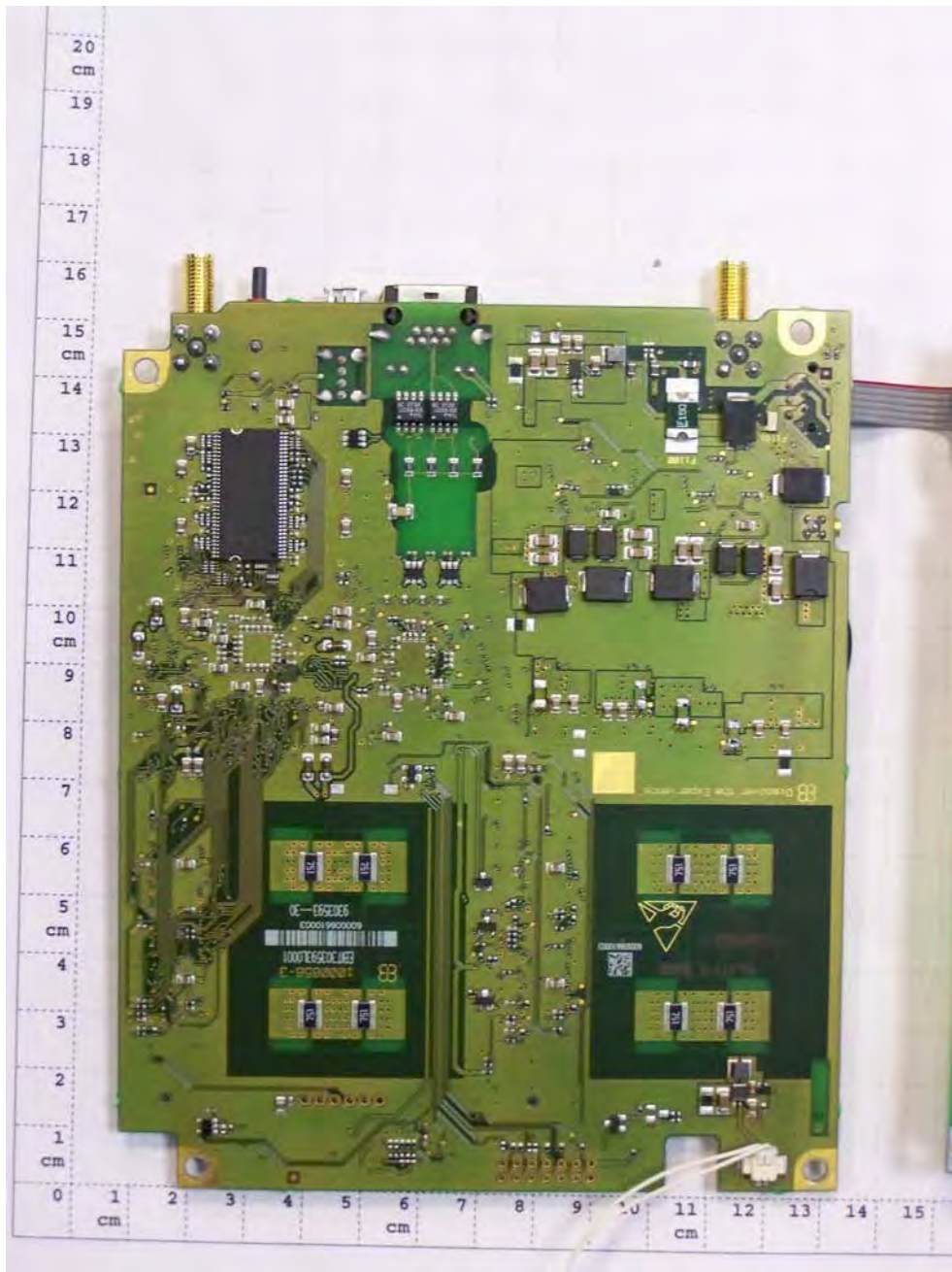
Photograph 9: view on bottom side of main PCB
