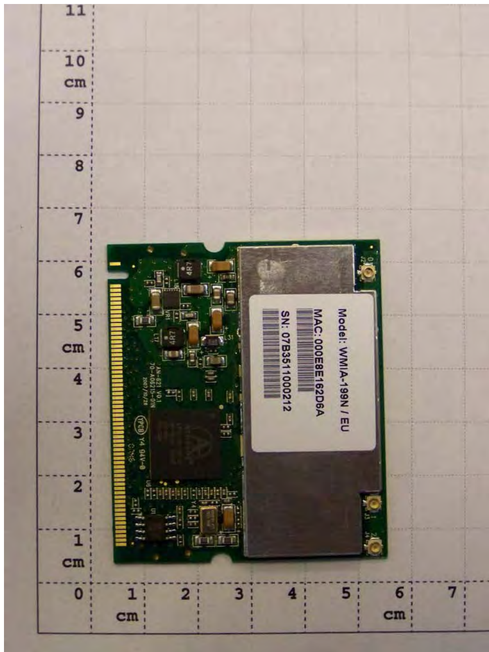
Photograph 10: view on top side of Radio PCB
