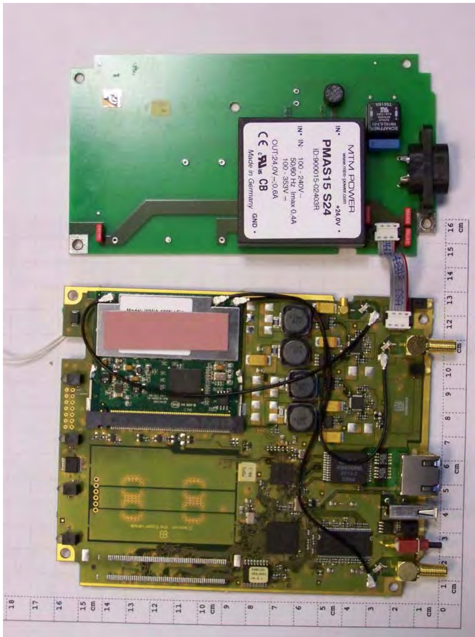
Photograph 7: view on top side of main and power supply PCB
