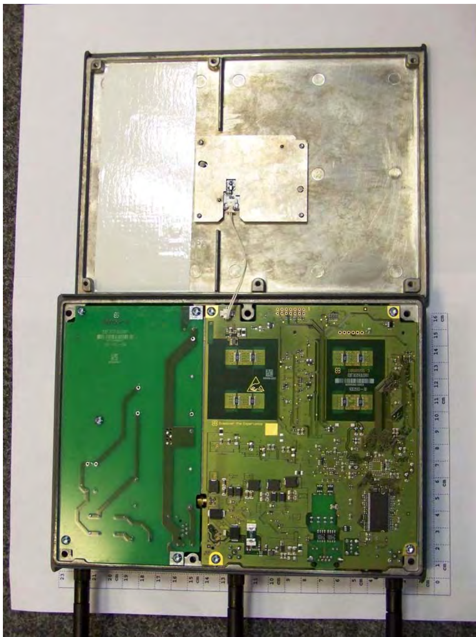
Photograph 3: Overall top view with opened housing
