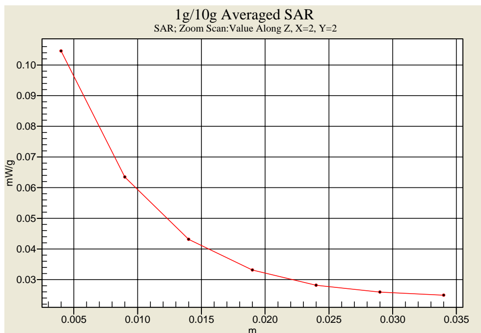
Figure 12. Z-axis Plot of flat 802.11b CH1_6M
