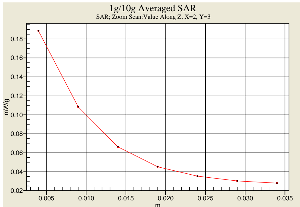
Figure 11. Z-axis Plot of flat 802.11b CH1_11M
