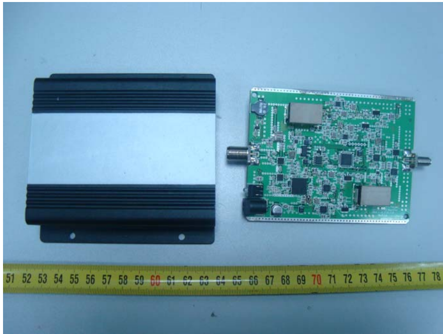
EUT – Main Board Shield Top view
