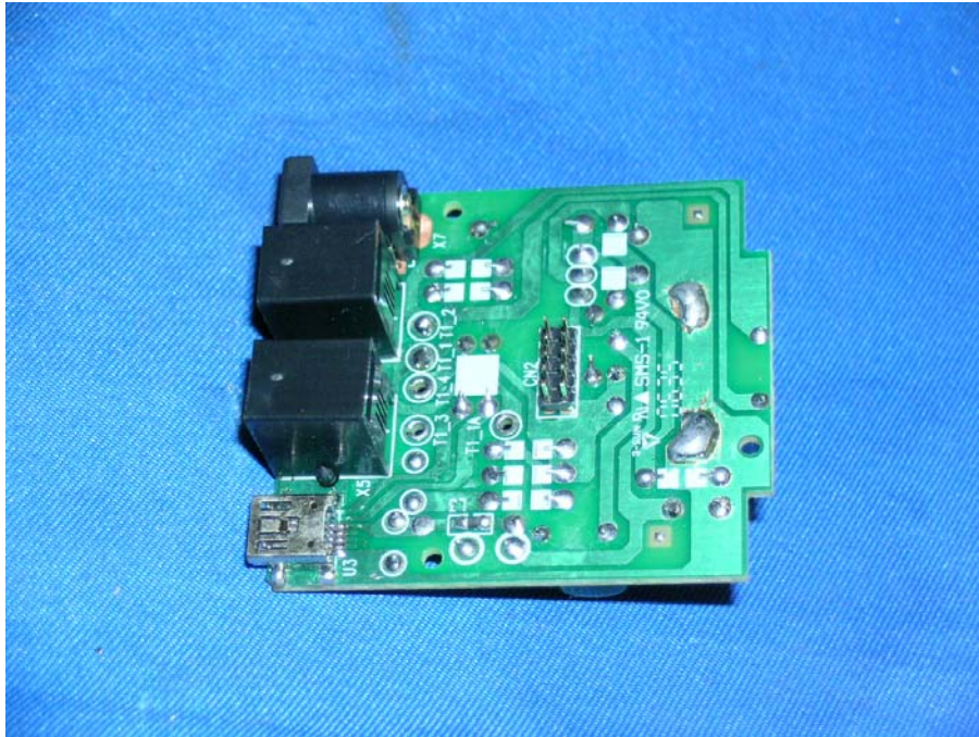
Docking station Main PCB solder side
