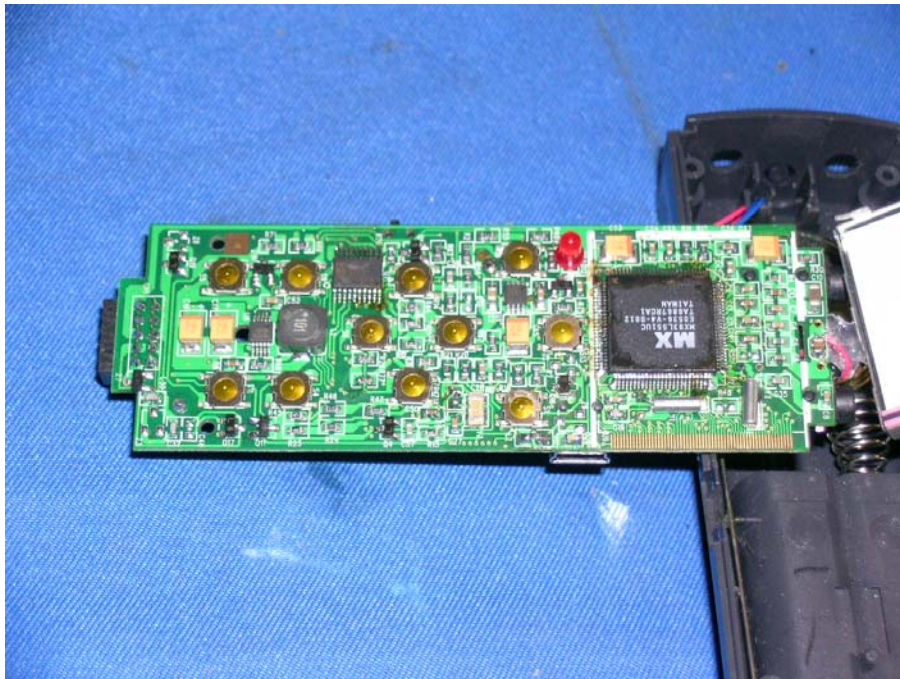
Recorder display front side (View 2)
