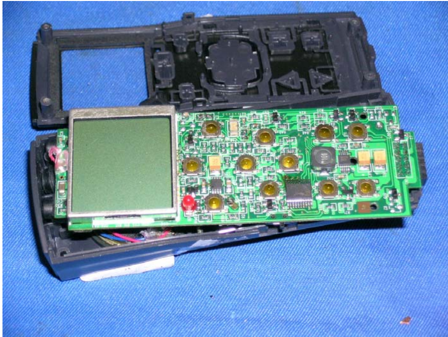
Recorder display front side (View 1)
