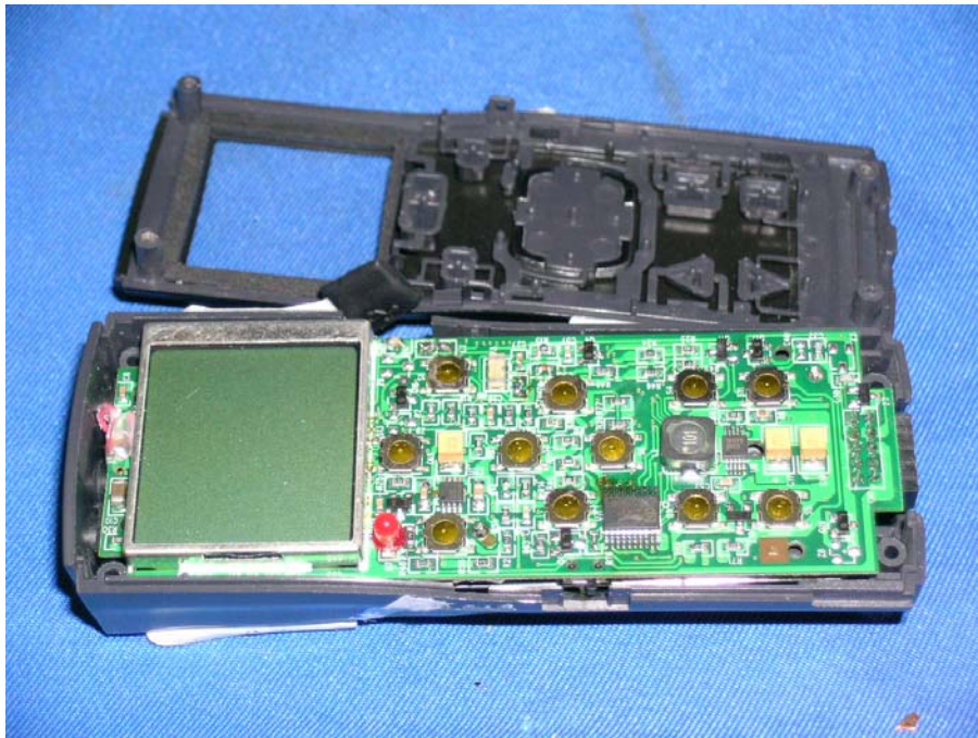
Recorder assembly
