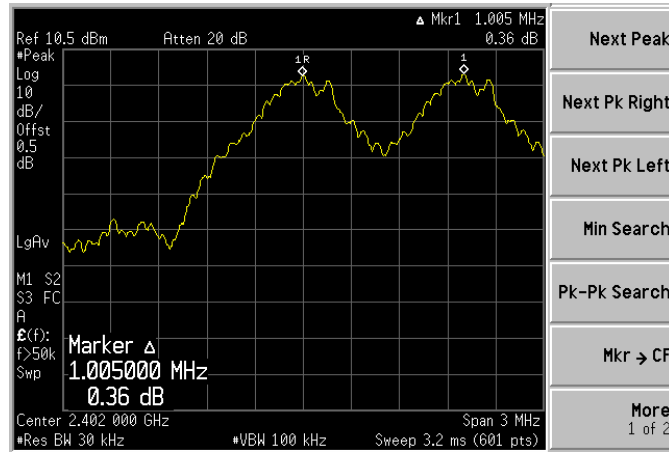
Figure 2. Plot of the Carrier Frequency Separation (Conducted)
