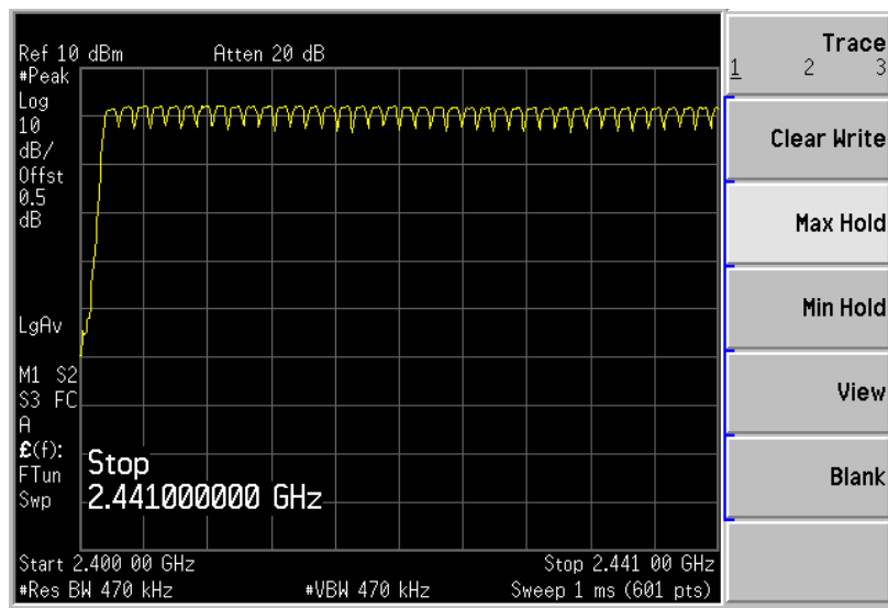
Figure 4. Plot of the Number of Hopping Channels (Conducted)
