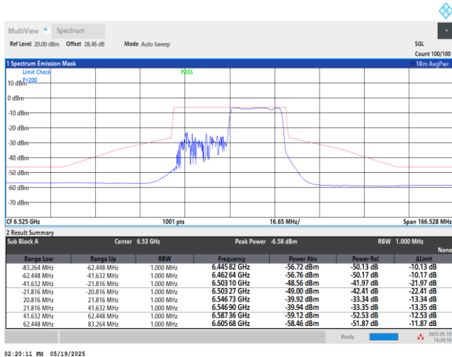
Plot on 6525 MHz
