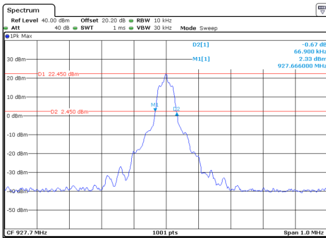
20 dB Bandwidth Plot on 927.7 MHz
