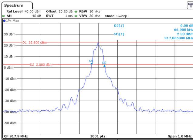
20 dB Bandwidth Plot on 917.9 MHz
